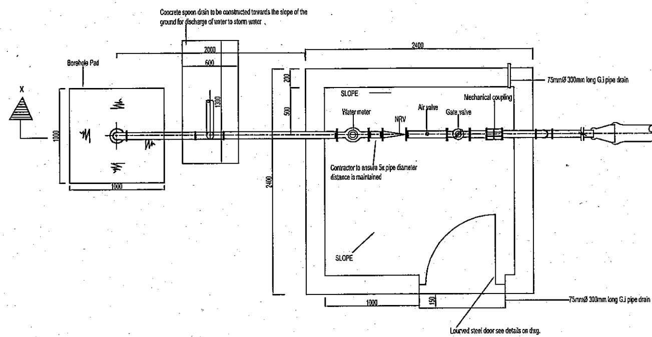
BOREHOLE STARTER ROOM PLAN Scale 1:40
