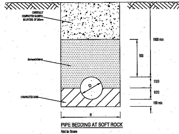
PIPE BEDDING for DIA. 100 to 300 mm
