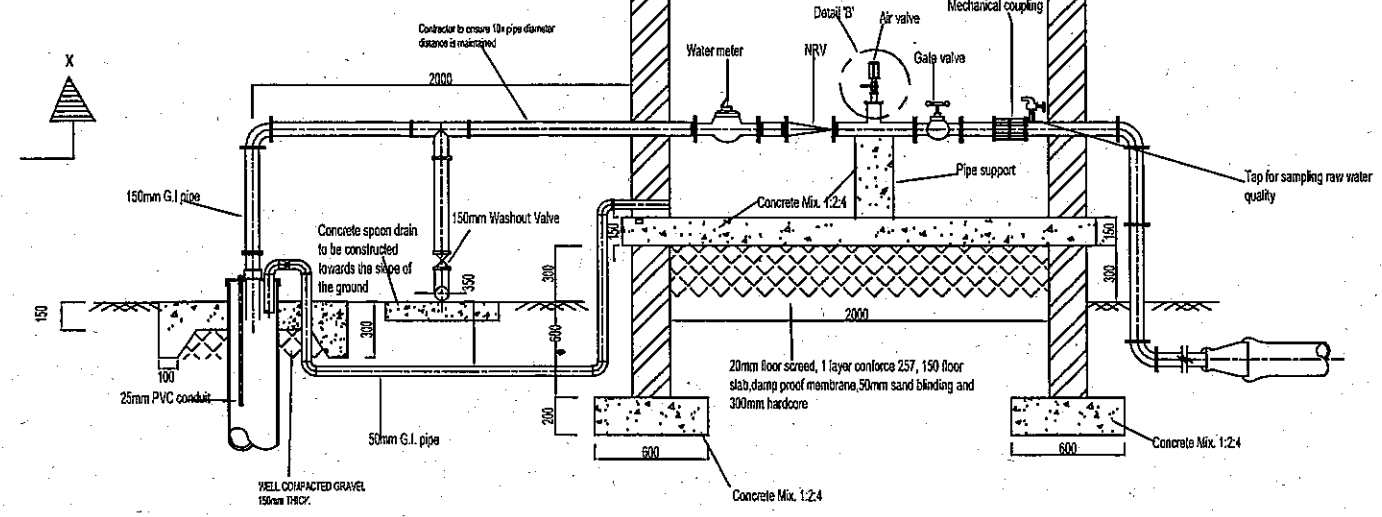
SECTION X-X Scale 1:40
