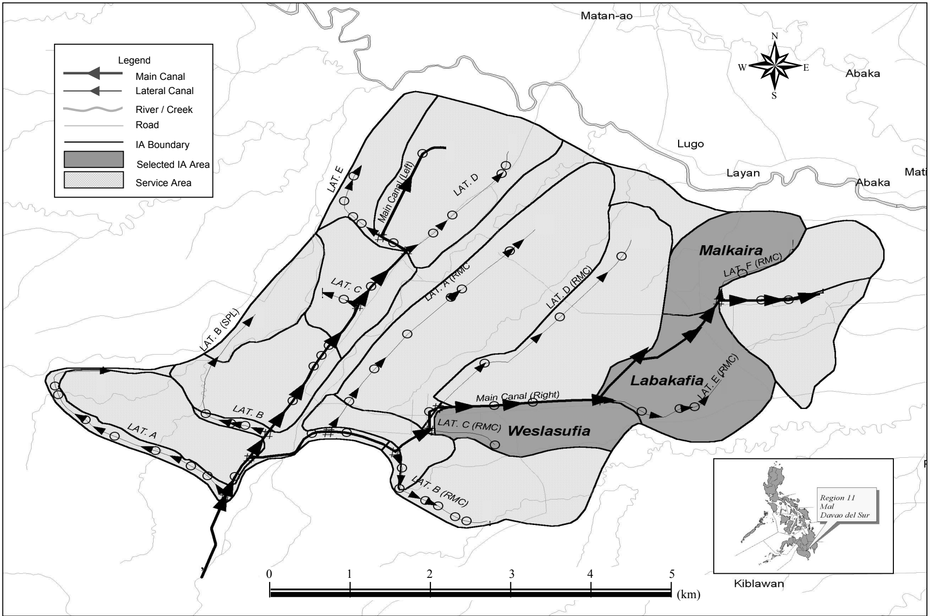
Figure 7.1 General Layout and Location of the Pilot IAs in Mal
