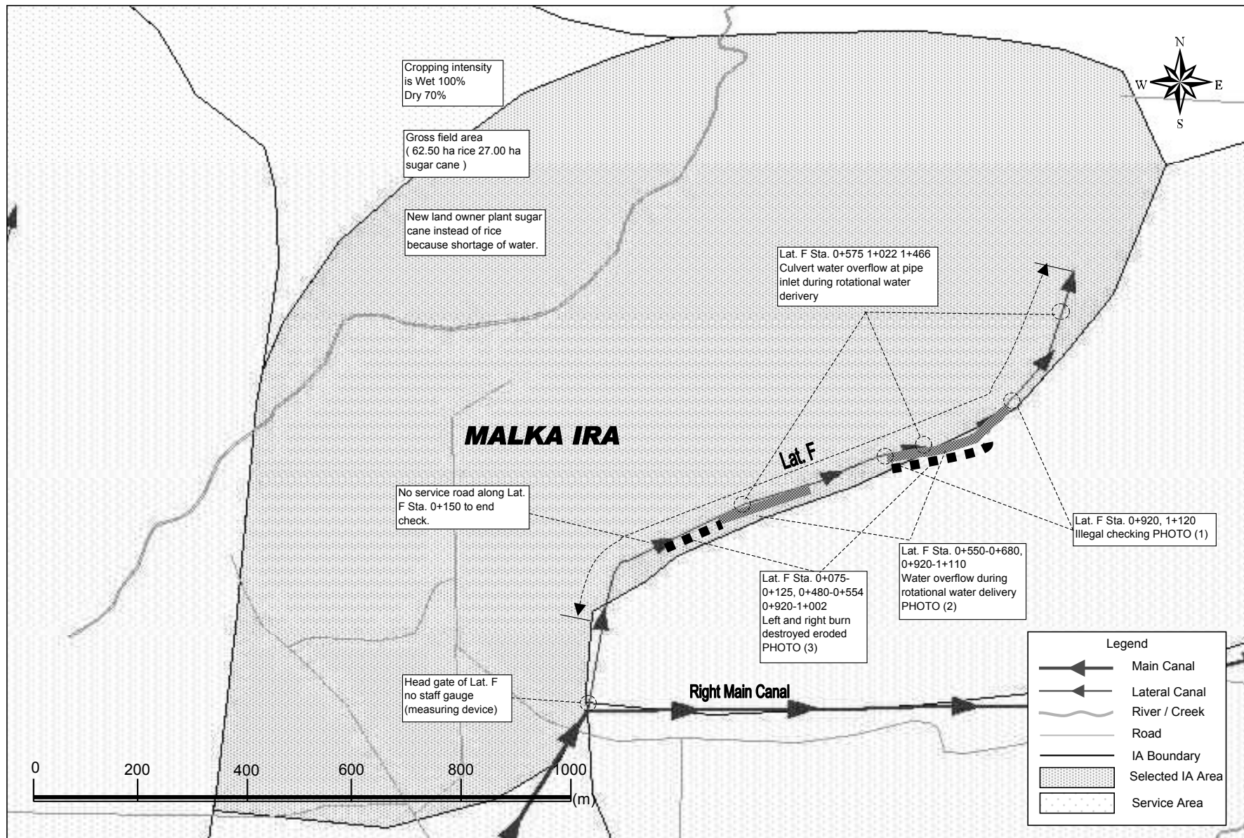
Figure 7.4 Findings on Walk Through Mal RIS - Labakafia IA
