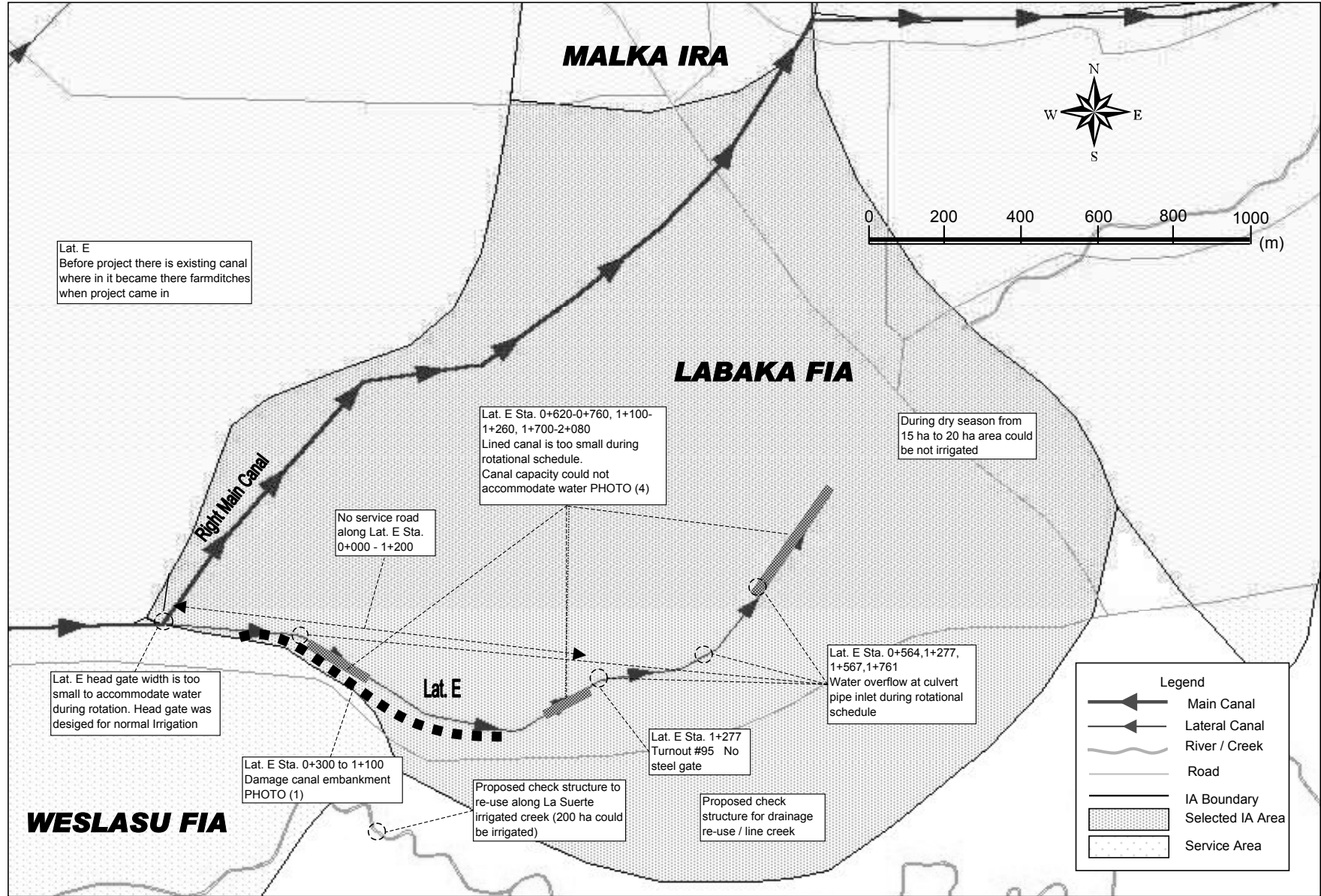
Figure 7.3 Findings on Walk Through Mal RIS - Labakafā IA
