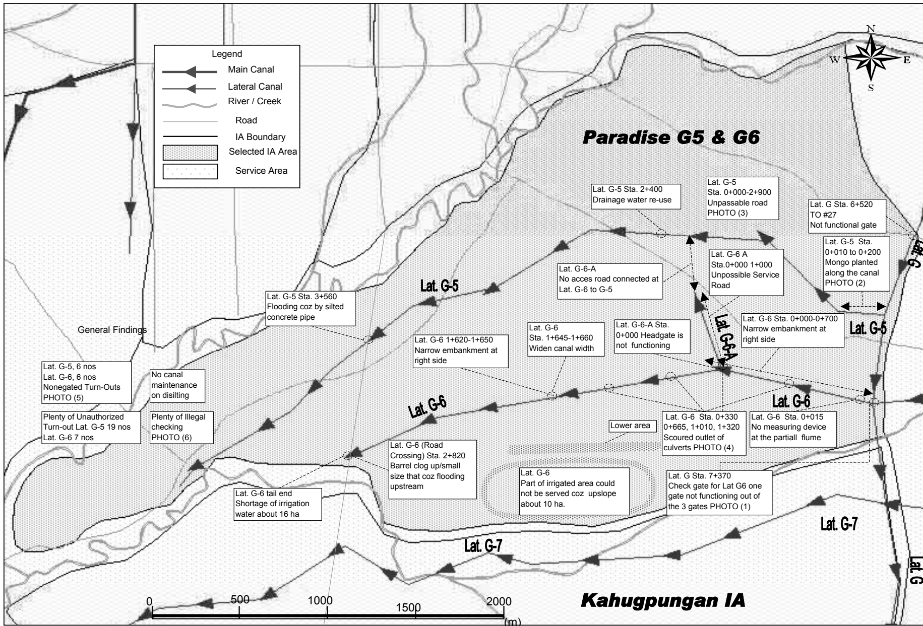
Figure 6.2 Findings on Walk Through Palangui RIS - Paradise G5 & G6 IA
