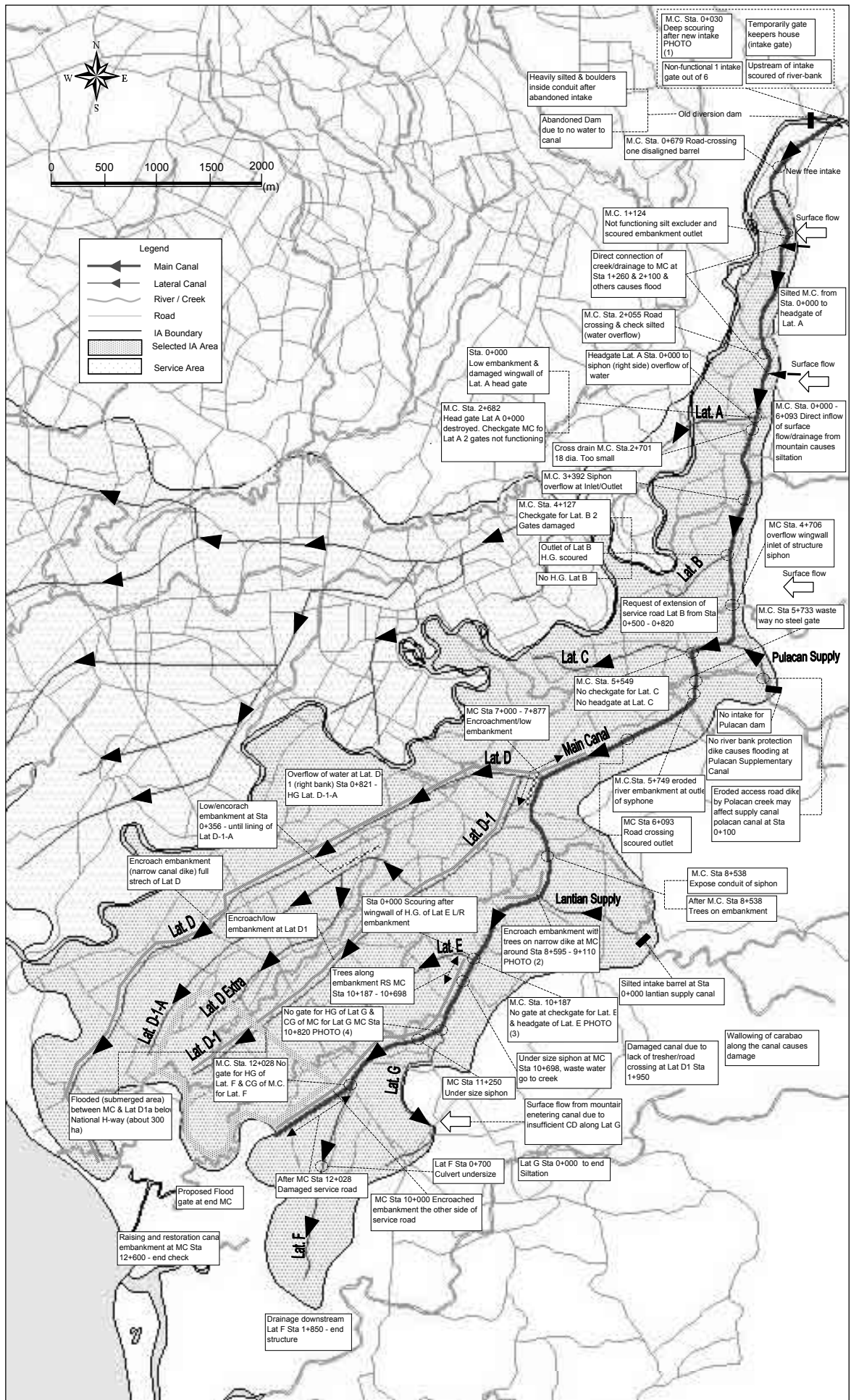
Figure 5.2 Findings on Walk Through Labangan RIS - Muchrist IA
