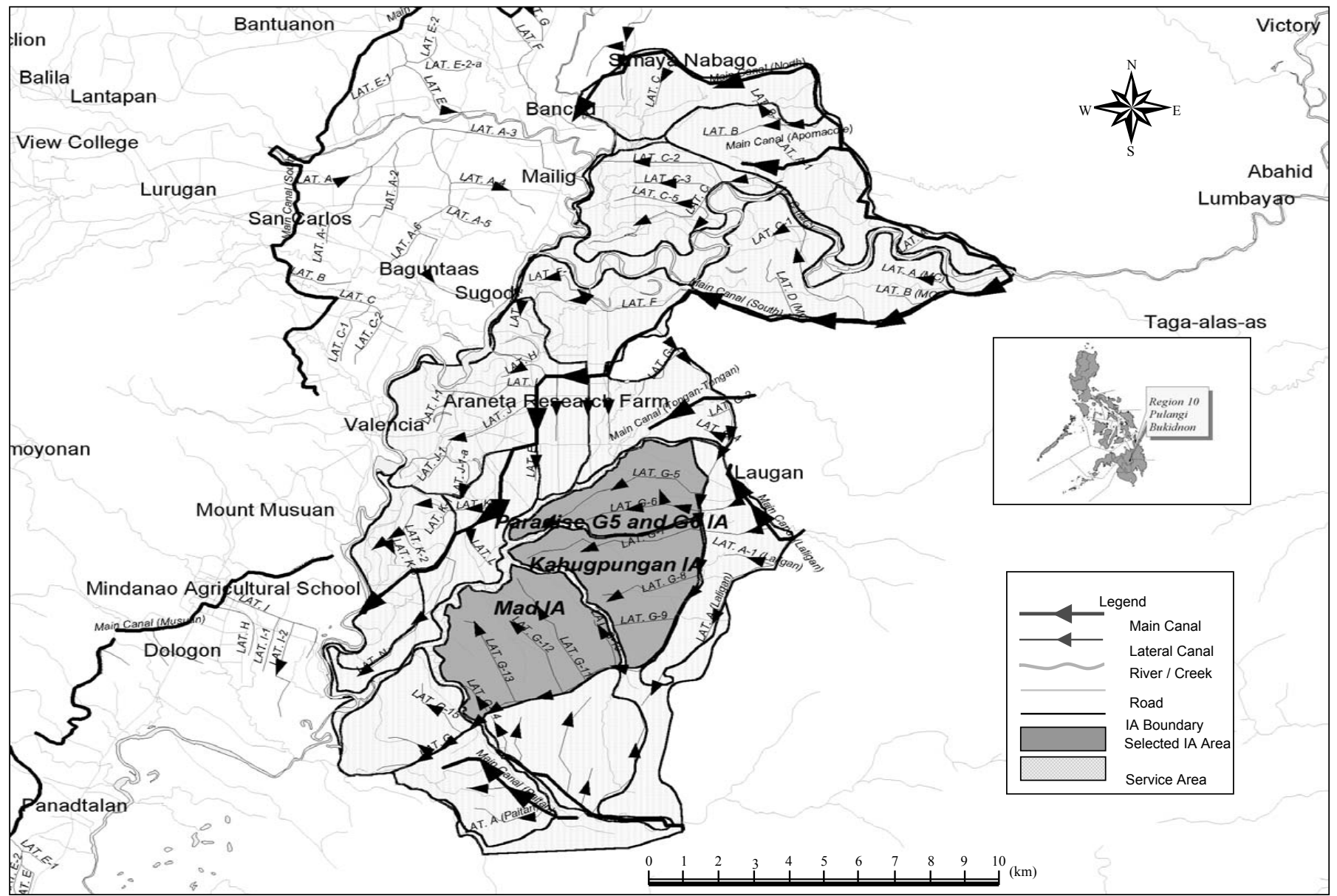
Figure 6.1 General Layout and Location of the Pilot IAs in Pulangui RIS A10-68
