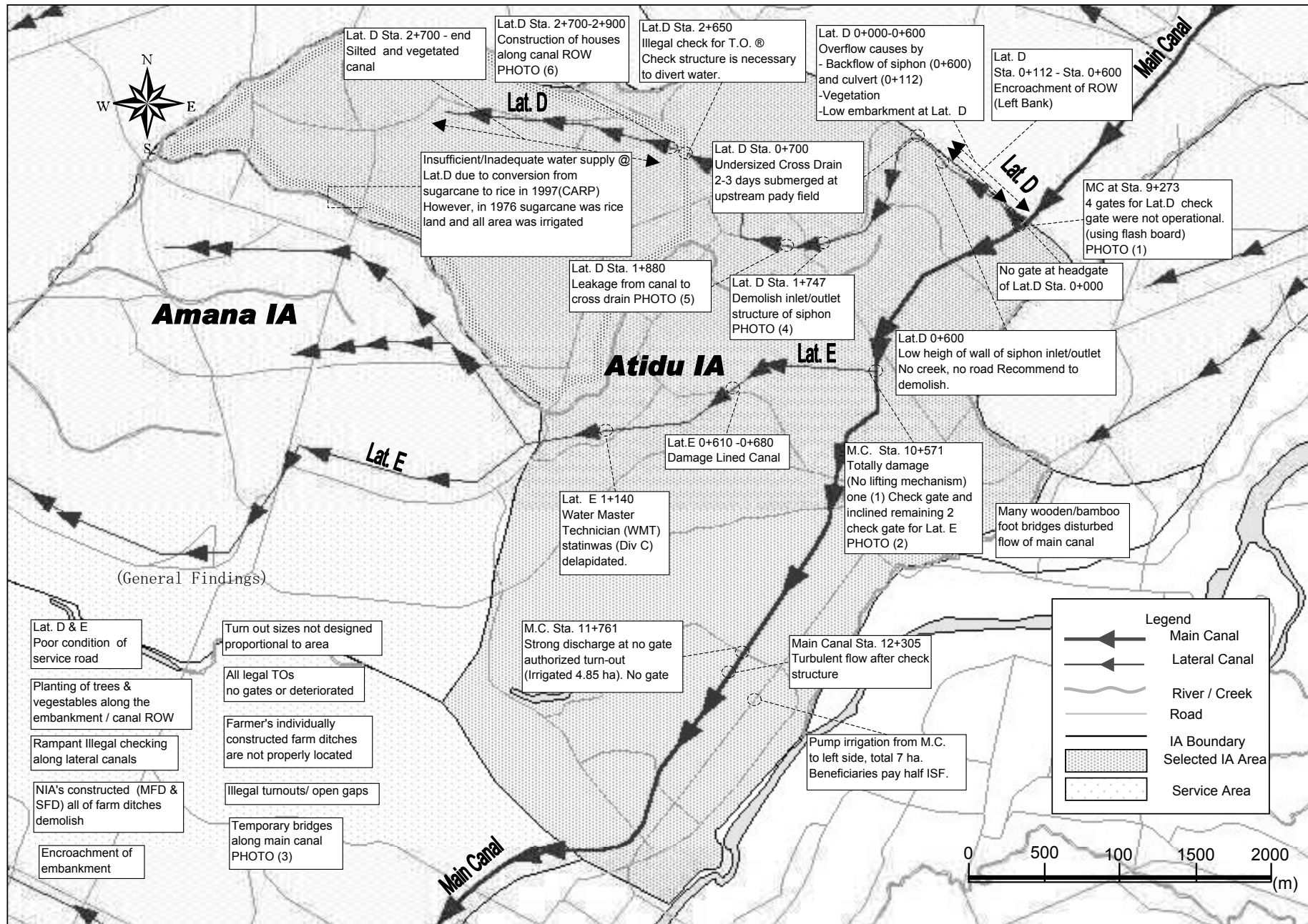
Figure 4.2 Findings on Walk Through Bago RIS - Atidu IA
