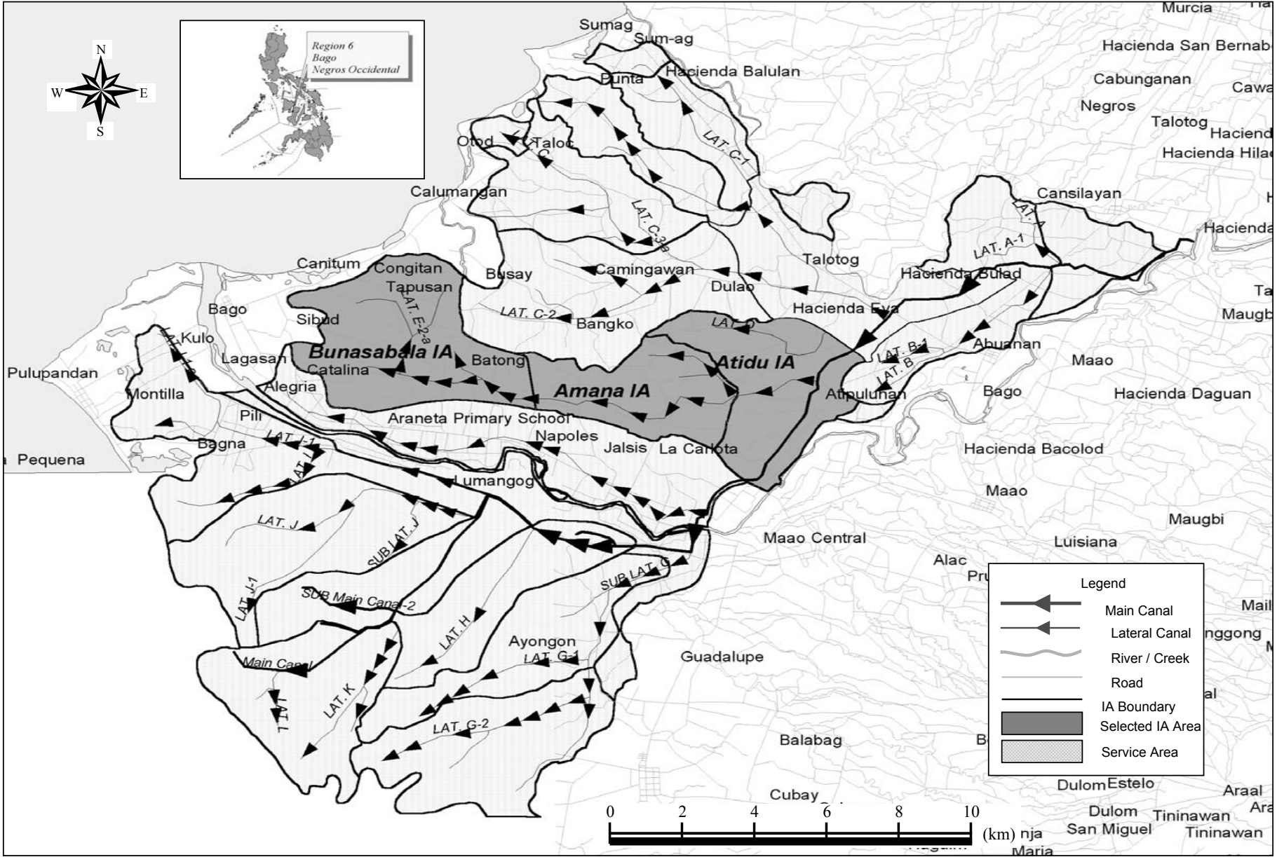
Figure 4.1 General Layout and Location of the Pilot IAs in Bago RIS A10-61
