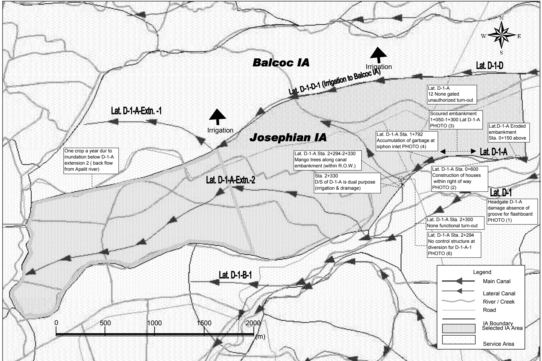
Figure 3.4 Findings on Walk Through Angat RIS - Josephian IA
