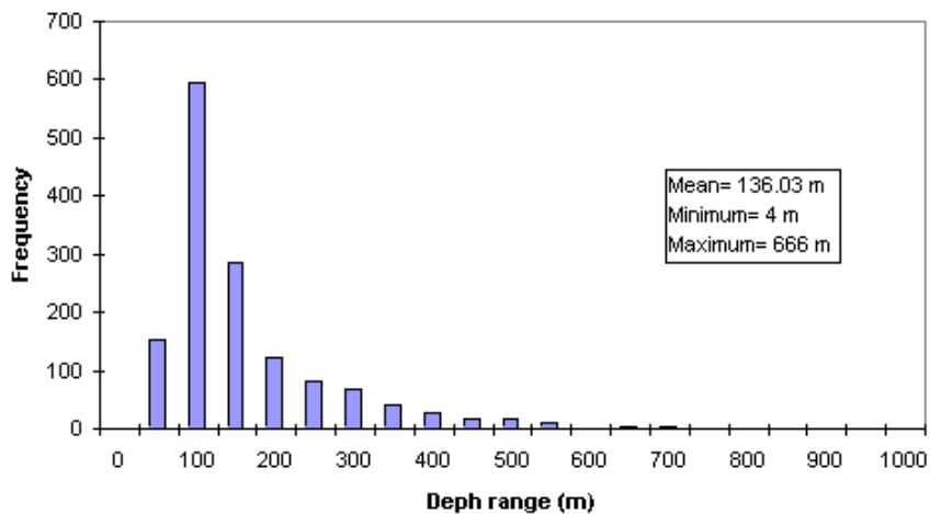
Figure 2.2 Histogram of well depth presented by the captured information in the database
