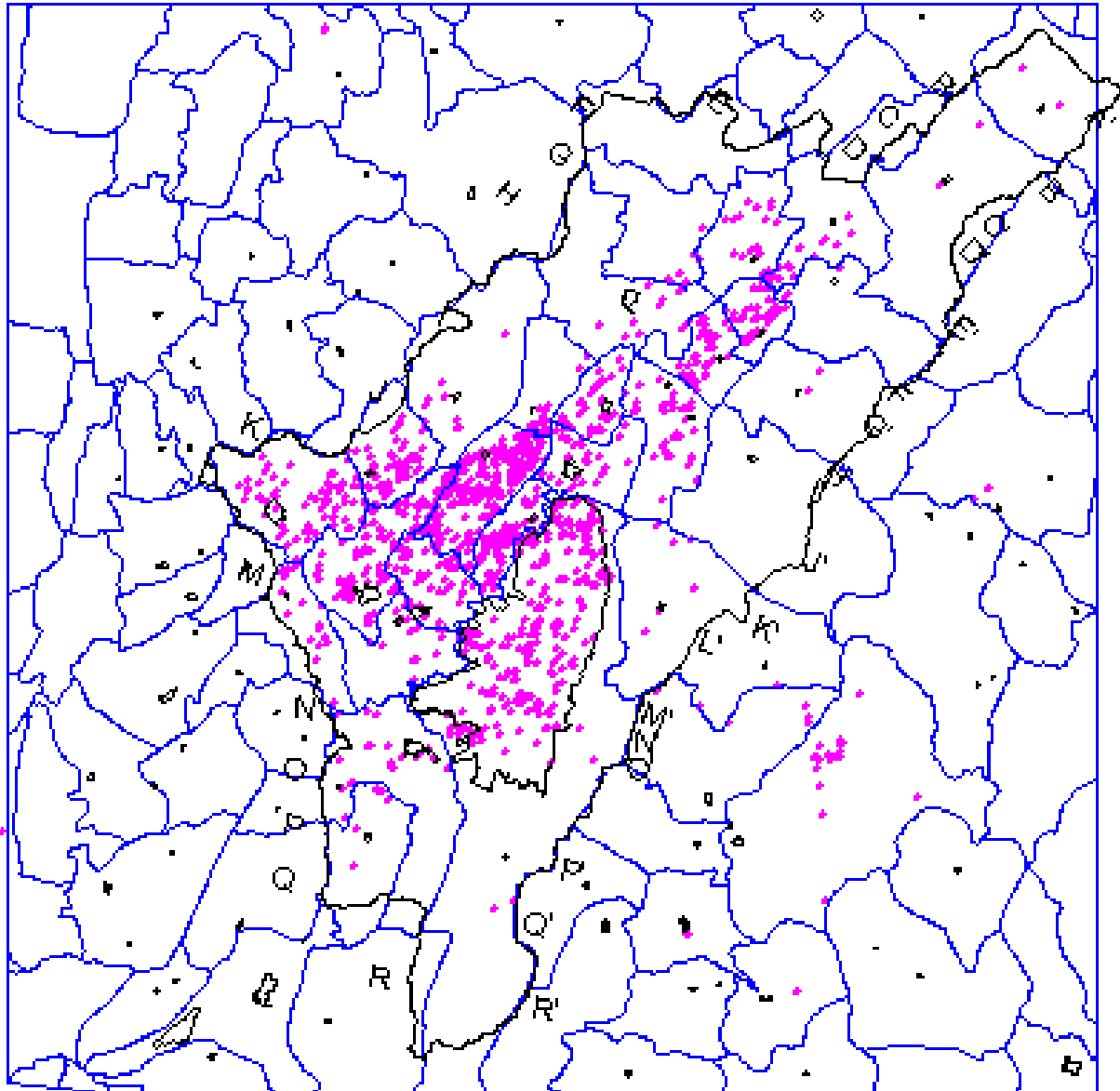
Figure 2.1 Spatial distribution of well inventoried by JICA using CAR and DAMA files.
