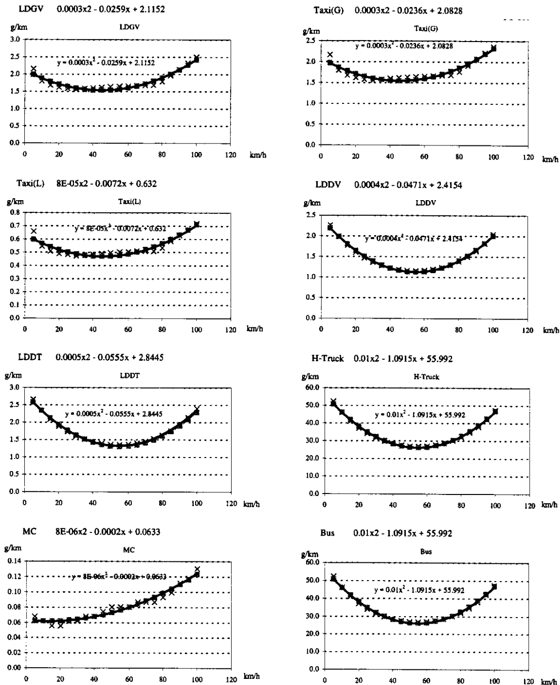
Figure 4.1.2.3 NO x Emission Factor of the vehicles at 2000
