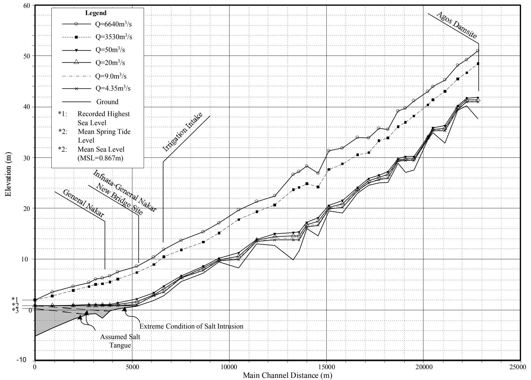
Figure I4.1 Profile of River Water Levels in Agos Lower Reach
