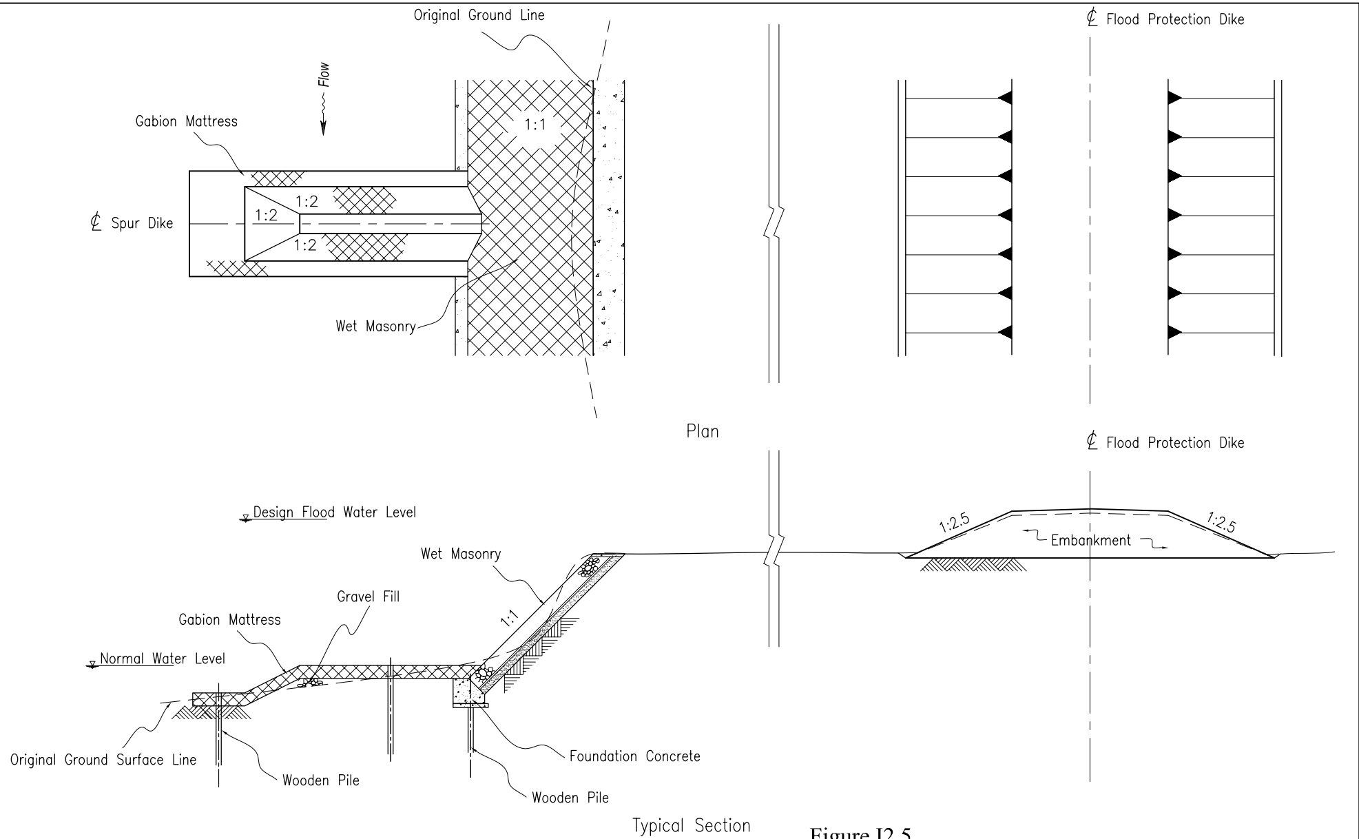
Figure I2.5 River Bank Protection Work and Flood Protection Dike
