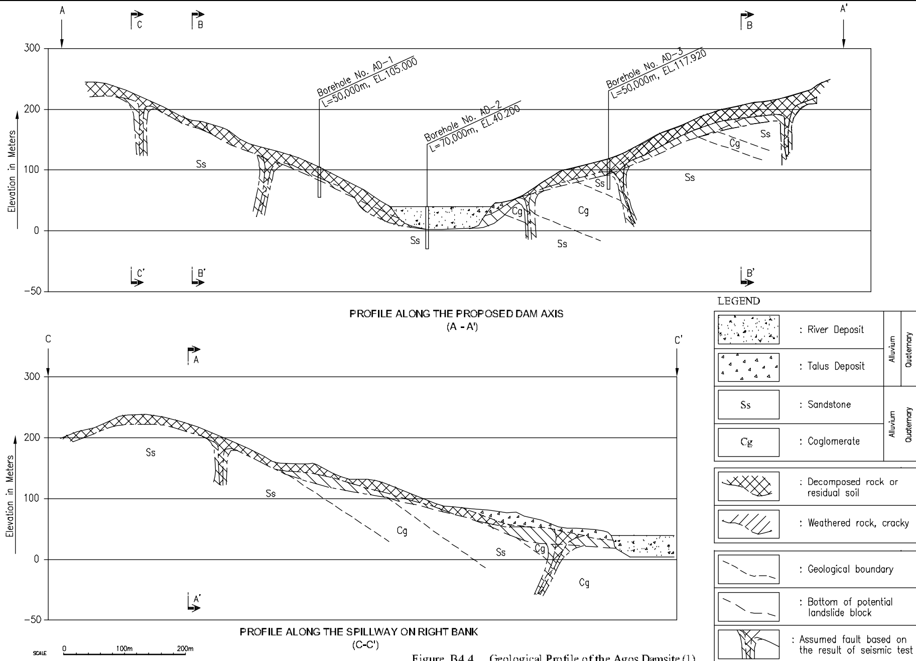
Figure B4.4 Geological Profile of the Agos Damsite (1)
