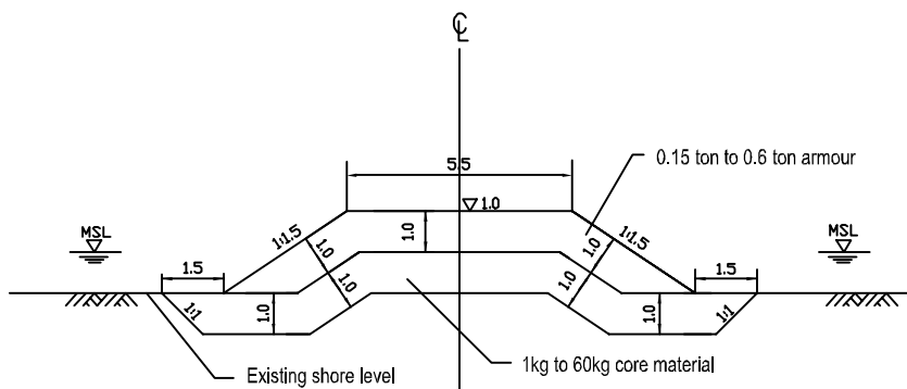
Jetty - Cross Section
