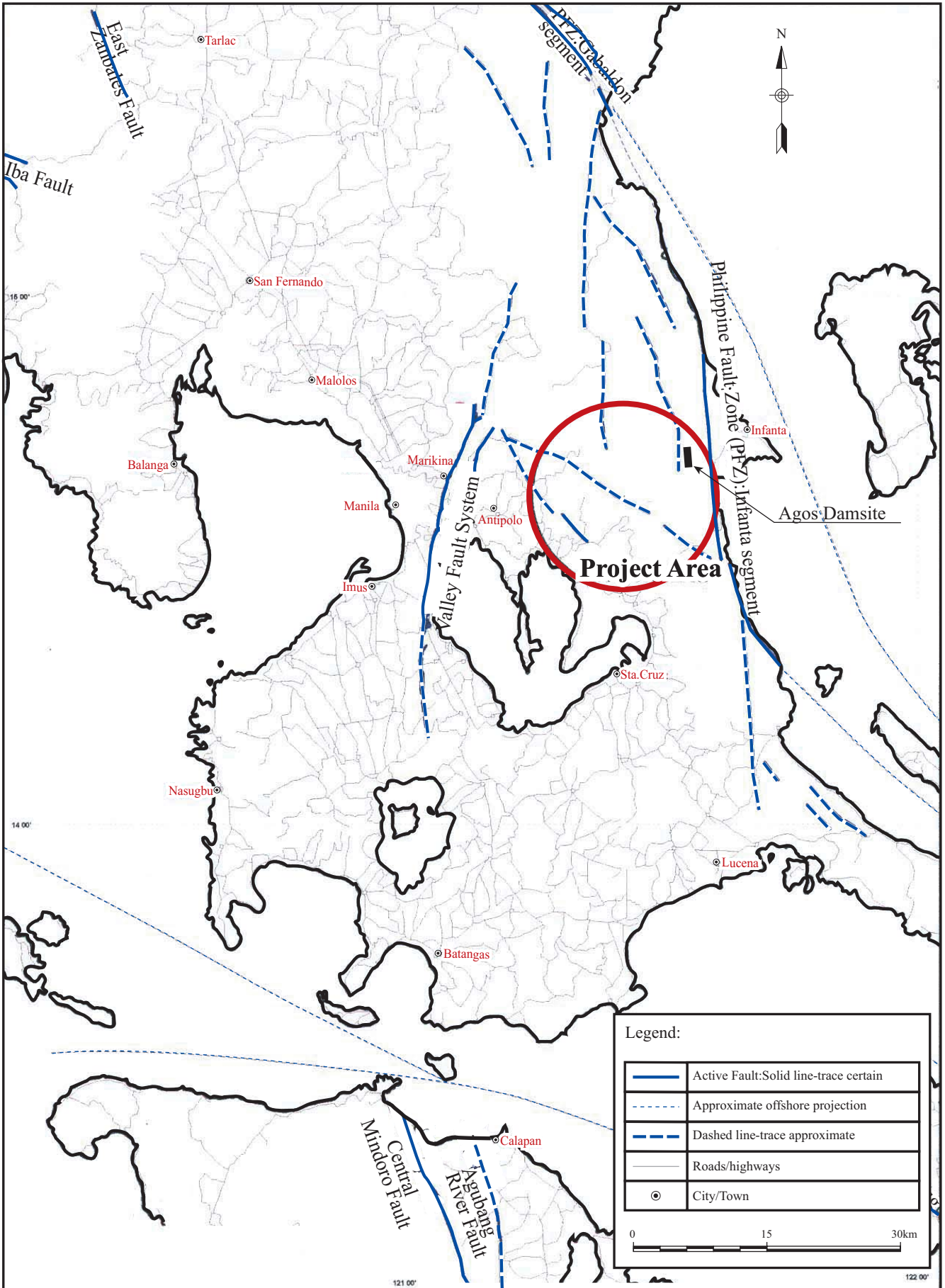
Figure 3.4 Distribution of Active Faults in Southern Luzon
