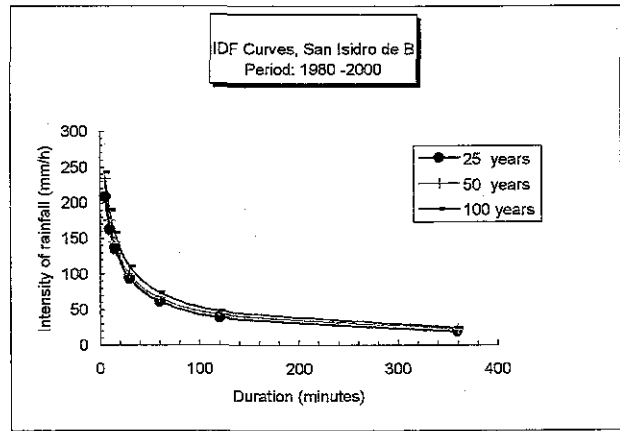
Figure 8.2.3 IDF Curve in San Ishidorode Barbacoa Station
