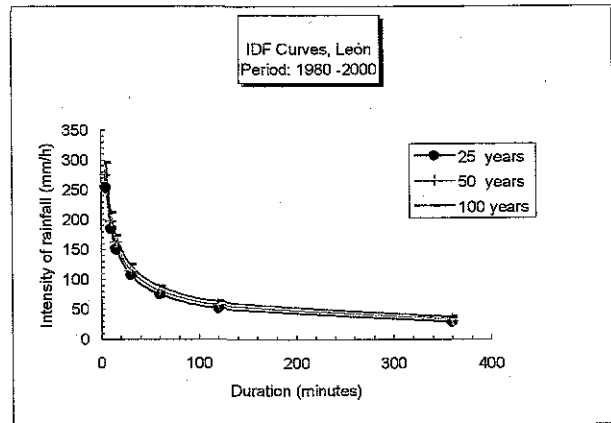
Figure 8.2.5 IDF Curve in Leon Station
