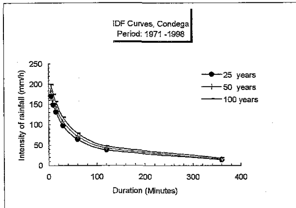
Figure 8.2.4 IDF Curve in Condega Station
