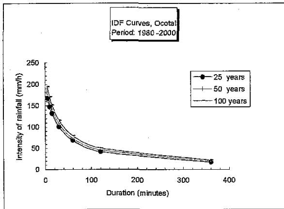
Figure 8.2.2 IDF Curve in Ocotal Station
