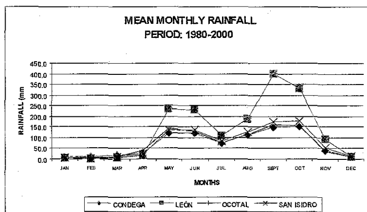
Figure 8.2.1 Rainfall Data in Object Observatory Stations
