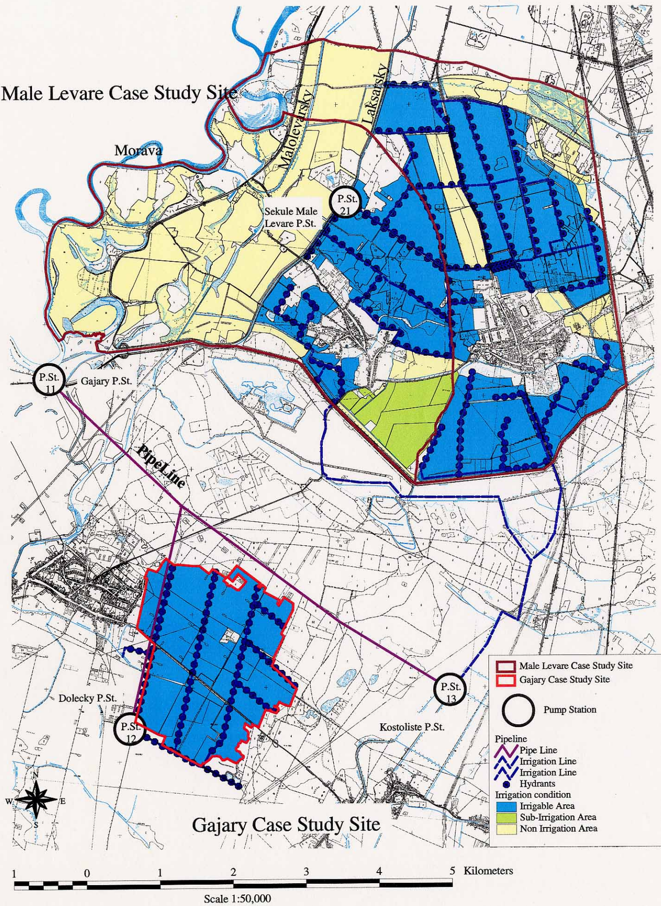
Figure 4.2.2 Irrigation Condition in Case Study Area
