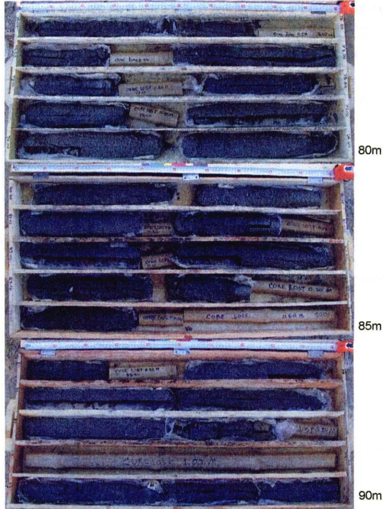
Figure 2.1.3 CH-2 (Girls College) 60-90m THE STUDY ON THE GROUNDWATER DEVELOPMENT OF DEEP AQUIFERS FOR SAFE DRINKING WATER SUPPLY TO ARSENIC AFFECTED AREAS IN WESTERN BANGLADESH JAPAN INTERNATIONAL COOPERATION AGENCY (JICA)
