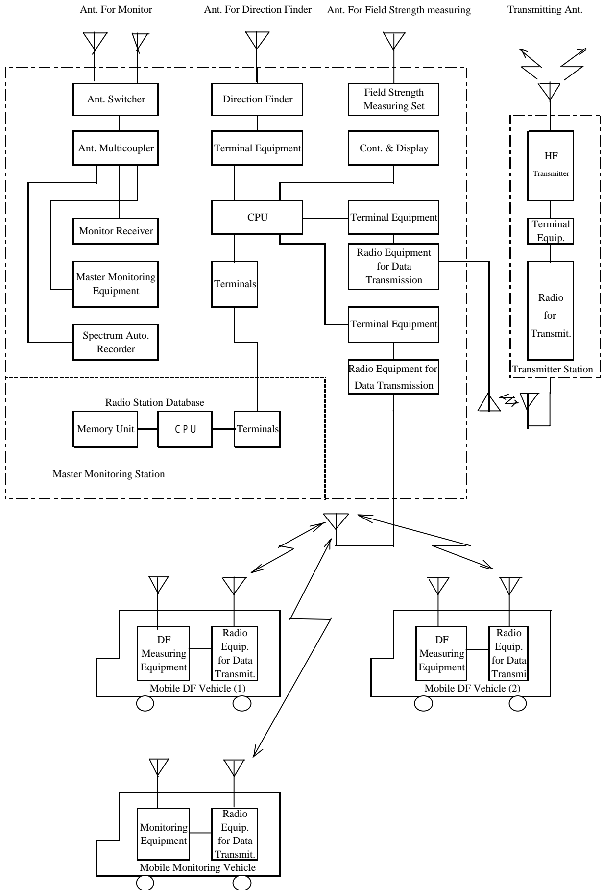
D. Figure 12.3-4 Block Diagram for HF Radio Monitoring and Direction Finding System
