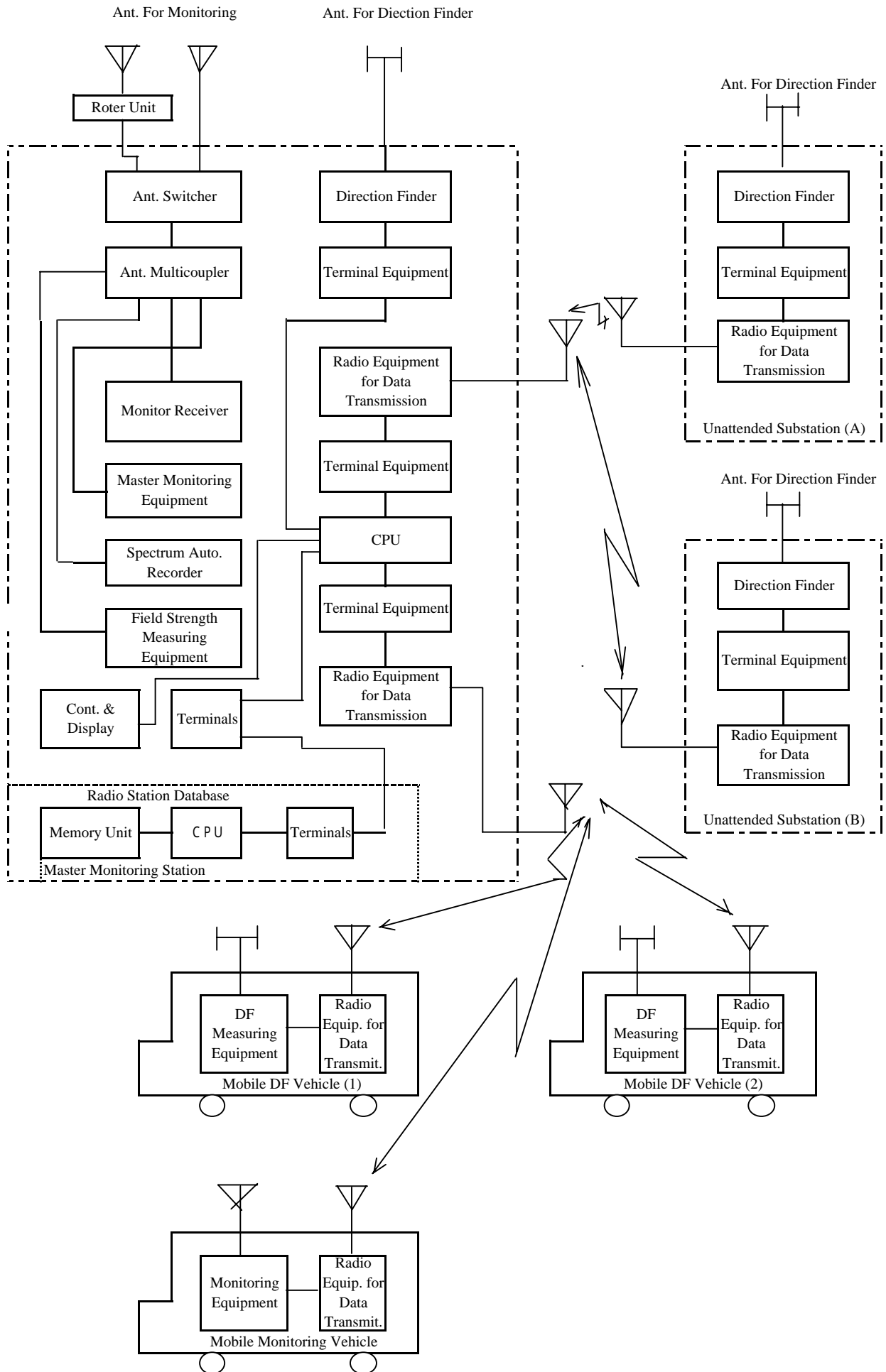
D. Figure 12.3-5 Block Diagram of VHF/UHF Radio Monitoring and Direction Finding System
