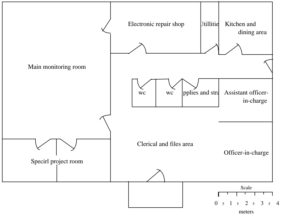
D.Figure 12.3-3 Typical Floor Plan for a Monitoring Station Building
