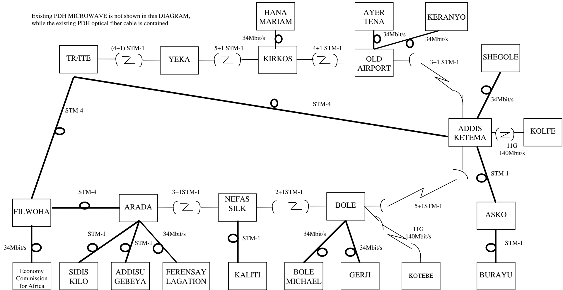
D. Figure 3.3-4 ADDIS ABABA INTEREXCHANGE SDH LINKS (under implementation)
