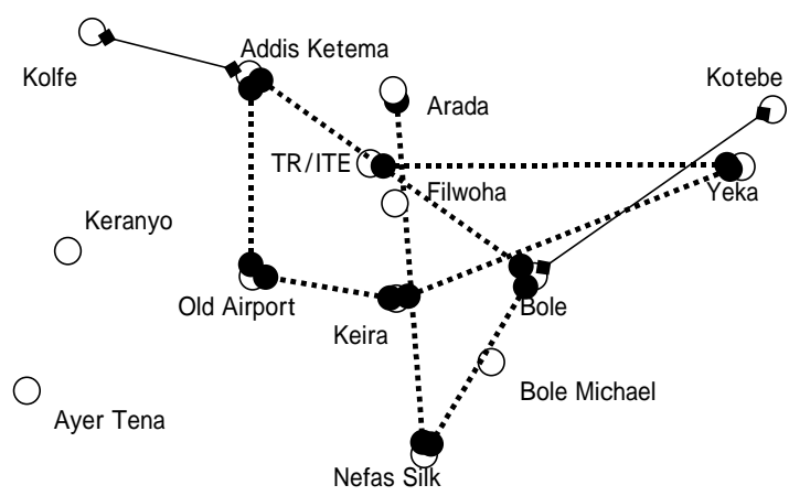
D.Figure 3.3-3 (b)ETC's MAIN RADIO FREQUENCY USAGE in ADDIS ABABA and Mt.FURI (ADDITIONAL LINK in NEW PLAN)
