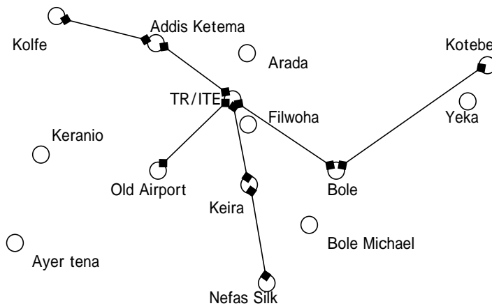
D. Figure 3.3-3(a) ETC's MAIN RADIO FREQUENCY USAGE in ADDIS ABABA and Mt.FUR (EXISTING)
