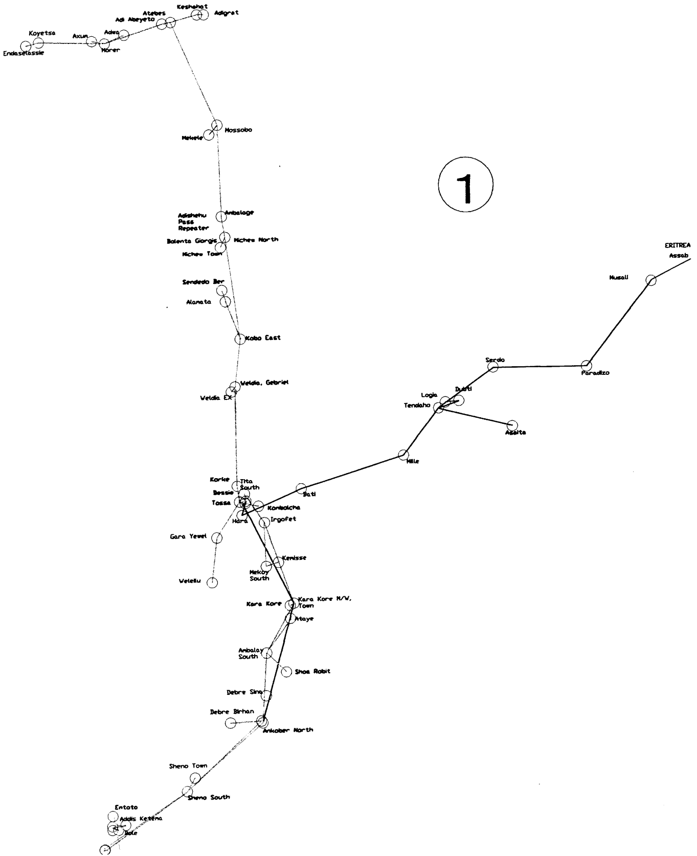
D. Figure 3.3.2 (2/7) Existing Microwave Route Map (Northern Route)
