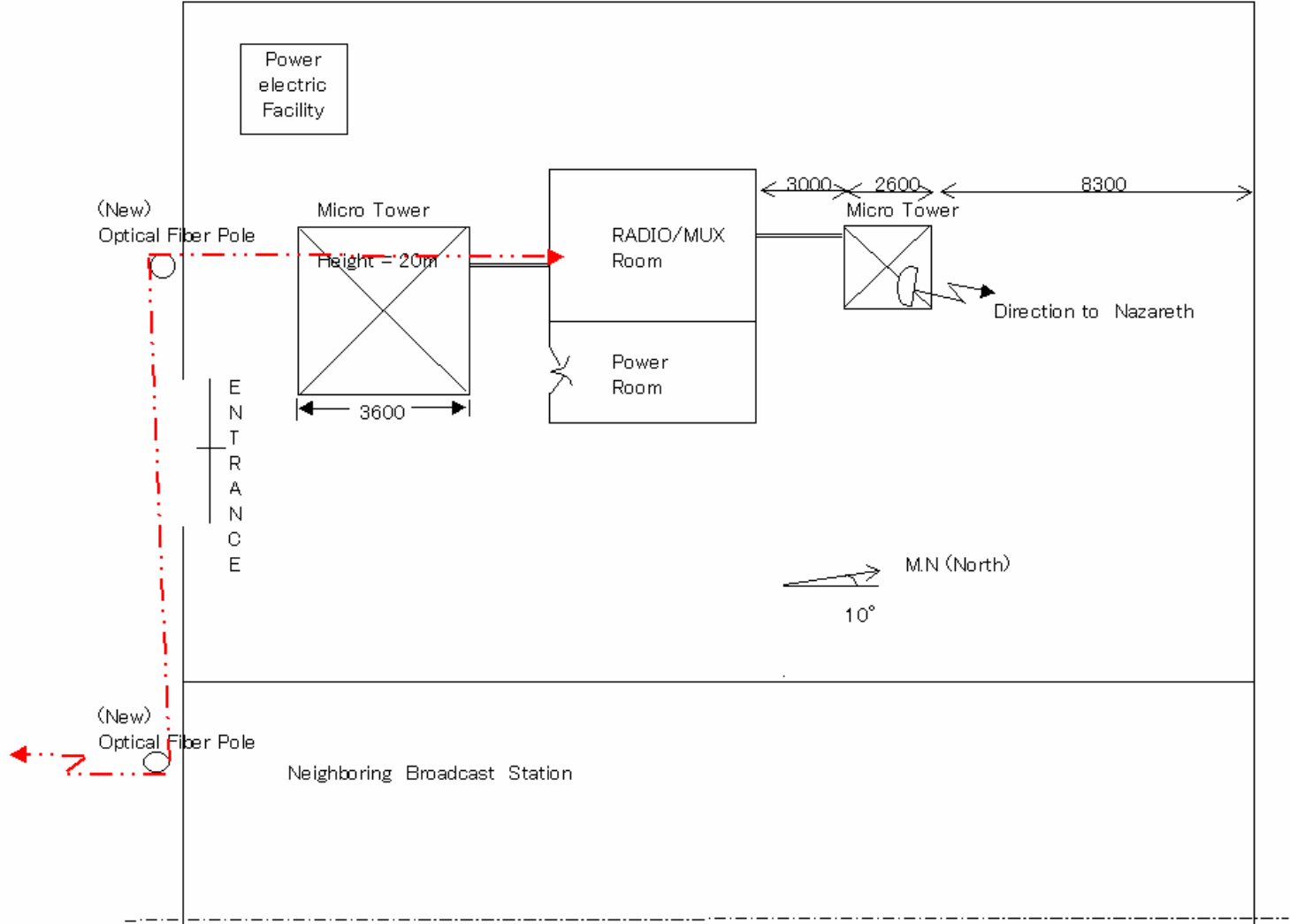
Fig . 5.3.5-5 ADAMA WEST MW Rep. Cable Laying Point
