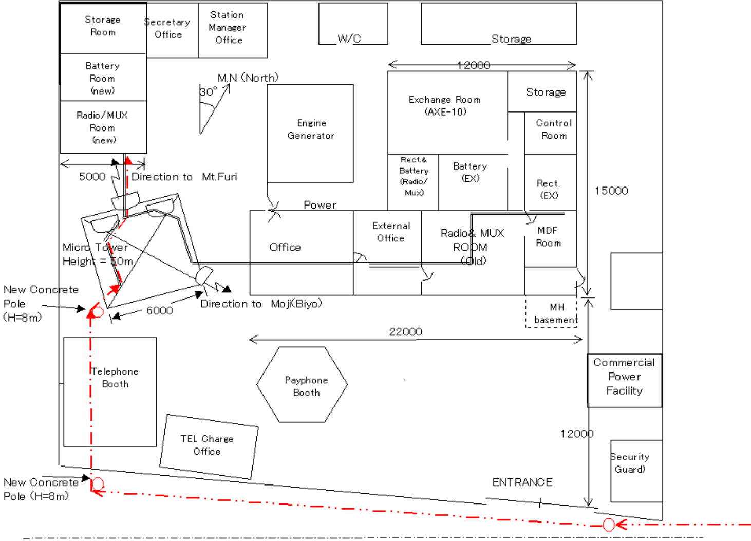
Fig . 5.3.5-4 Debre Zeit Cable Laying Point
