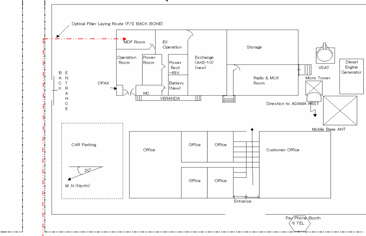
Fig . 5.3.5-6 Nazareth Primary Center Cable Laying Point
