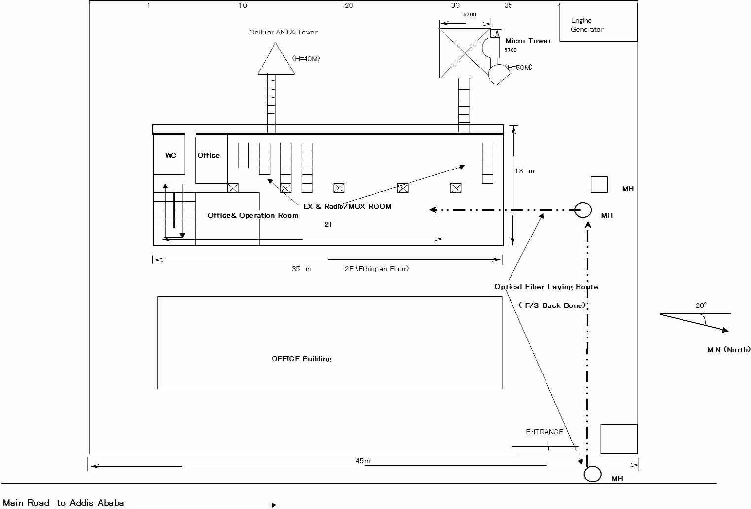
Fig .5.3.5-3 AA NEFAS Silk Cable Laying Point
