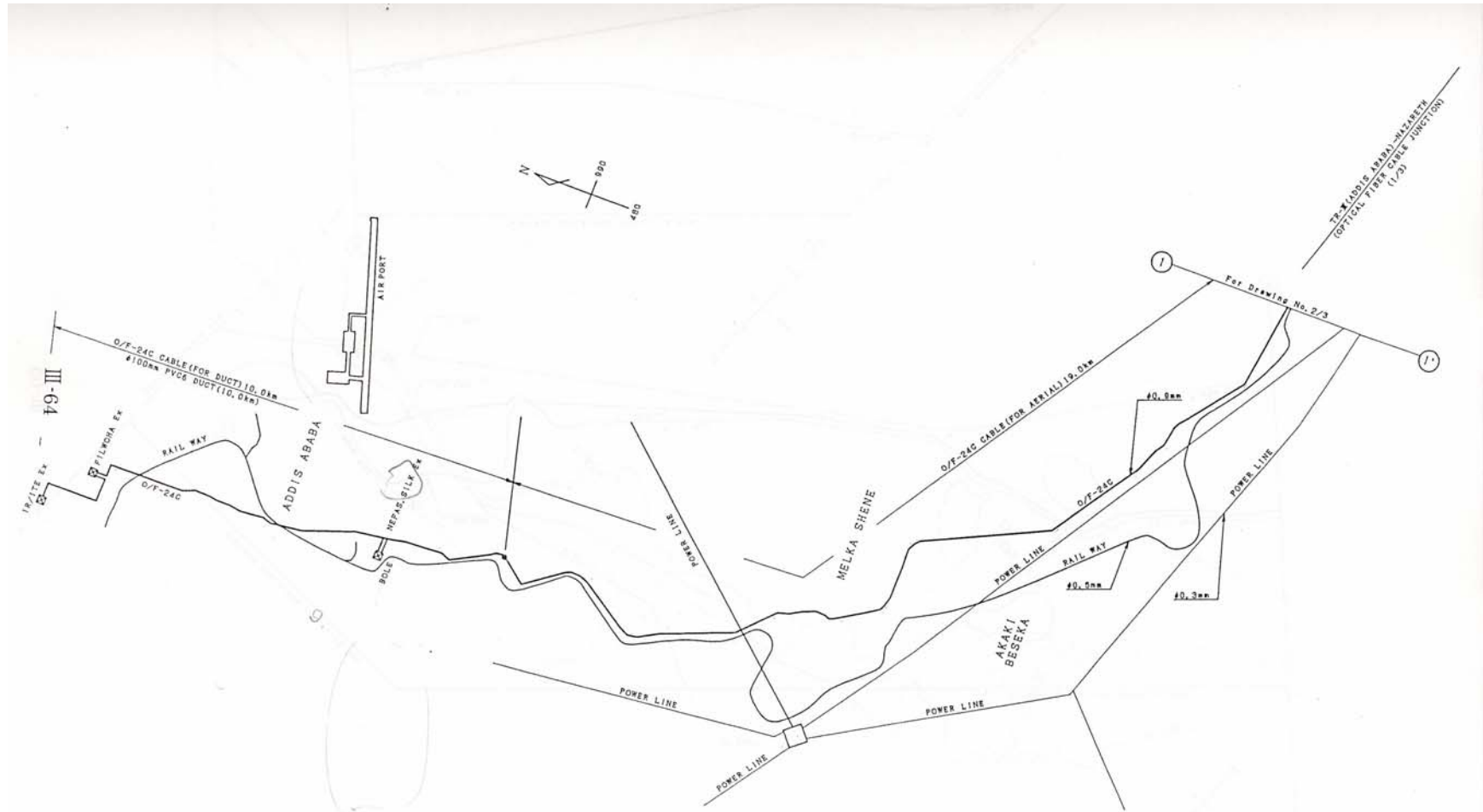
Figure 5.3.3 (1/3) Optical Fiber Laying Route (Addis Ababa Nazareth/Outer city)
