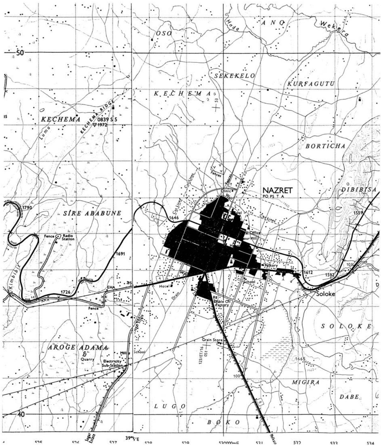
Fig.5.3.4 Optical Fiber Laying Route (Nazareth)
