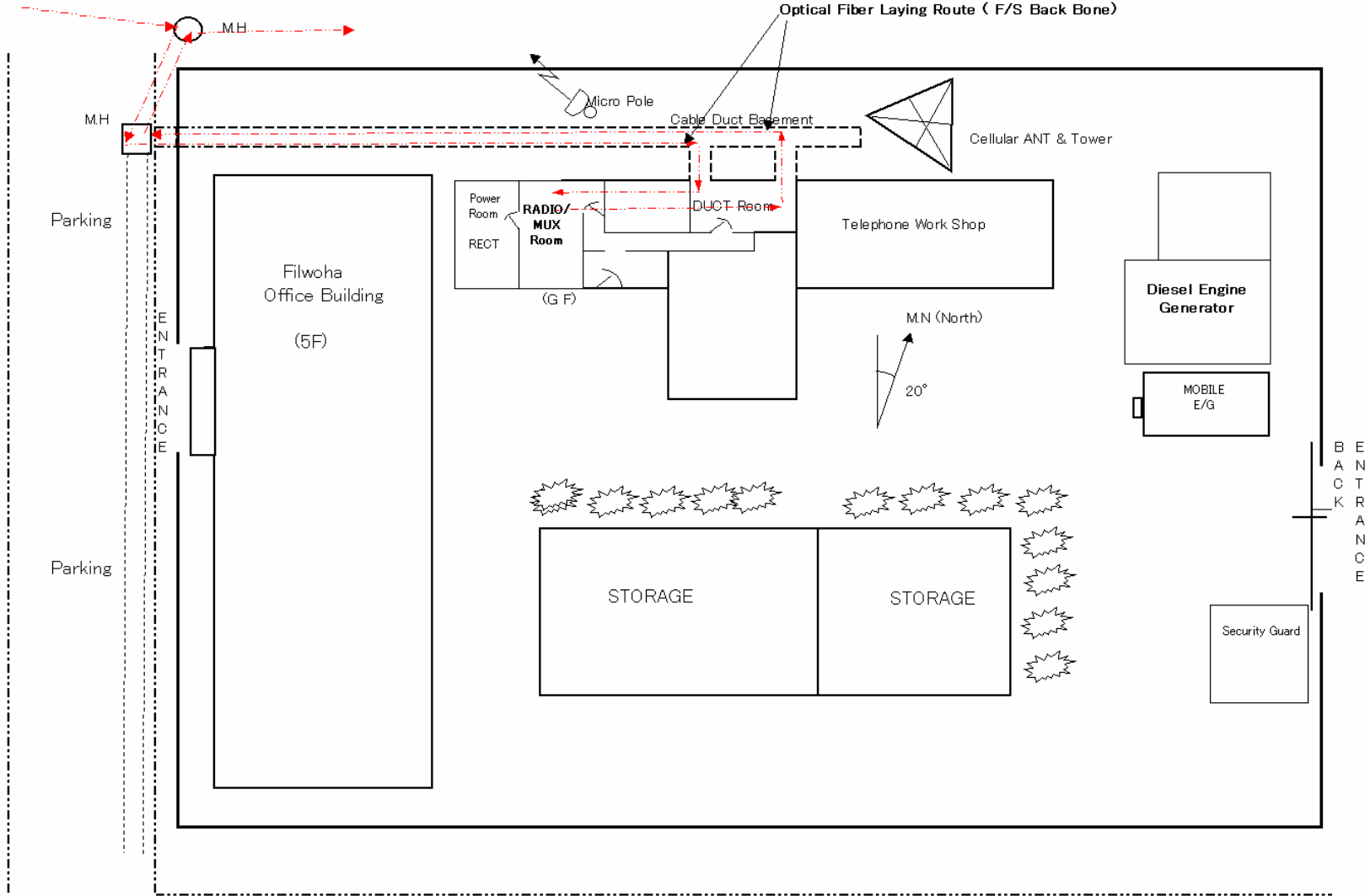
Fig . 5.3.5-2 AA FILWOHA Center Cable Laying Point
