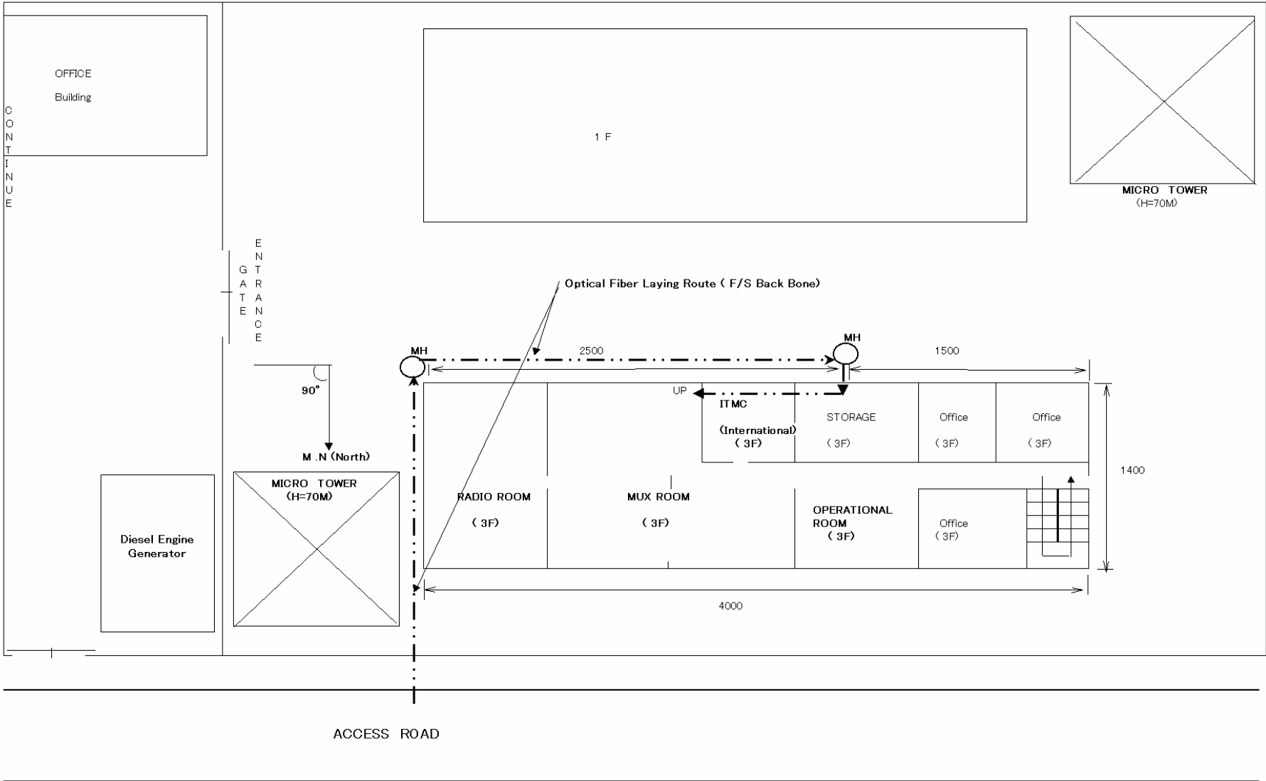
Fig . 5.3.5-1 Addis Ababa IR/ITE Center Cable Laying Point
