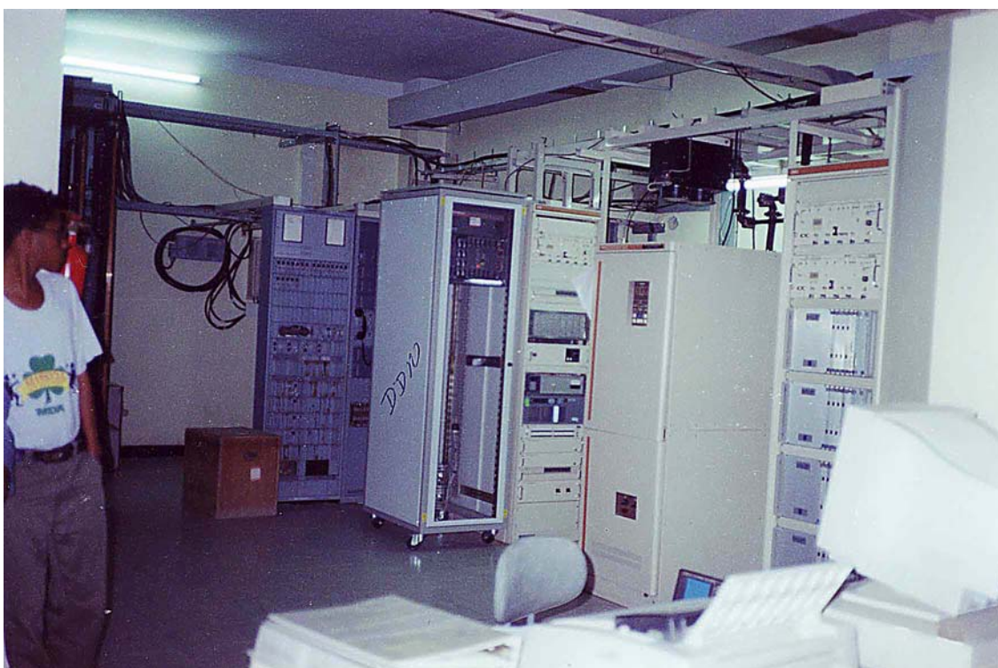
Photo-No.1-4, Transmission Equipment Room (2F), Mekele PC
