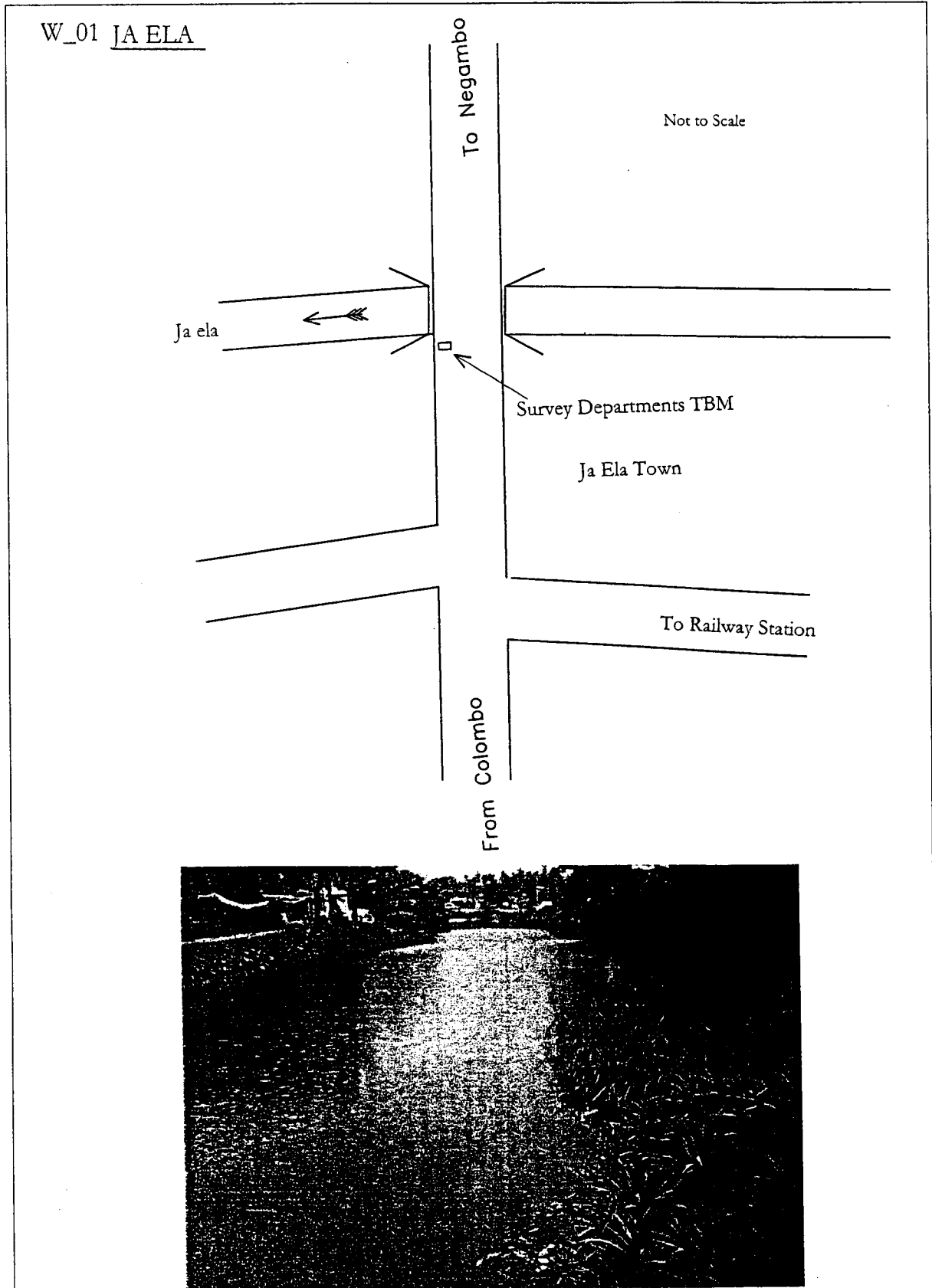
The Study on Storm Water Drainage Plan for the Colombo Metropolitan Region in the Democratic Socialist Republic of Sri Lanka JAPAN INTERNATIONAL COOPERATION AGENCY Sketch of Water Level Gauging Station W01
