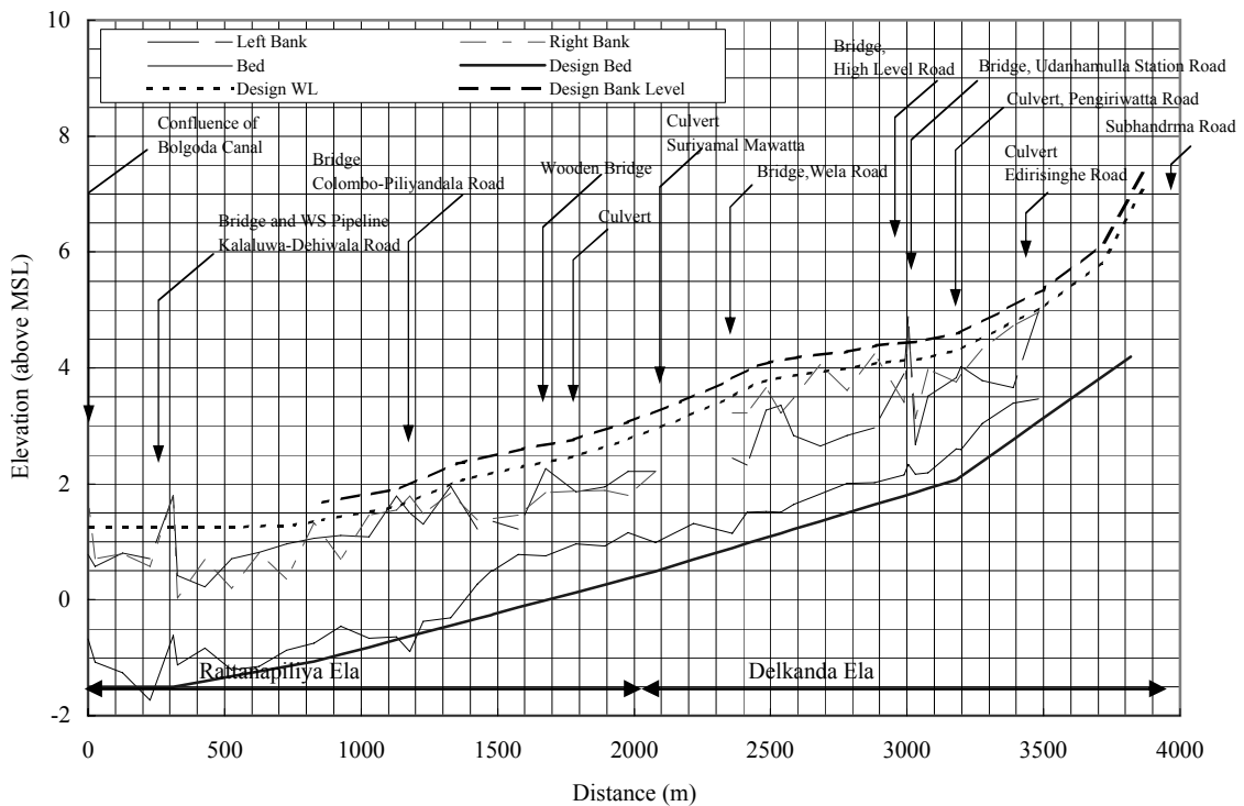
Figure 4.5.5 Longitudinal Profiles of Channel Improvement for Nugegoda Ela, Delkanda Ela and Rattanapitiya Ela
