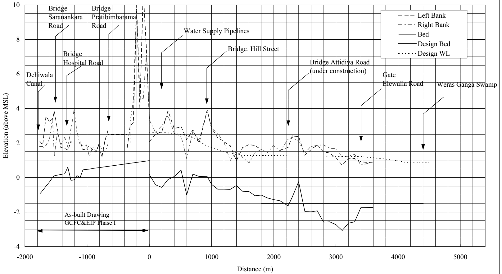
Figure 4.5.7 Longitudinal Profile of Channel Improvement of Bolgoda Canal
