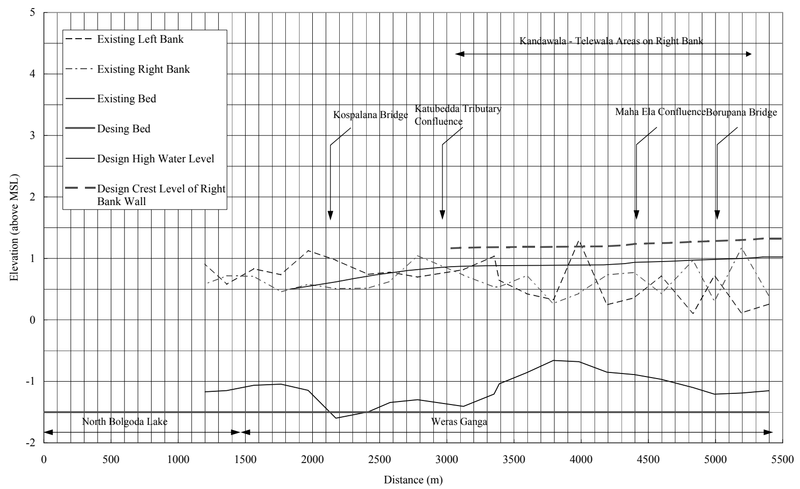
Figure 4.5.3 Longitudinal Profile of Channel Improvement of Weras Ganga Scheme
