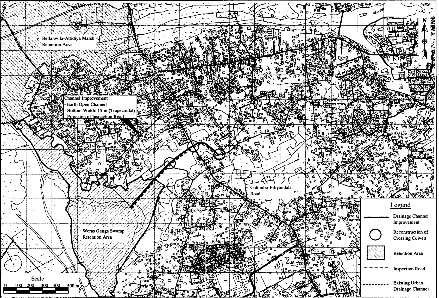
Figure 4.5.9 Boralessgamuwa South Scheme
