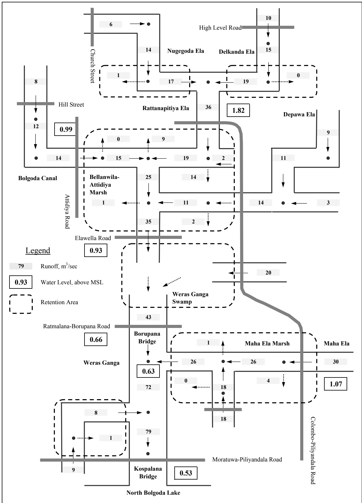
Figure 4.4.4 Distribution of Design Flood Runoff (1/6) (2-year Return Period)
