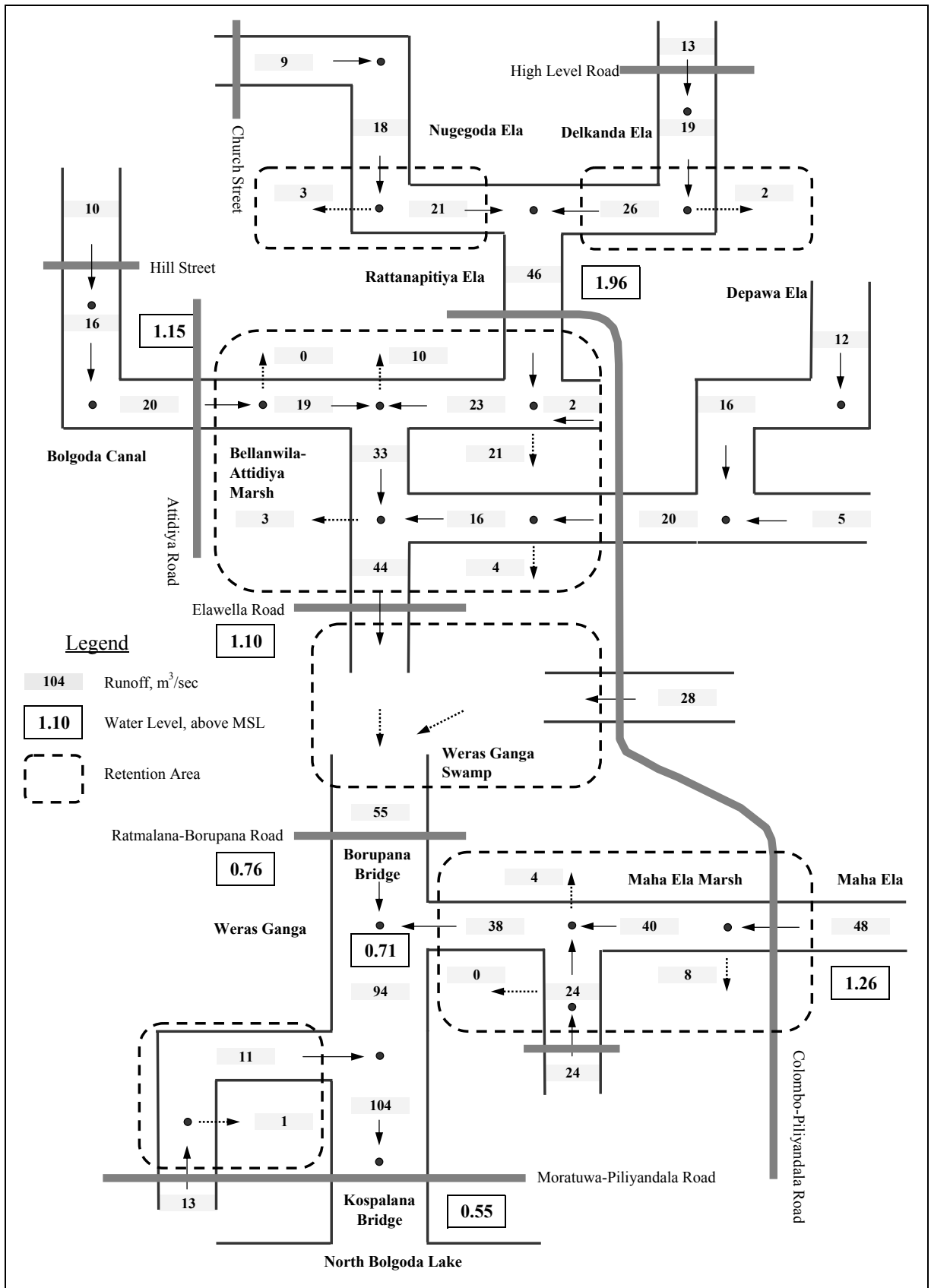
Figure 4.4.4 Distribution of Design Flood Runoff (2/6) (5-year Return Period)
