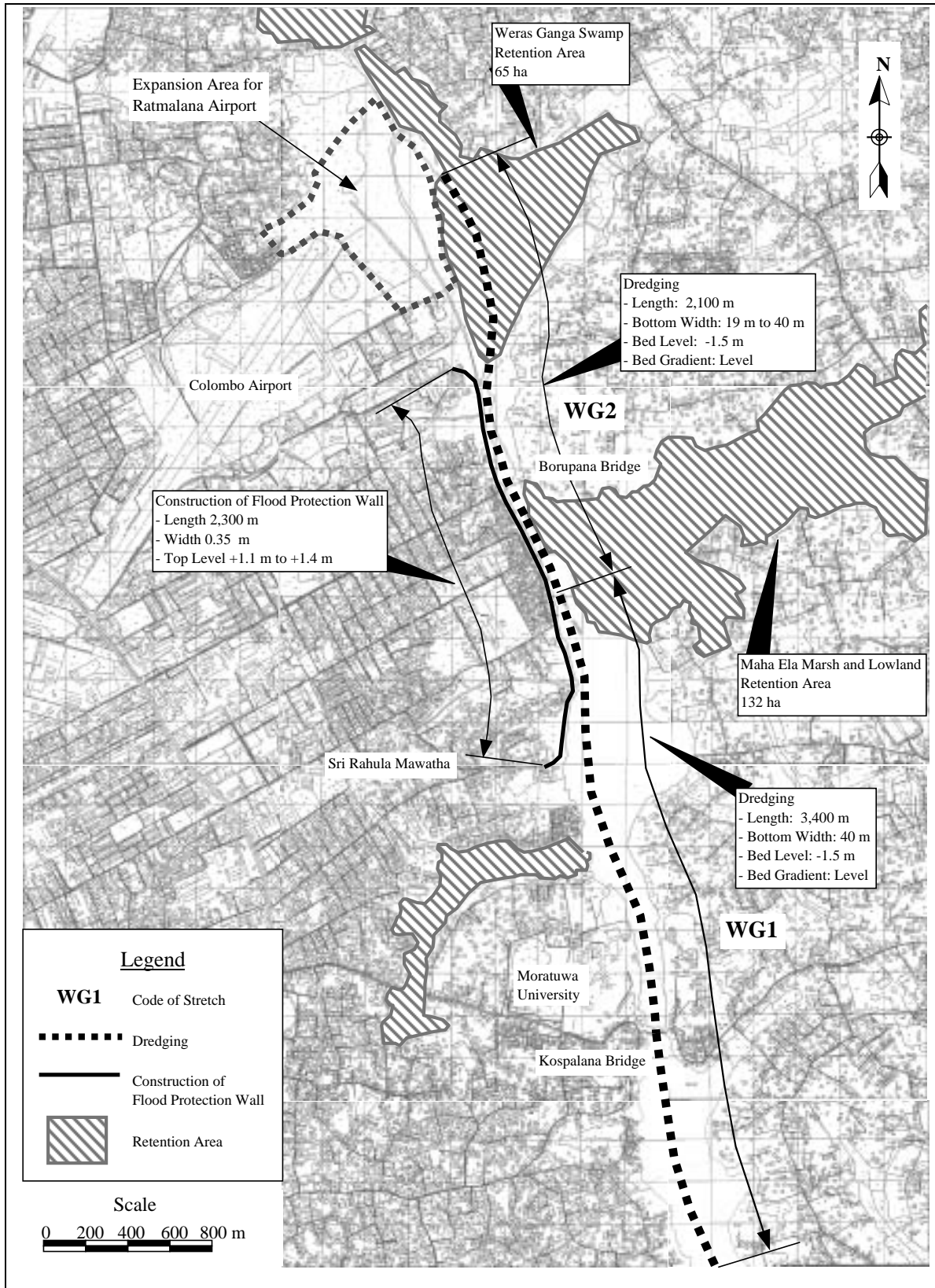
Figure 4.5.2 Weras Ganga Scheme
