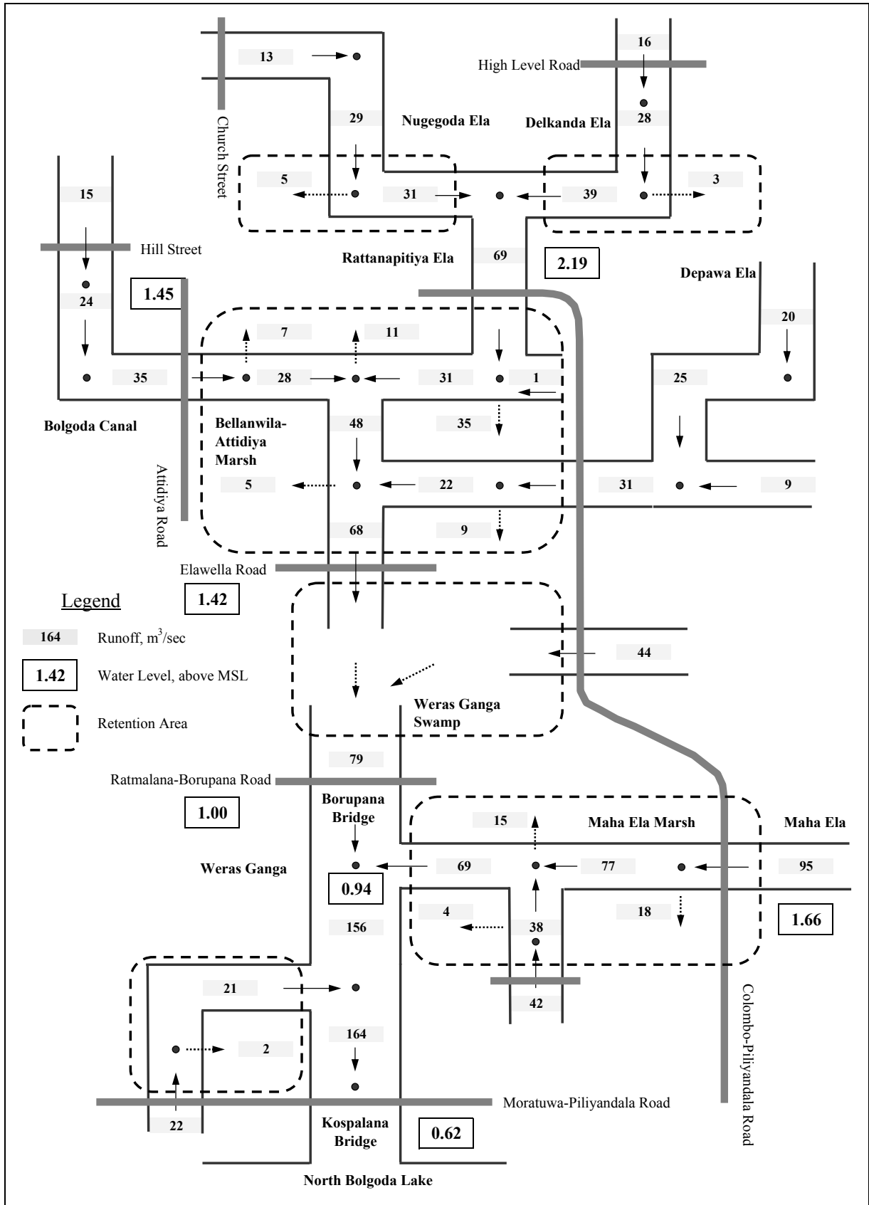
Figure 4.4.4 Distribution of Design Flood Runoff (5/6) (50-year Return Period)
