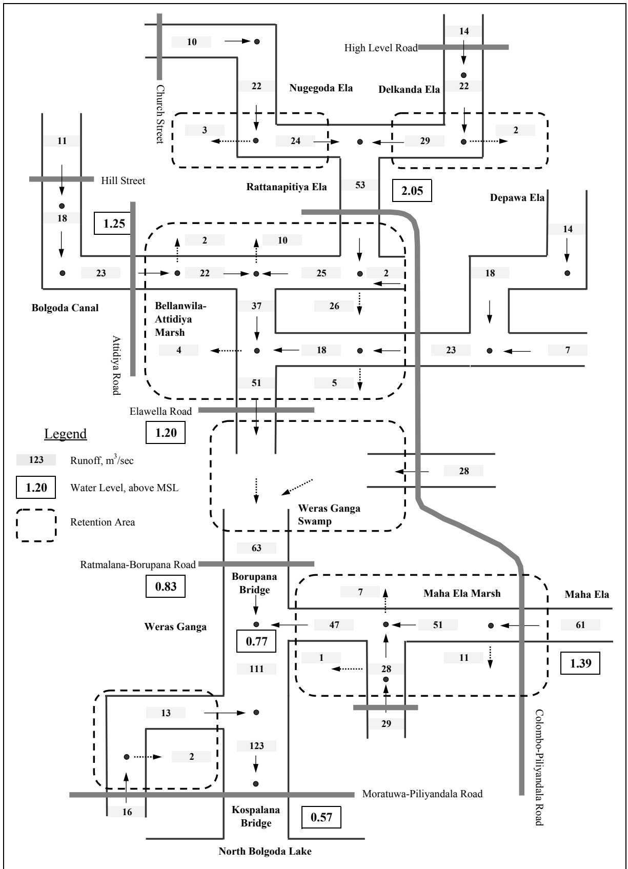
Figure 4.4.4 Distribution of Design Flood Runoff (3/6) (10-year Return Period)
