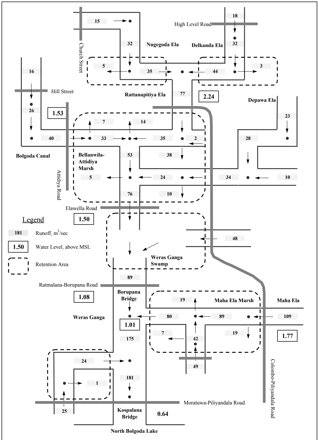
Figure 4.4.4 Distribution of Design Flood Runoff (6/6) (100-year Return Period)
