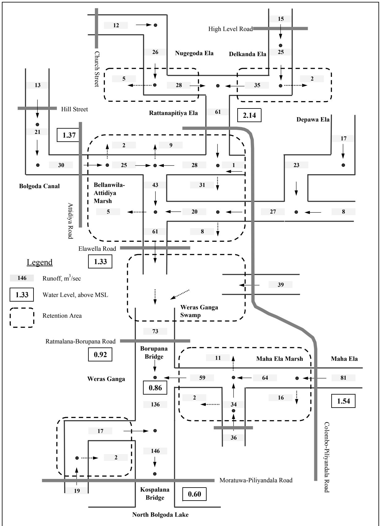
Figure 4.4.4 Distribution of Design Flood Runoff (4/6) (25-year Return Period)
