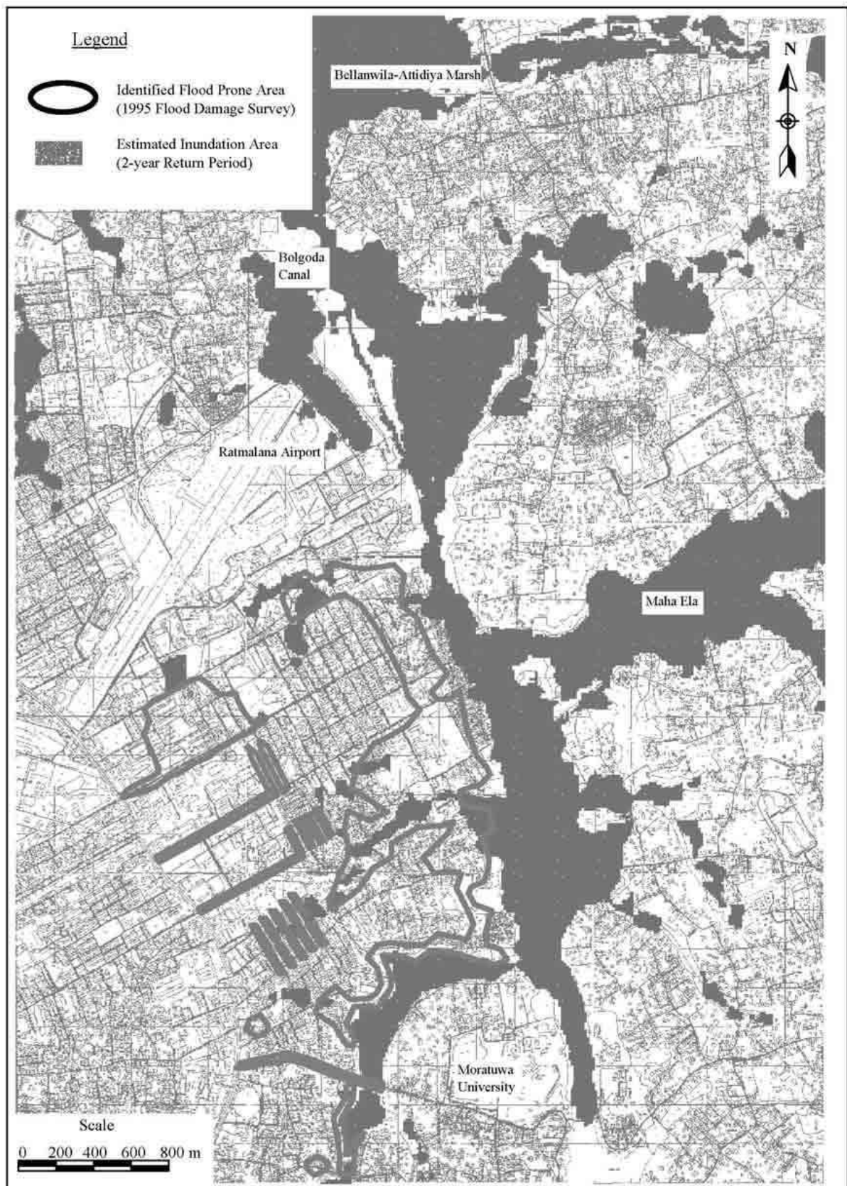
Figure 3.7.1 Flooding Area in Ratmalana-Moratuwa Sub-basin (2/2) (1995 Flood Damage Survey)
