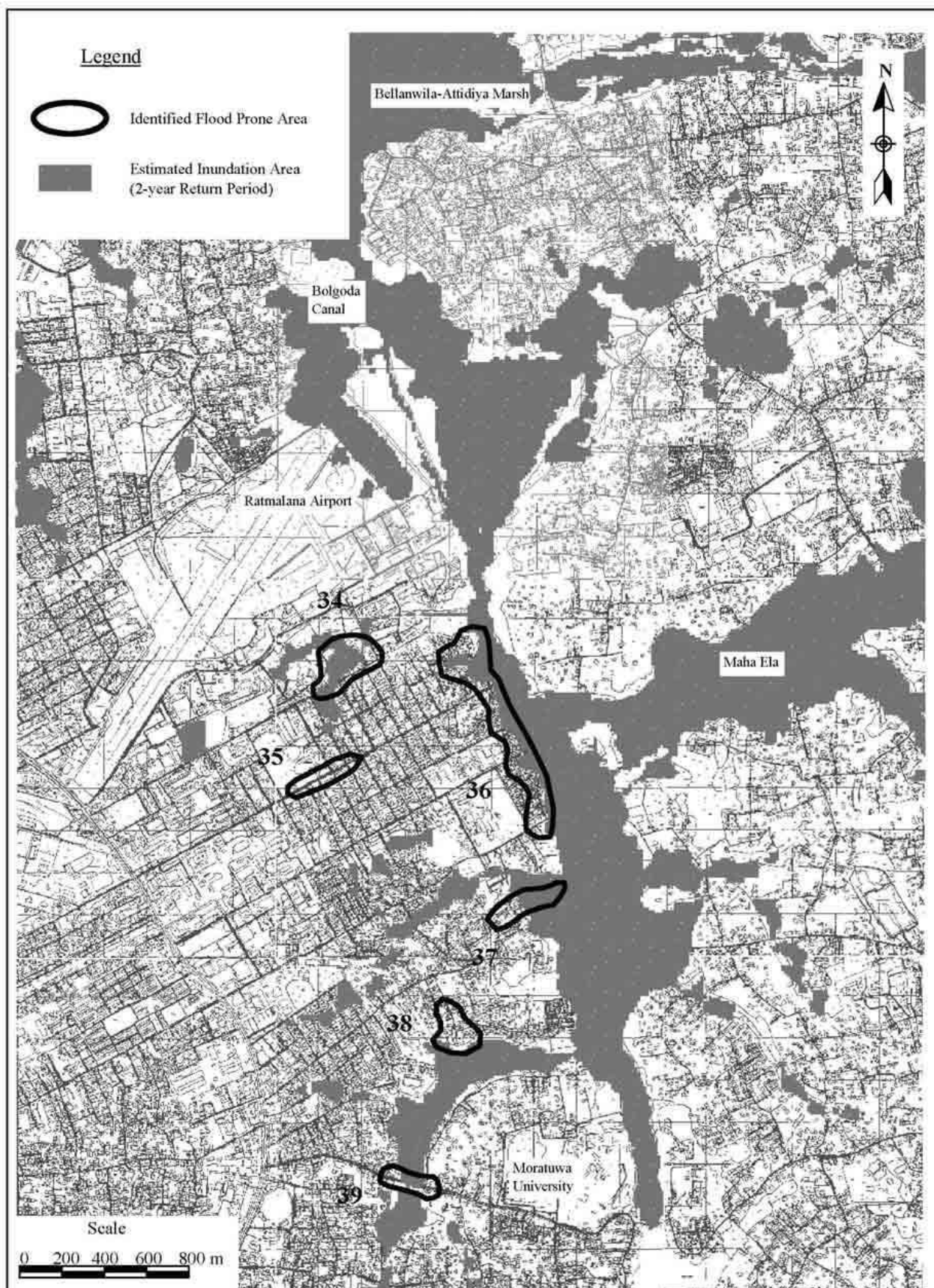
Figure 3.7.1 Flooding Area in Ratmalana-Moratuwa Sub-basin (1/2) (2001 Flood Damage Survey)
