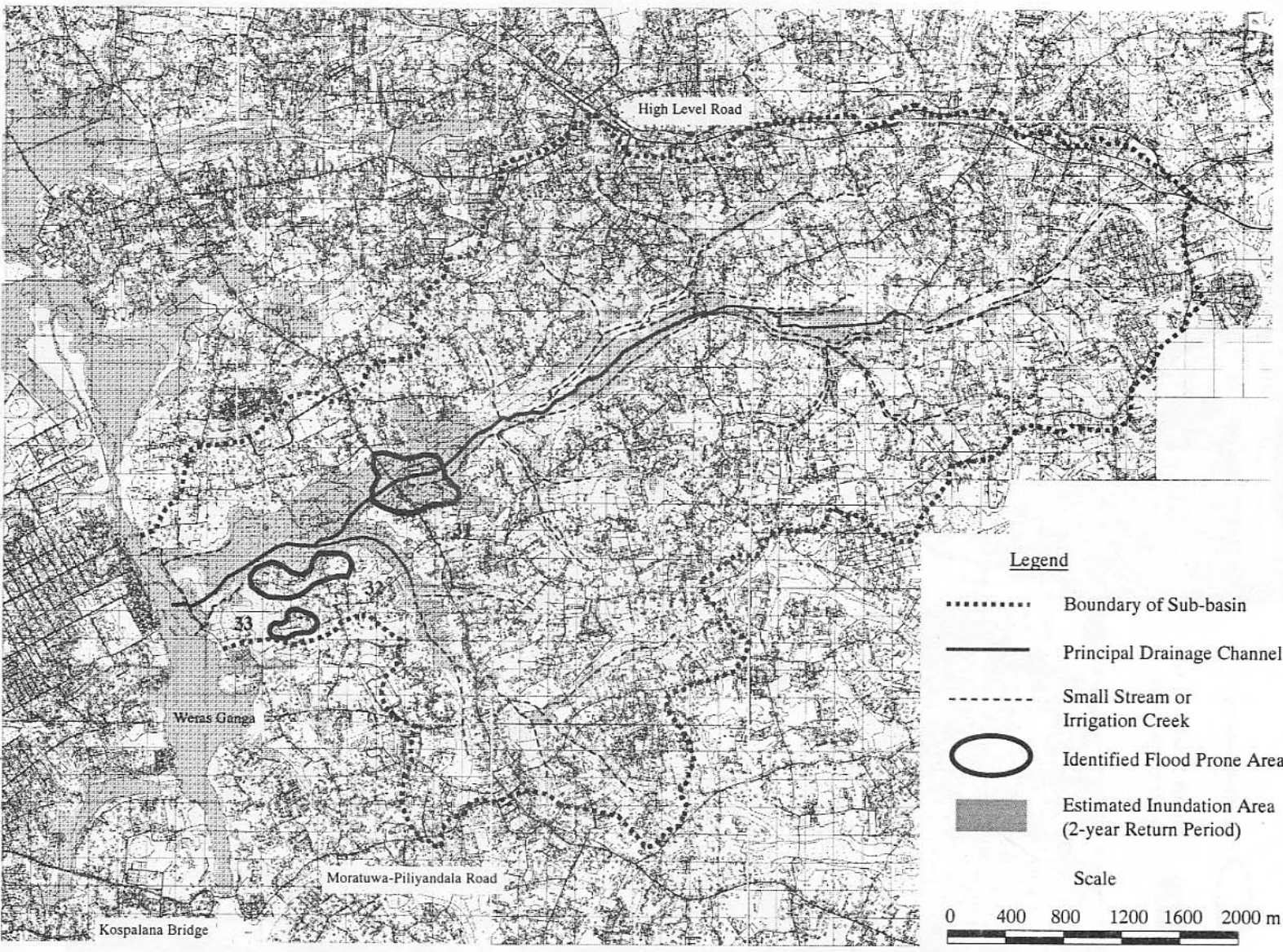
Figure 3.6.1 Flood Prone Areas in Maha Ela Sub-basin
