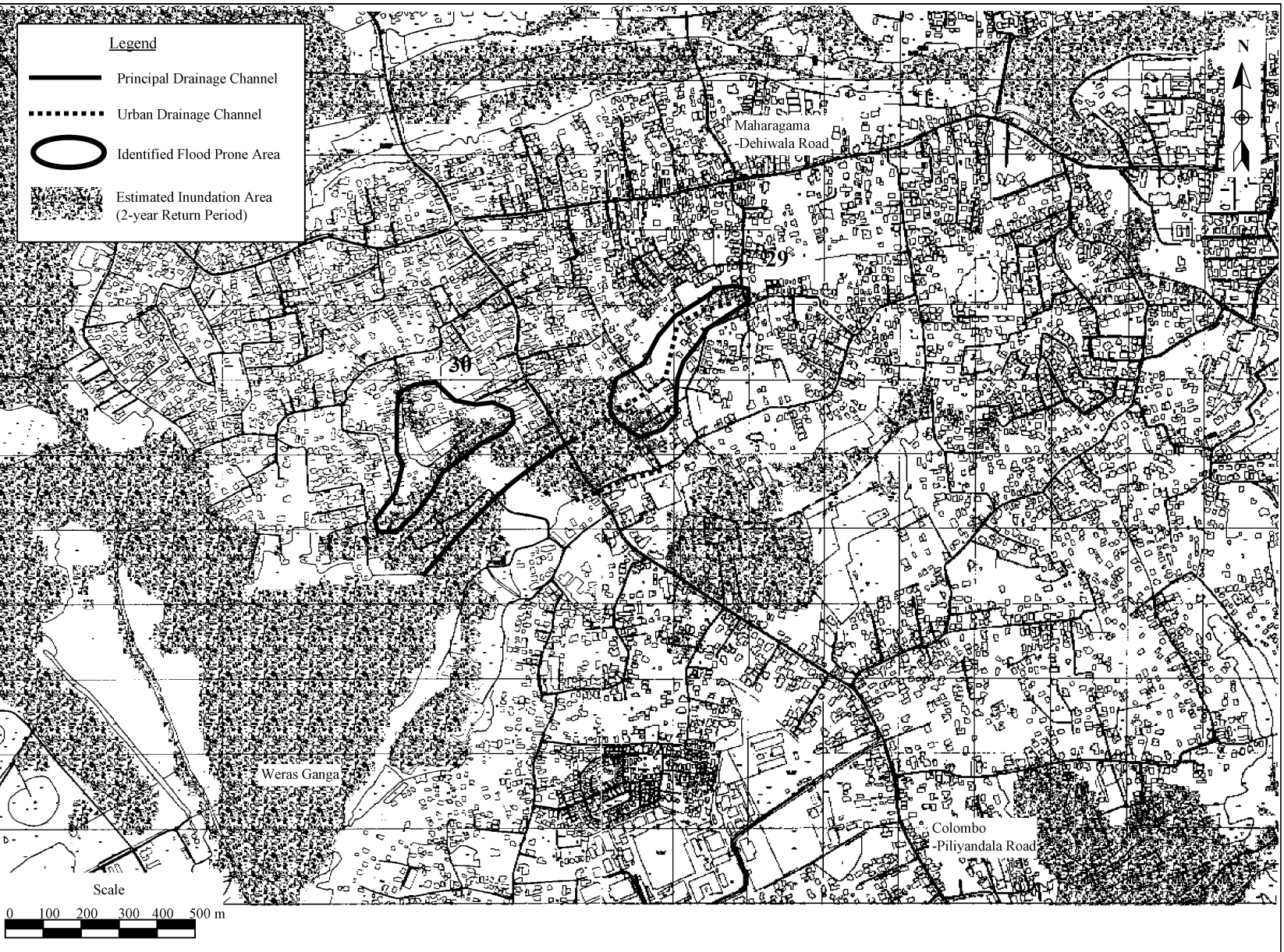
Figure 3.5.1 Flood Prone Areas in Boralesgamuwa South Sub-basin
