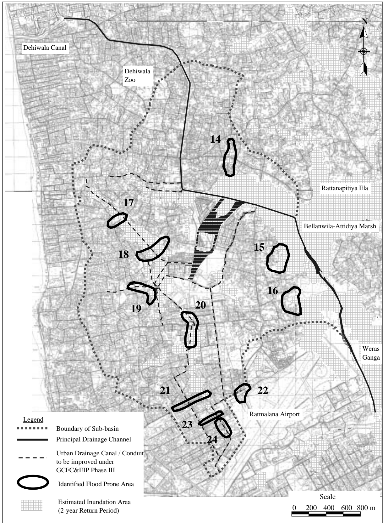
Figure 3.3.1 Flooding Area in Bolgoda Canal Sub-basin (1/2) (2001 Flood Damage Survey)
