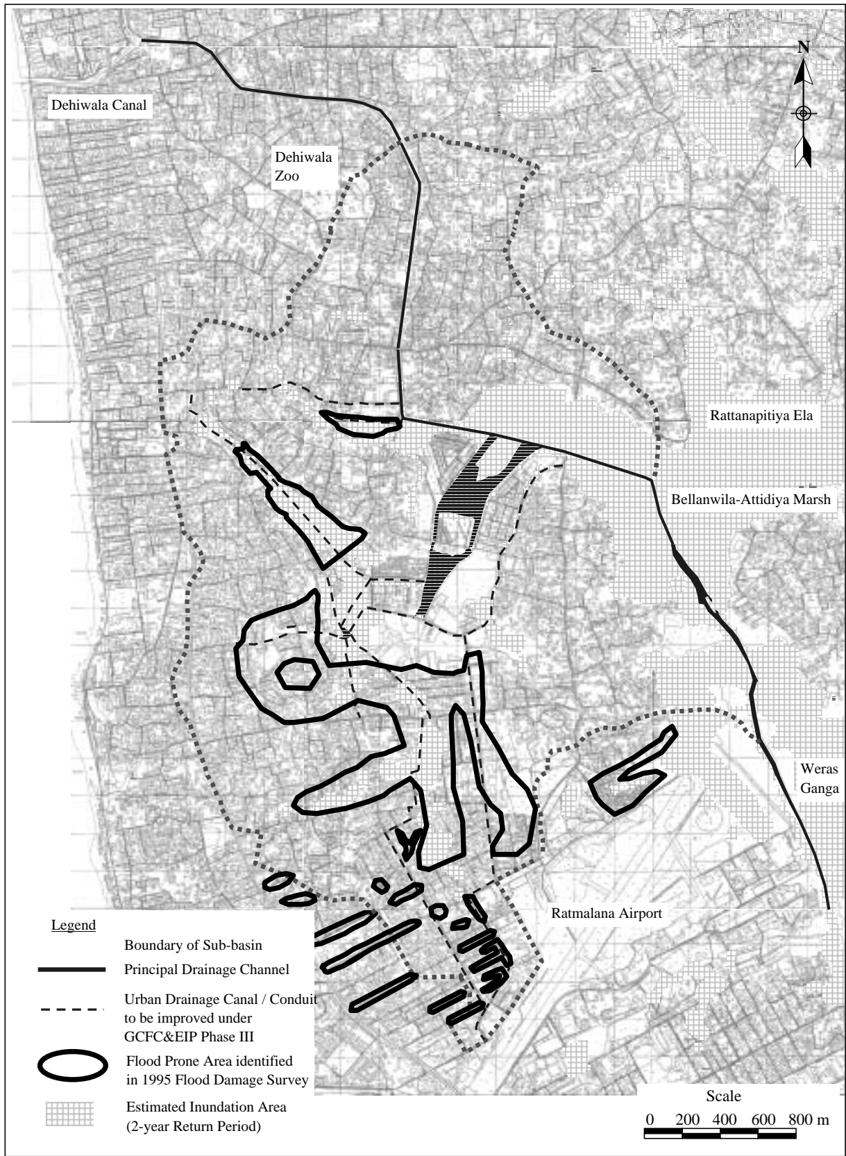
Figure 3.3.1 Flooding Area in Bolgoda Canal Sub-basin (2/2) (1995 Flood Damage Survey)
