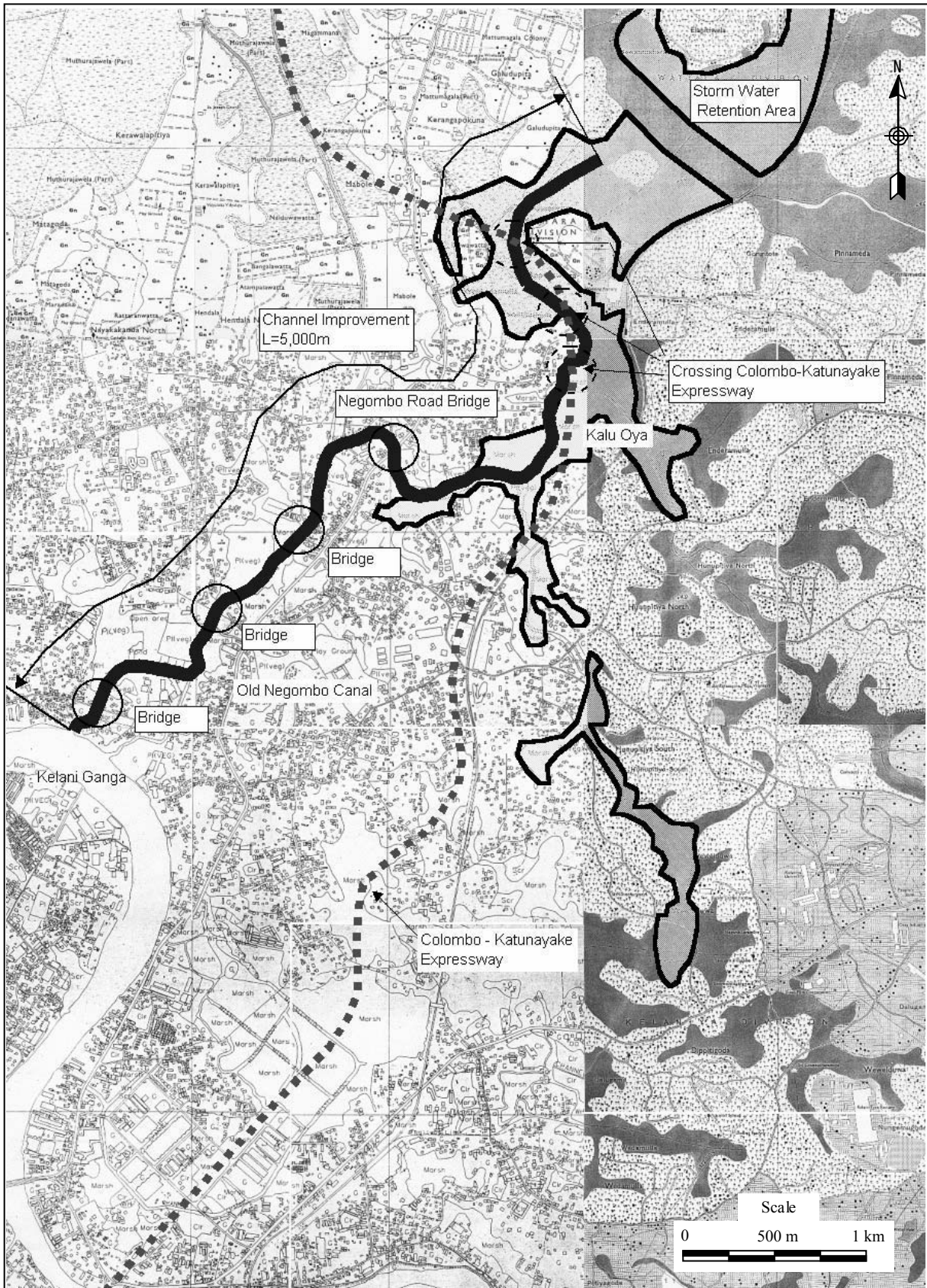
Figure 6.3.2 General Plan of Kalu Oya – Old Negombo Canal Improvement
