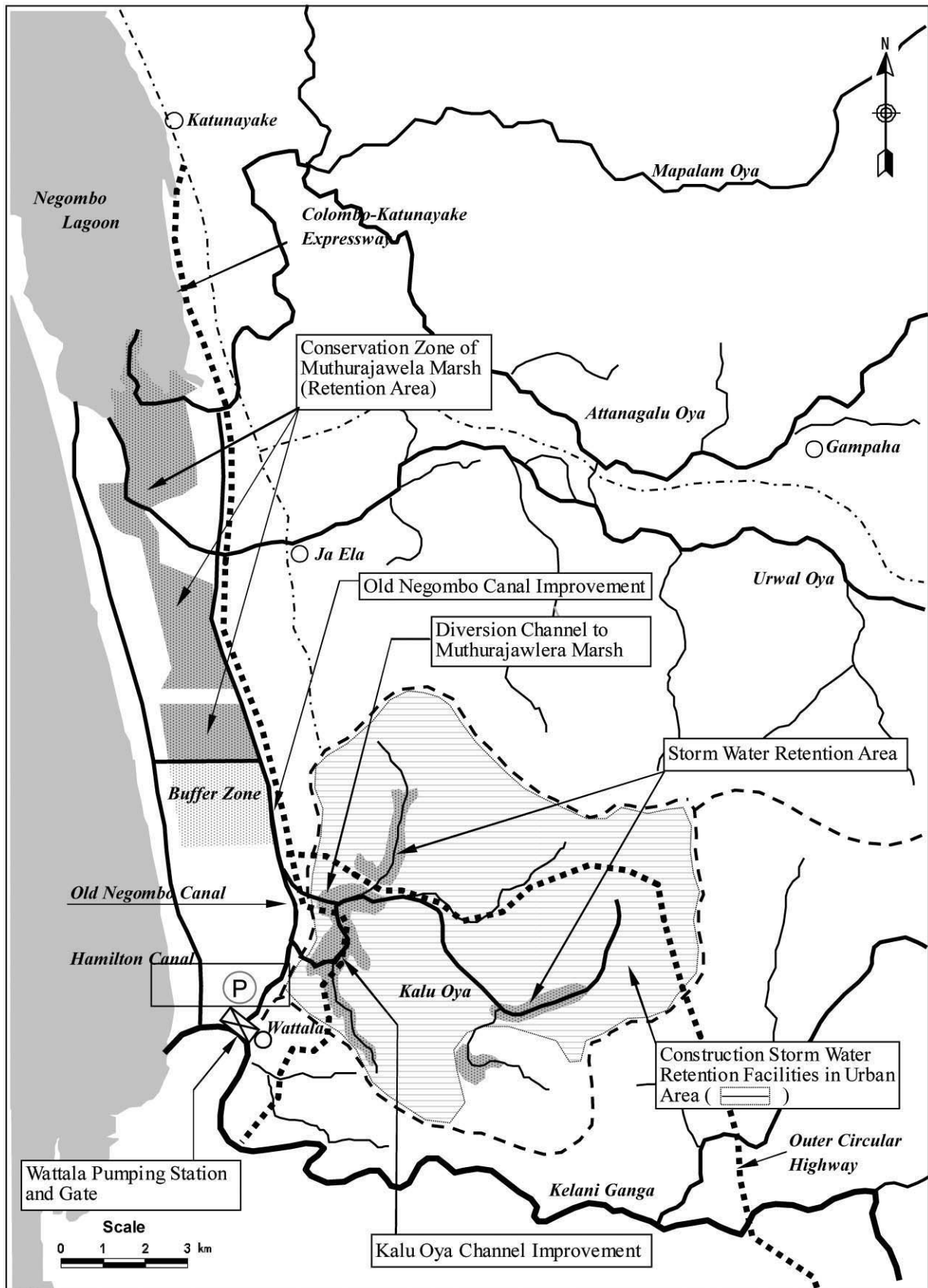
Figure 6.3.1 Conceivable Structural Measures for Kalu Oya Basin
