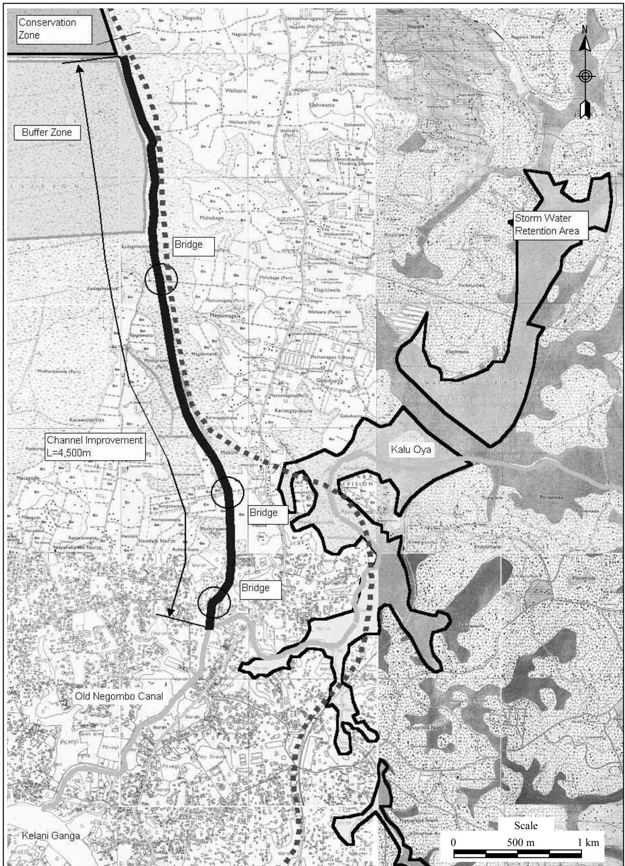
Figure 6.3.3 General Plan of Old Negombo Canal Improvement to Muthurajawela Marsh
