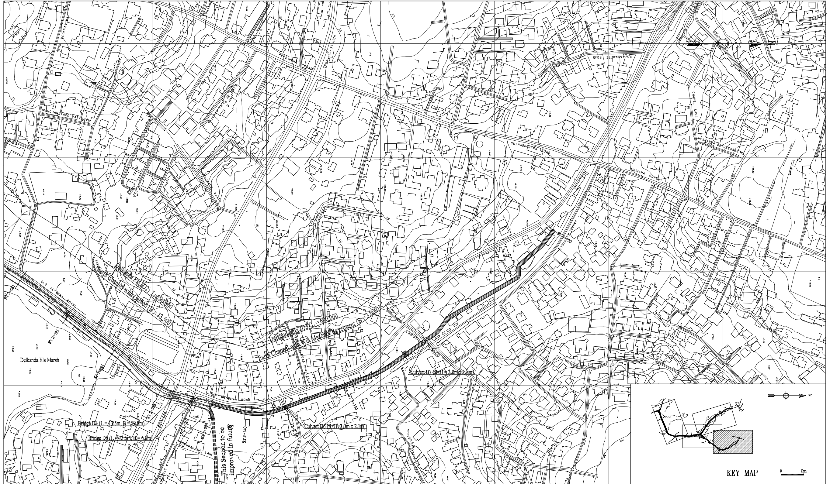
The Study on Storm Water Drainage Plan for the Colombo Metropolitan Region in the Democratic Socialist Republic of Sri Lanka JAPAN INTERNATIONAL COOPERATION AGENCY Drawing 14 Plan of Proposed Rattanaipitiya Ela and Delkanda Ela Channel Improvement (3/3)
