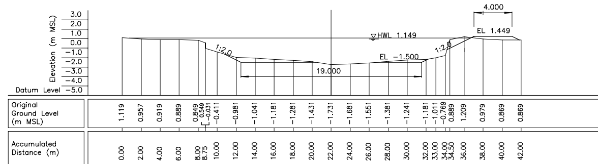
TYPICAL CROSS SECTION (ST 0+670)
