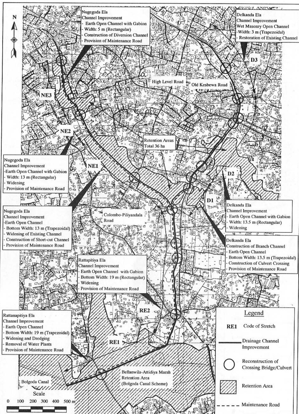
Figure 15.11 Nugegoda-Rattapitiya Scheme
