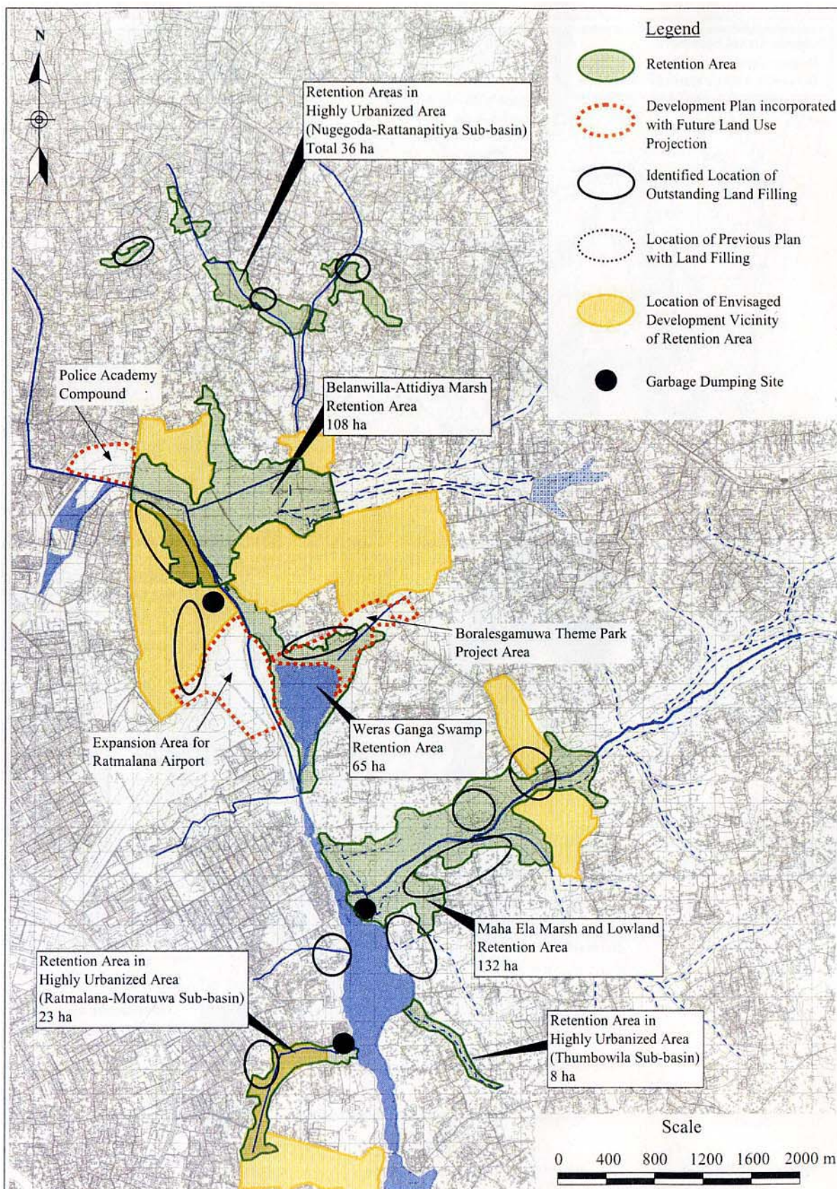
Figure 4.48 Retention Areas under Future Land Use Projection
