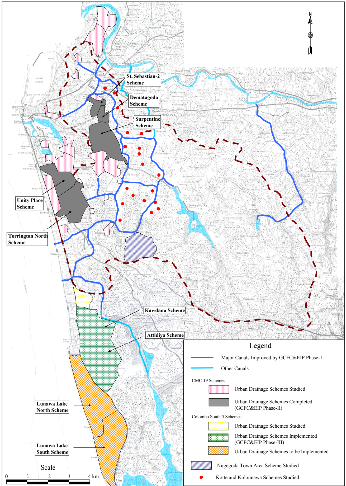
Figure 2.13 Existing and Planned Storm Water Drainage Schemes in Greater Colombo
