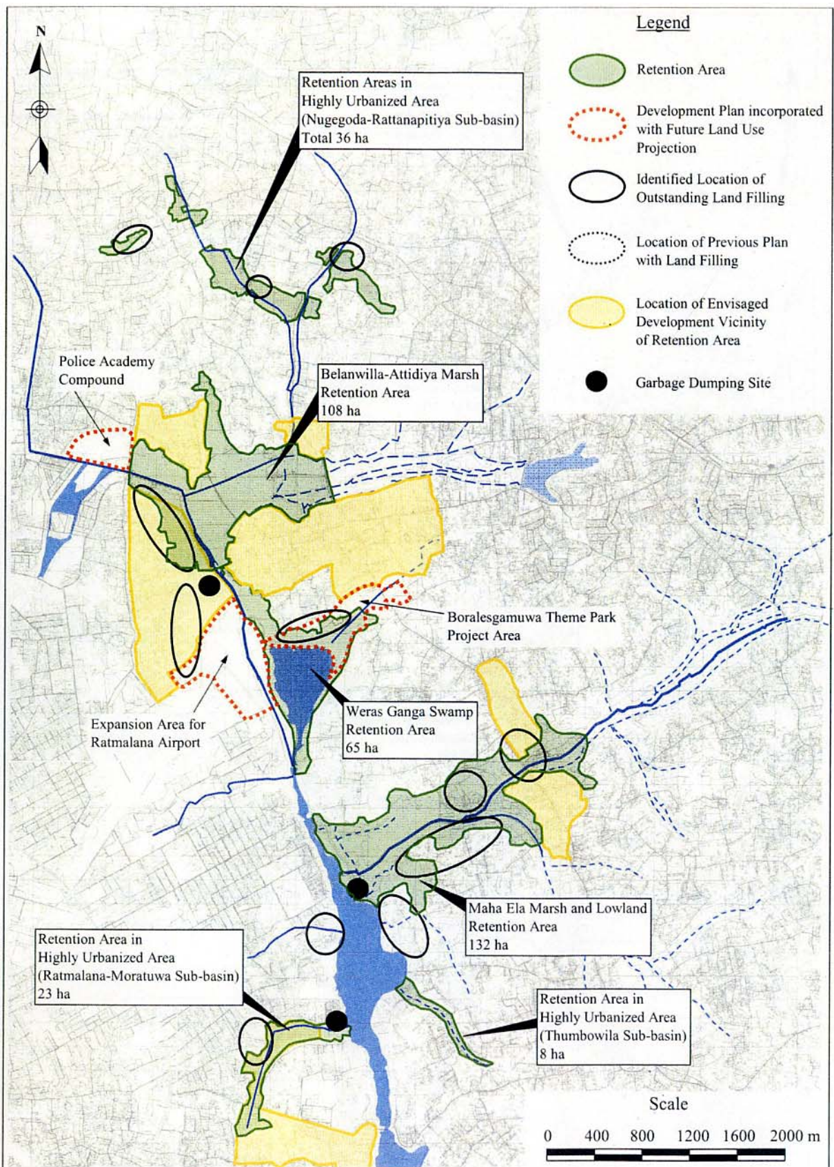
Figure 4.10 Retention Areas under Future Land Use Projection
