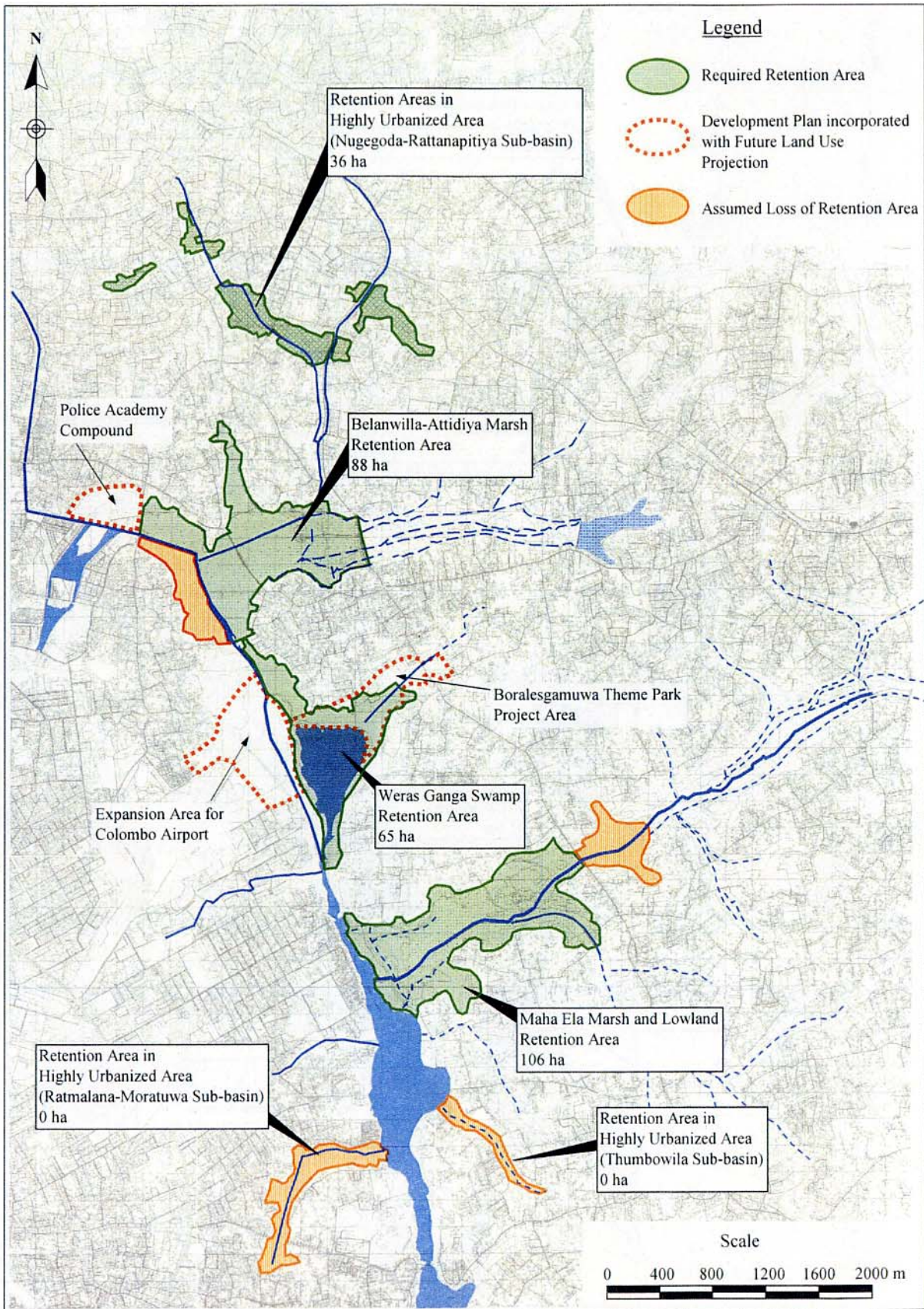
Figure 4.11 Required Retention Area
