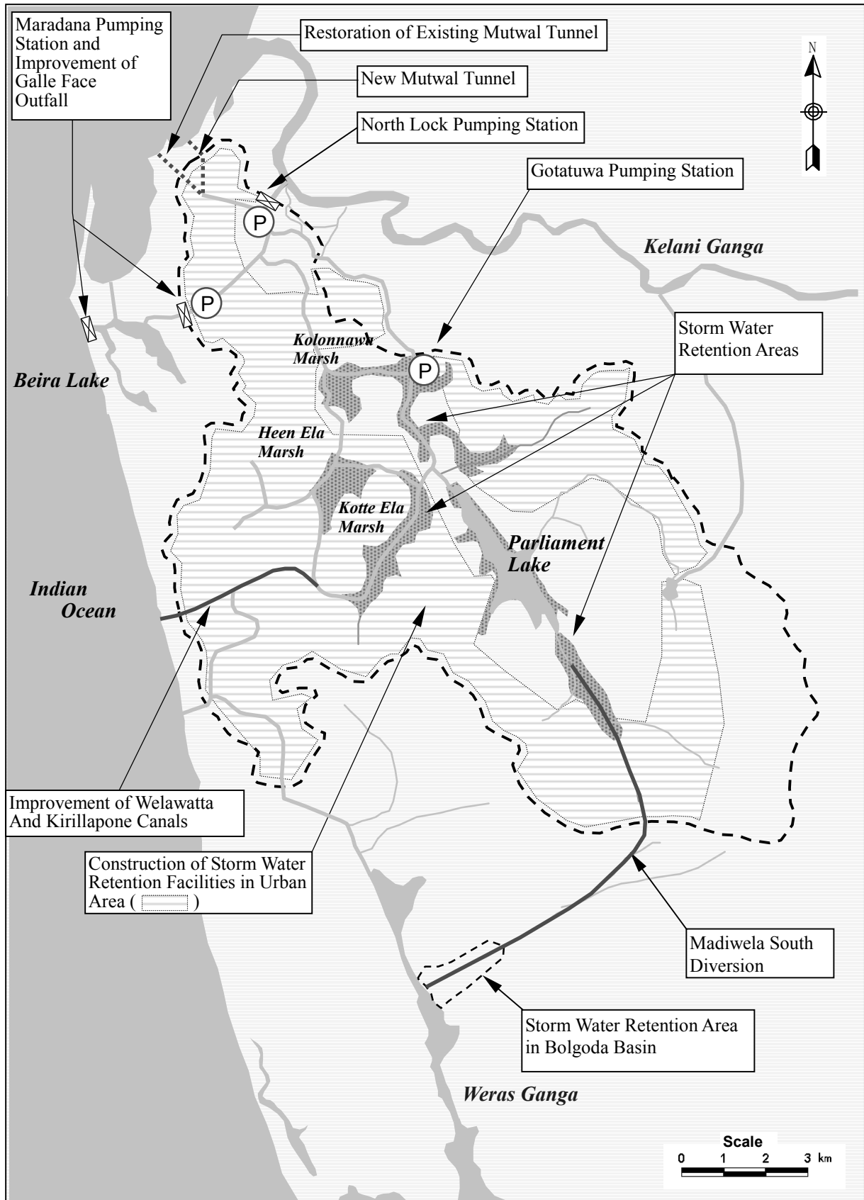
Figure 4.6 Conceivable Structural Measures for Greater Colombo Basin
