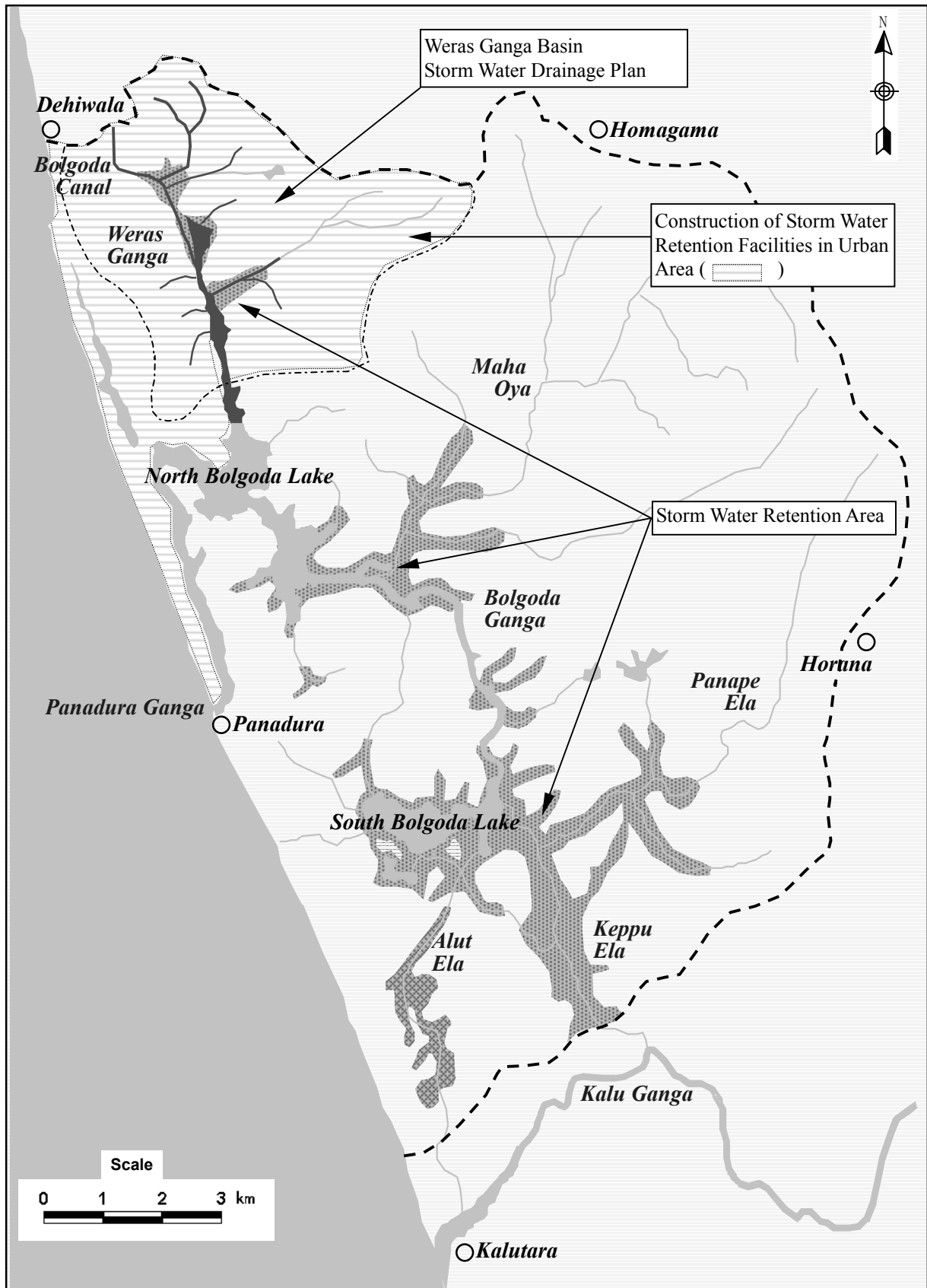
Figure 4.8 Conceivable Structural Measures for Bolgoda Basin
