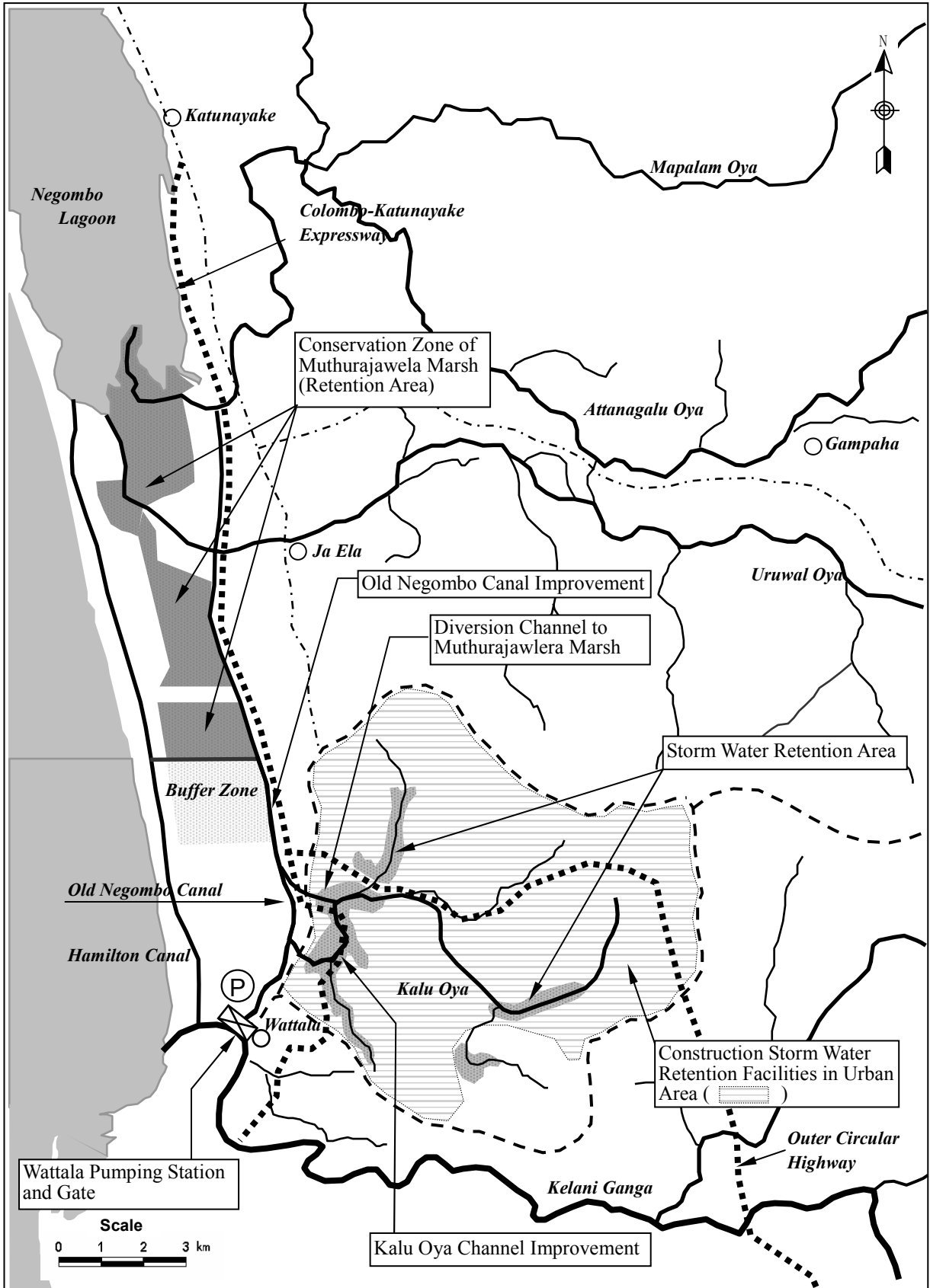
Figure 4.4 Conceivable Structural Measures for Kalu Oya Basin
