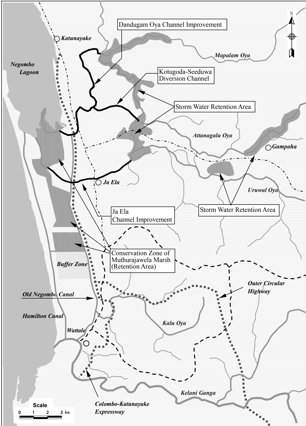
Figure 4.2 Conceivable Structural Measures for Ja Ela Basin
