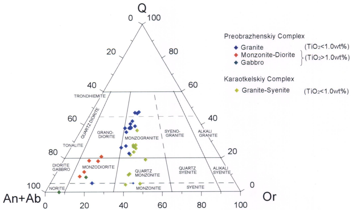
Fig.II-2-10 An+Ab-Or-Q Diagram
