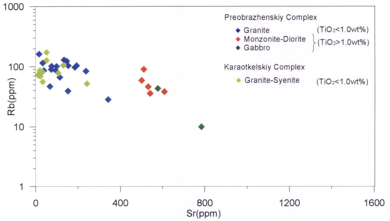
Fig.II-2-15 Rb-Sr diagram
