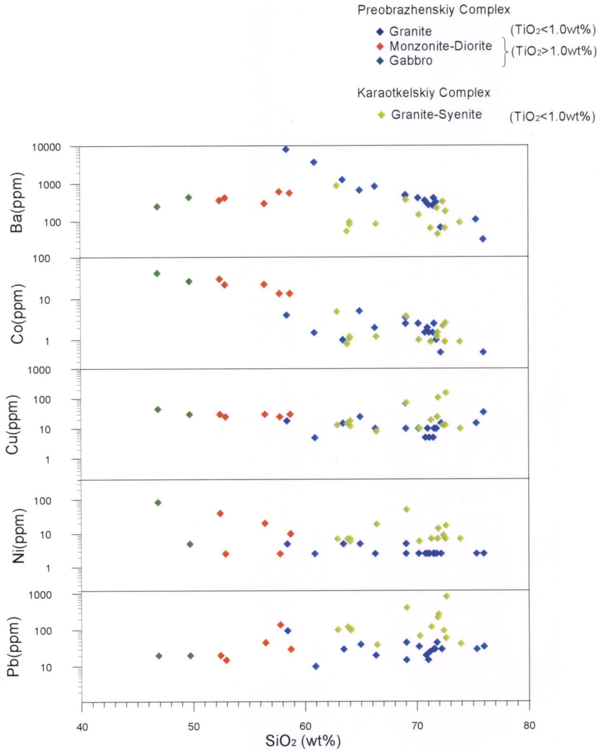
Fig.II-2-11 Minor Element-SiO 2 Variation Diagram
