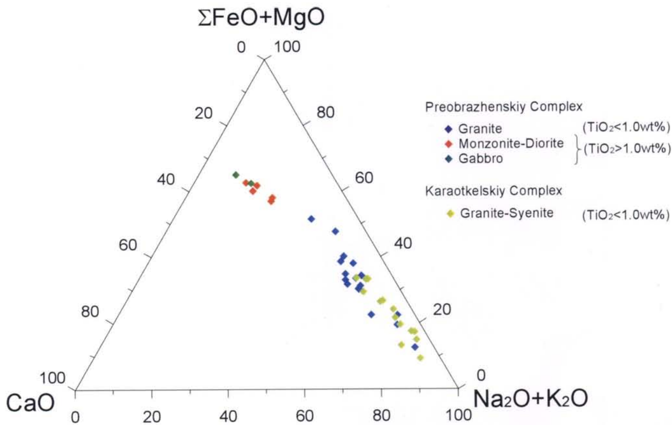
Fig.II-2-7 AFM( \Sigma FeO+MgO-CaO-Na 2 O+K 2 O) Diagram
