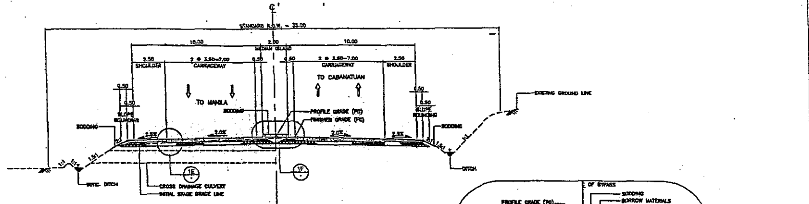
1B NORMAL SECTION - ULTIMATE STAGE SCALE 1:100
