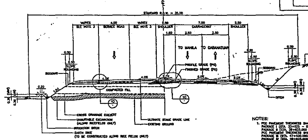
1B NORMAL SECTION - ULTIMATE STAGE SCALE 1:100
