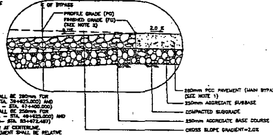
1C DETAIL SCALE 1:20
