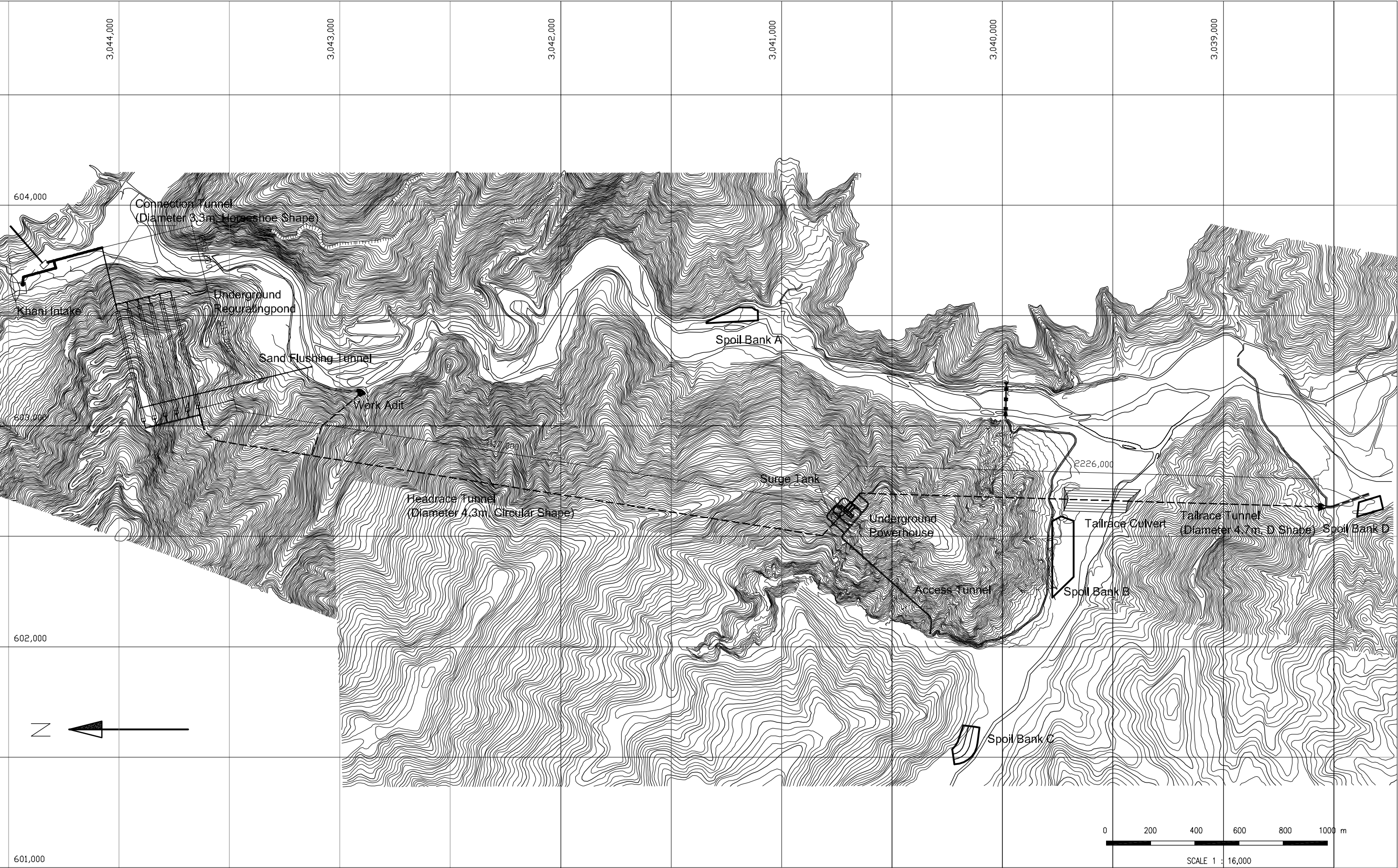
Figure 6.3.5 Plan of Underground Type Regulating Pond ( Alternative B )
