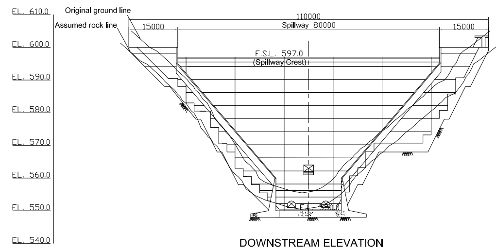
Figure 6.3.4 Details of Dam Type Regulating Pond (Alternative-A)
