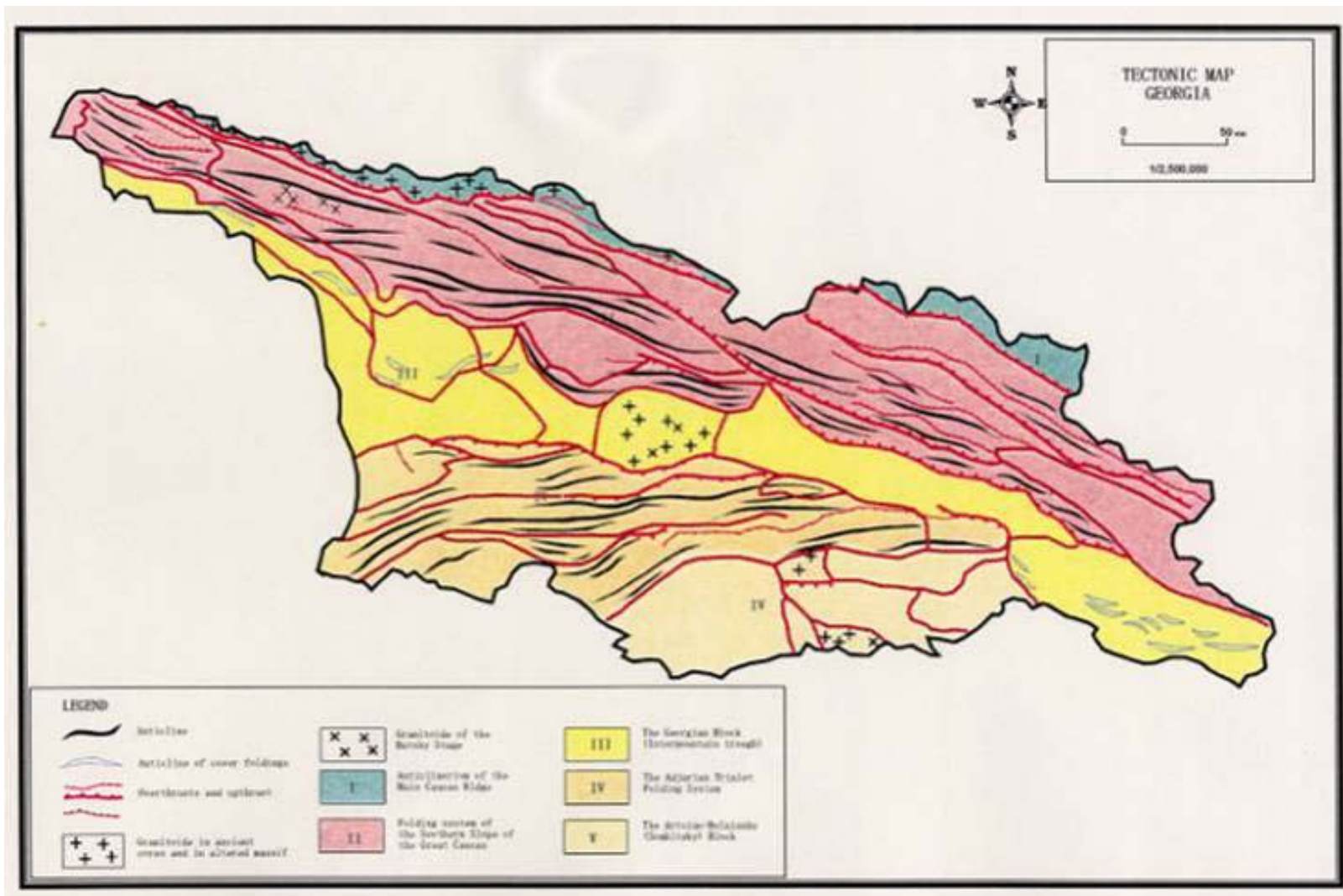
4. Tectonic Map
