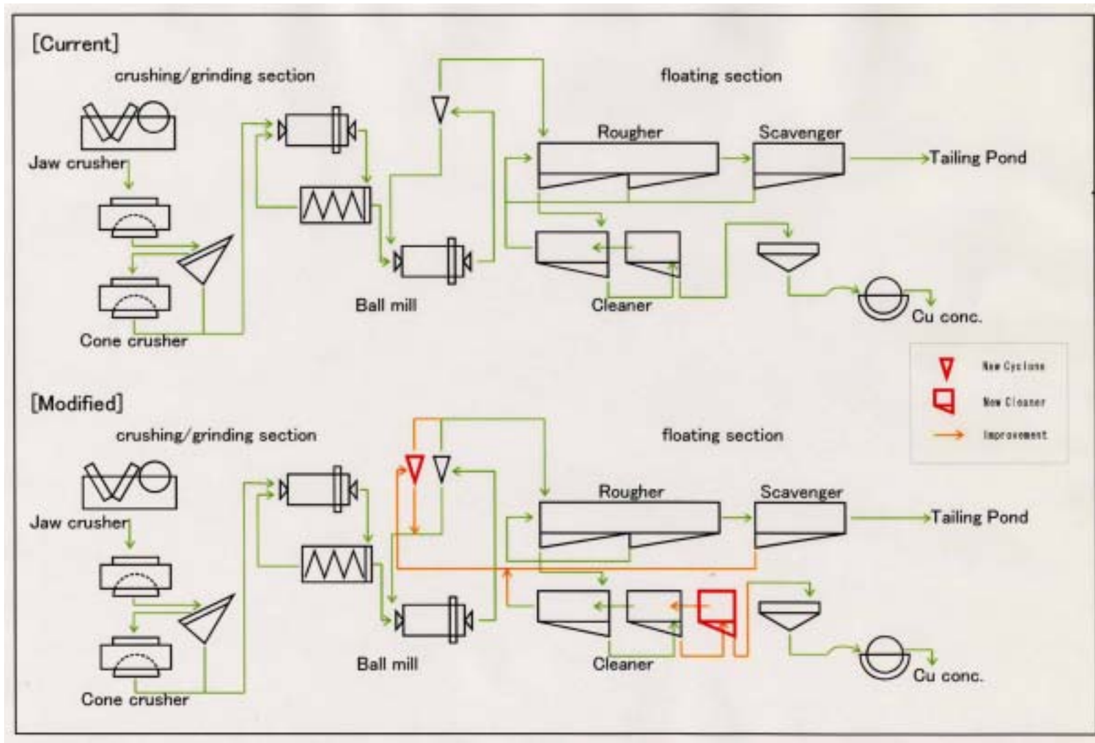
1 2 . Flow of Processing Facility System Improvement
