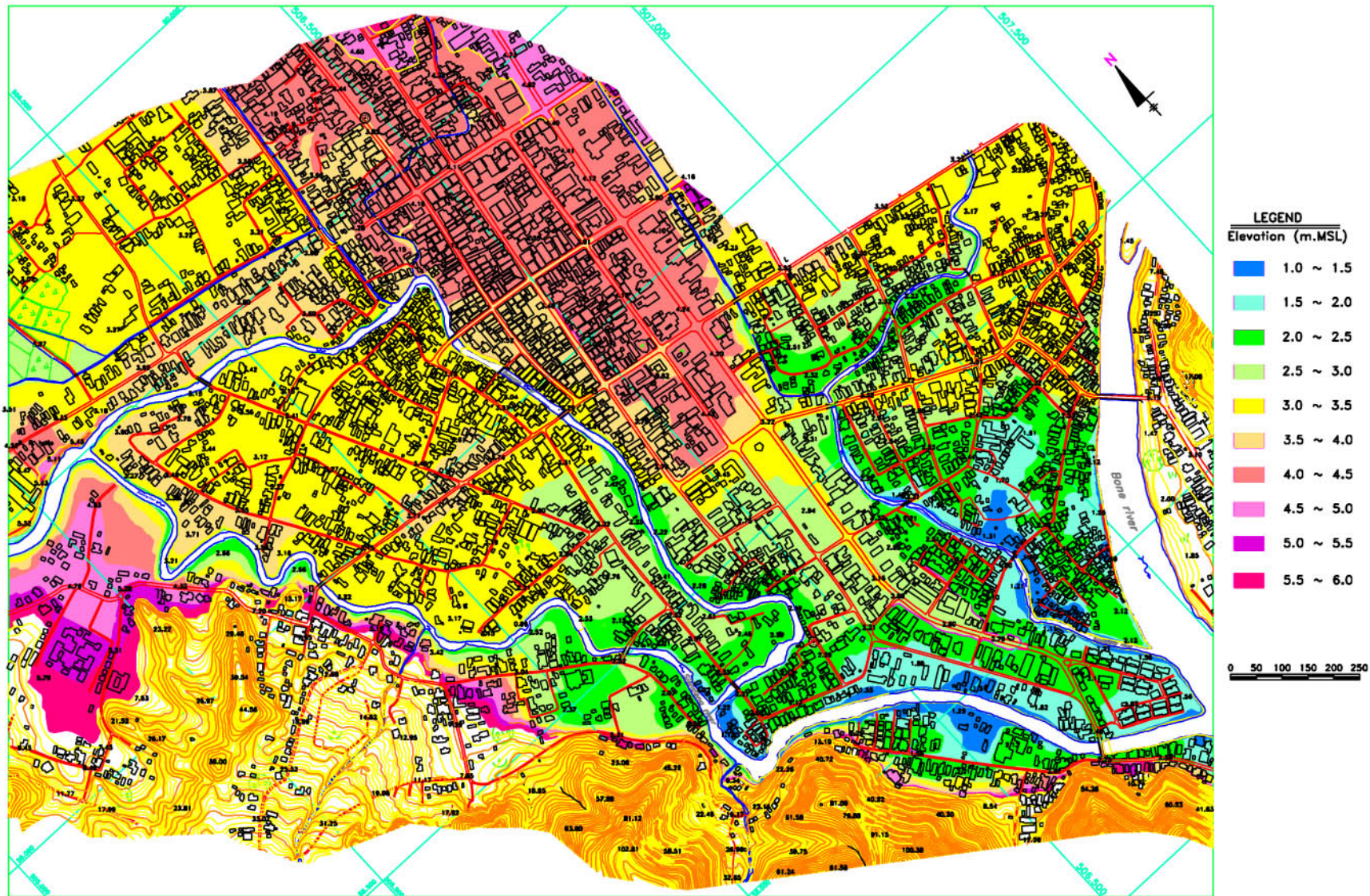
Figure C2.3.2 CONTOUR MAP OF FLOOD PRONE AREA IN GORONTALO CITY
