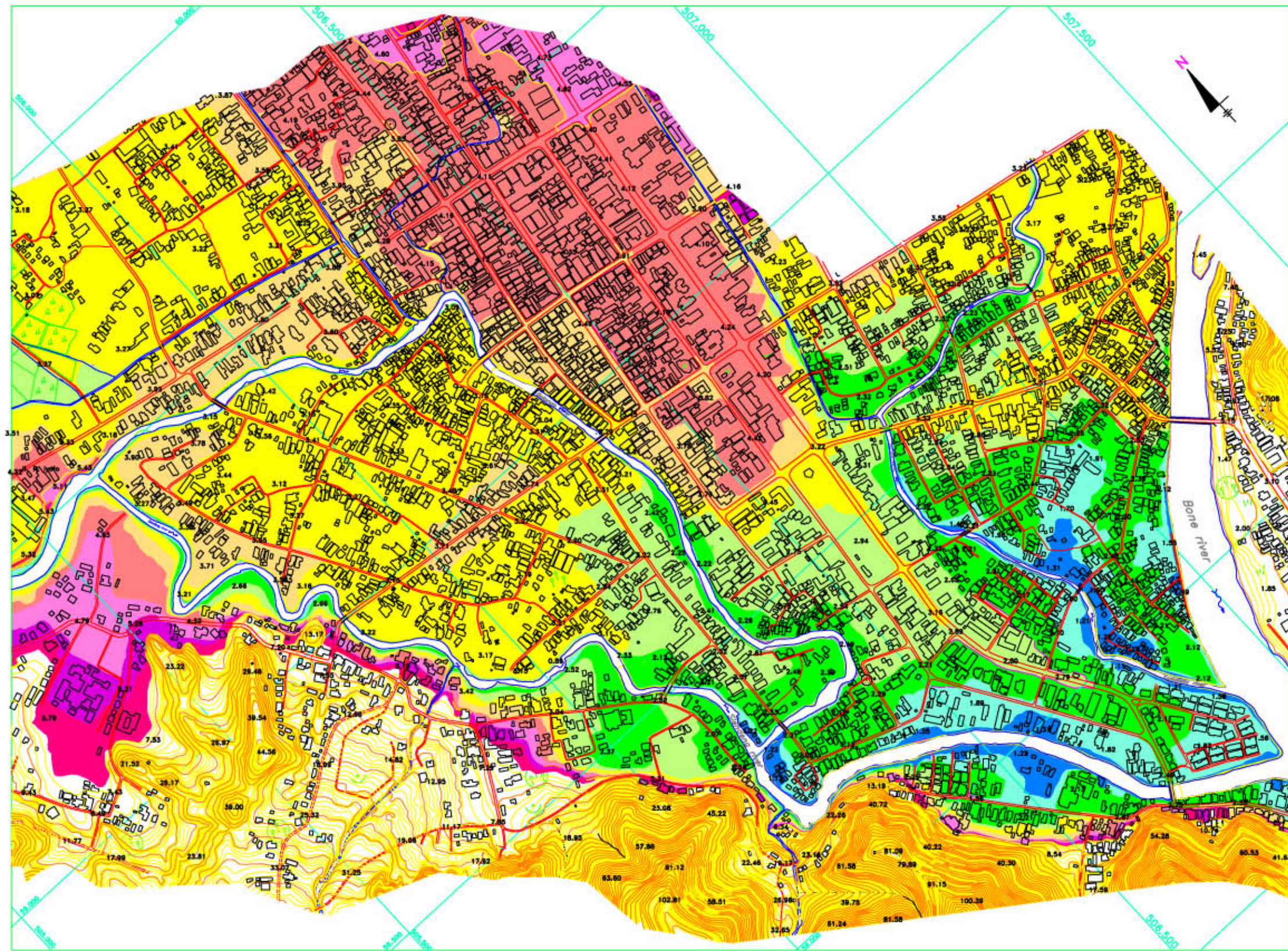
Figure 5.2.4 CONTOUR MAP OF FLOOD PRONE AREA IN GORONTALO CITY
