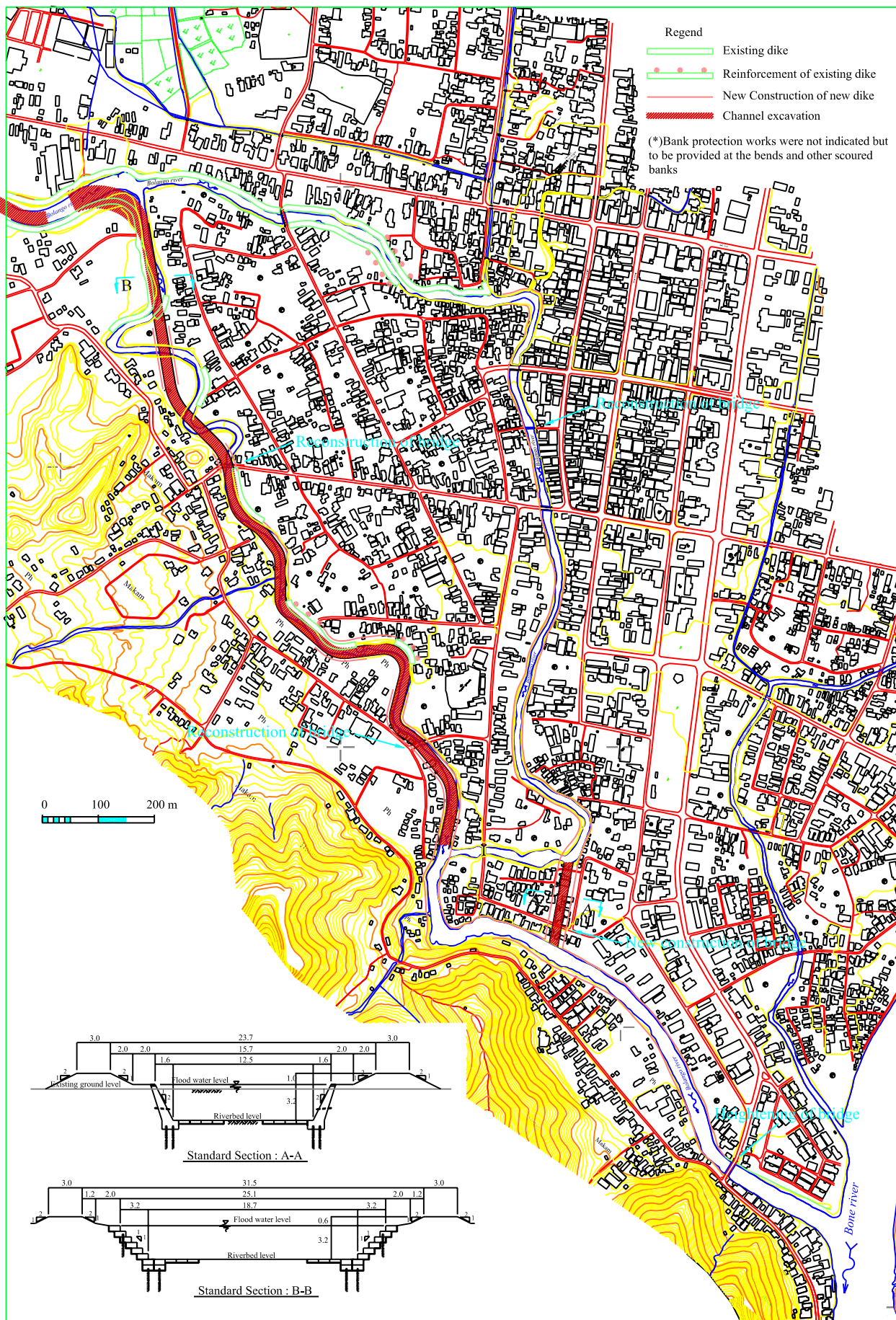
Figure 5.5 BBT RIVER IMPROVEMENT (1/2)
