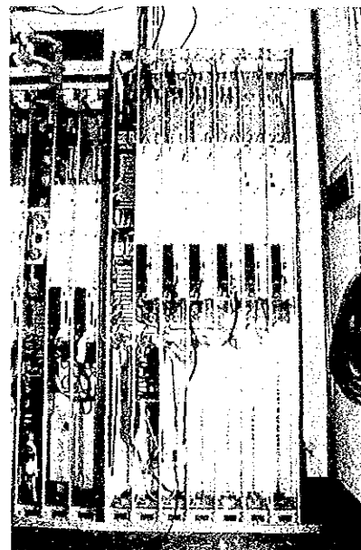
2-8 2Ghz/34Mbps, 7Ghz/16Mbps Microwave, 2.4Ghz Rural Subscriber Communications Relay System installed in P.Xnnoi Relay site
