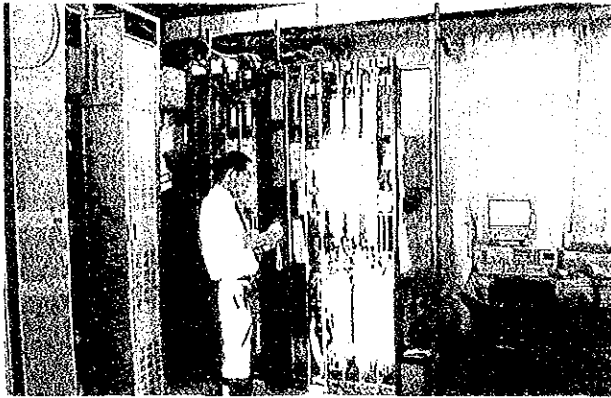
2-1 2Ghz/34Mbps Backbone Microwave System installed in Luangprabang telephone office
