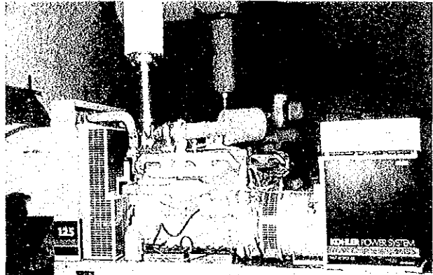
2-6 125KVA Diesel Engine Generator Fujitsu(Kohler power system) ,JICA installed in Luangprabang telephone office
