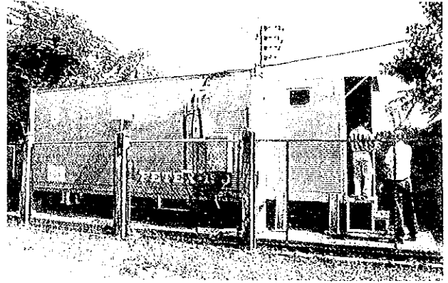
3-3 Transportable Switching System Fujitsu Ftex-150 installed in Vientiane area
