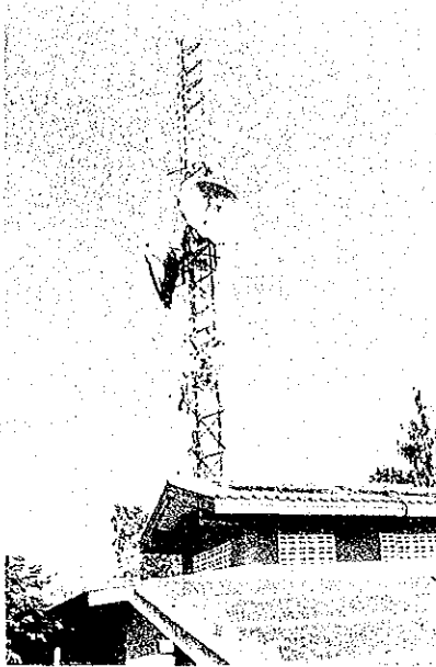
2-9 Microwave parabolic antenna and tower installed in P.Xnunoi Relay site
