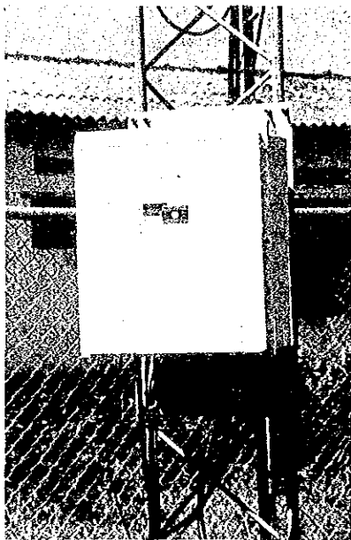
2-23 2.4Ghz Rural Subscriber Communications Terminal System, Alcatel Rutel, Germany installed located at Mounghoum in Xiengkhuang Province
