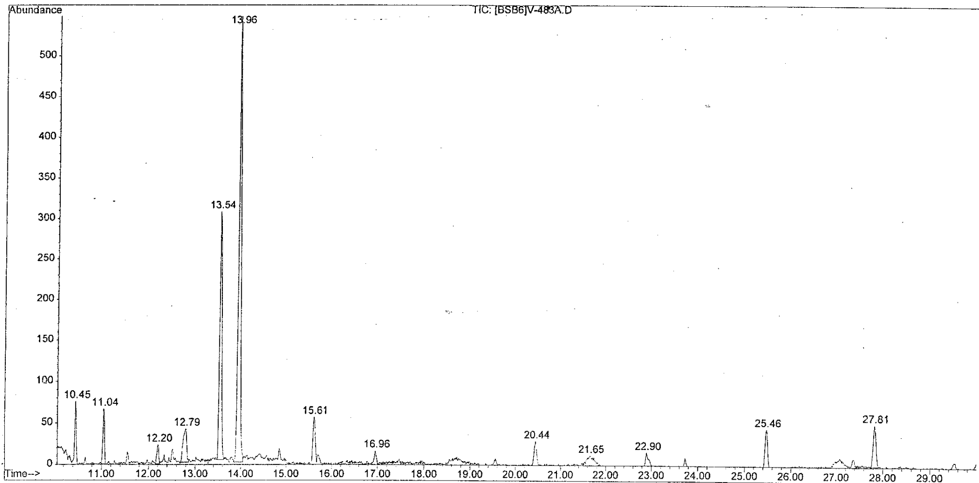
Figure G6. 8 Dioxin Analysis
