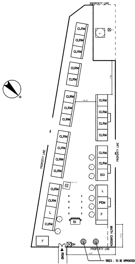
EXISTING SITE PLAN SCALE 1:1500M
