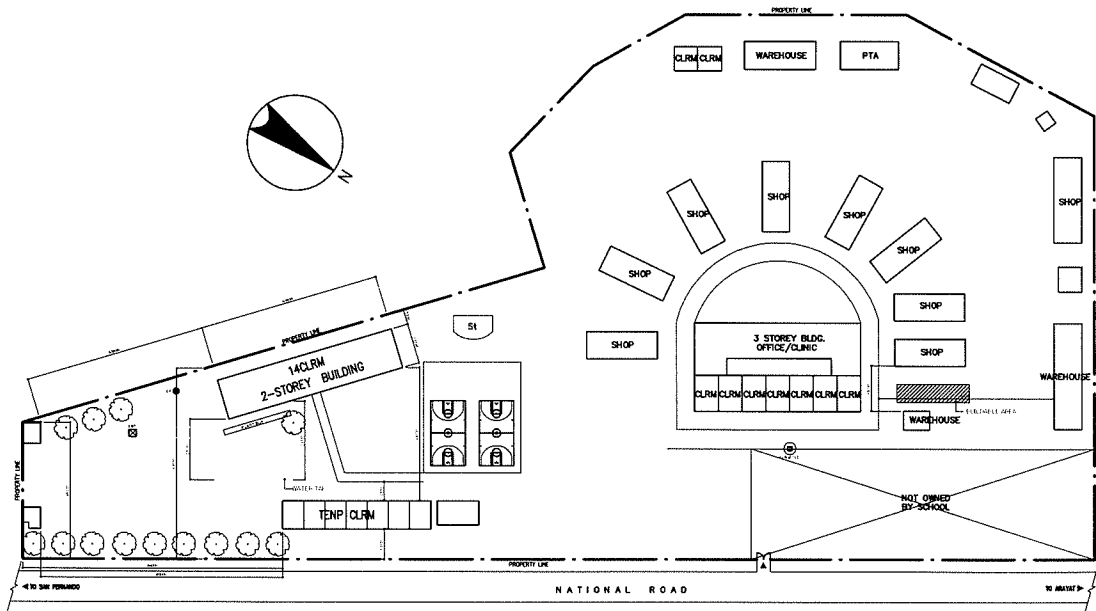
EXISTING SITE PLAN SCALE 1:2500M
