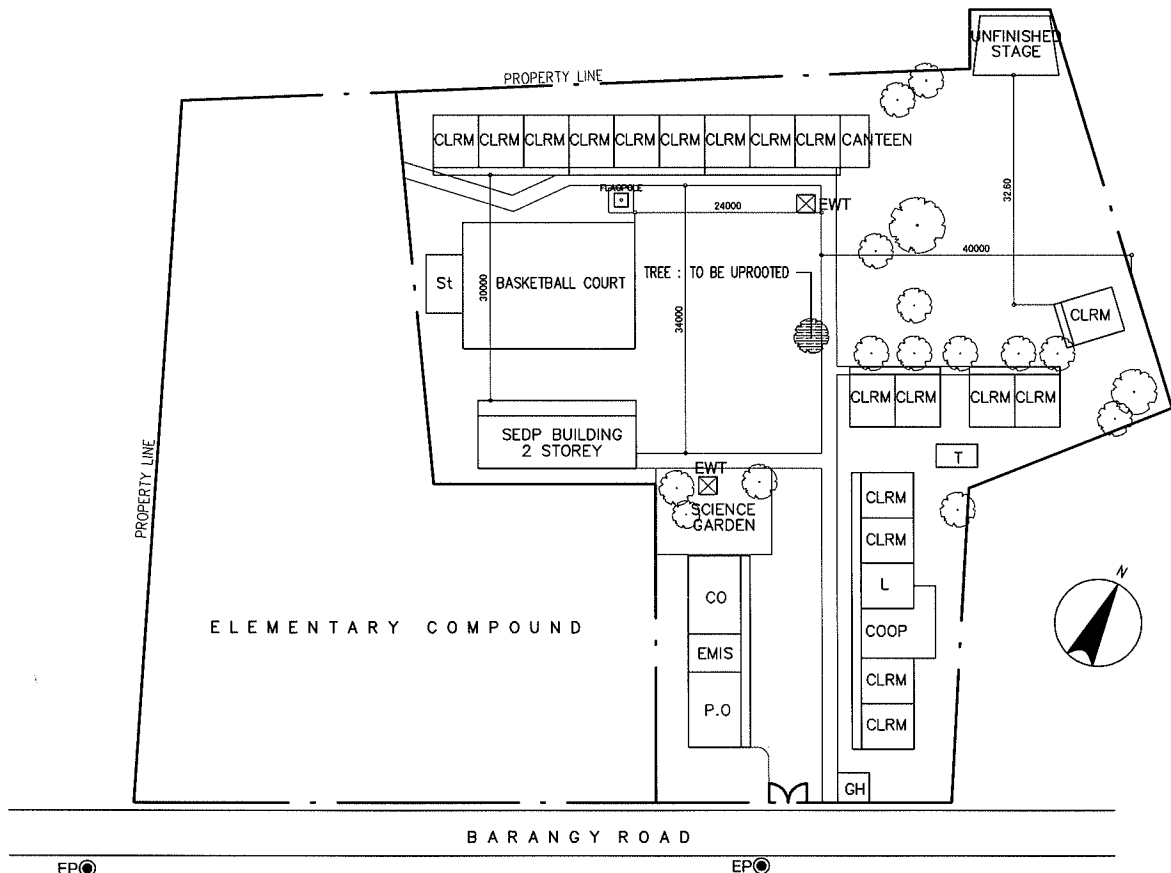
EXISTING SITE PLAN SCALE 1:1000M
