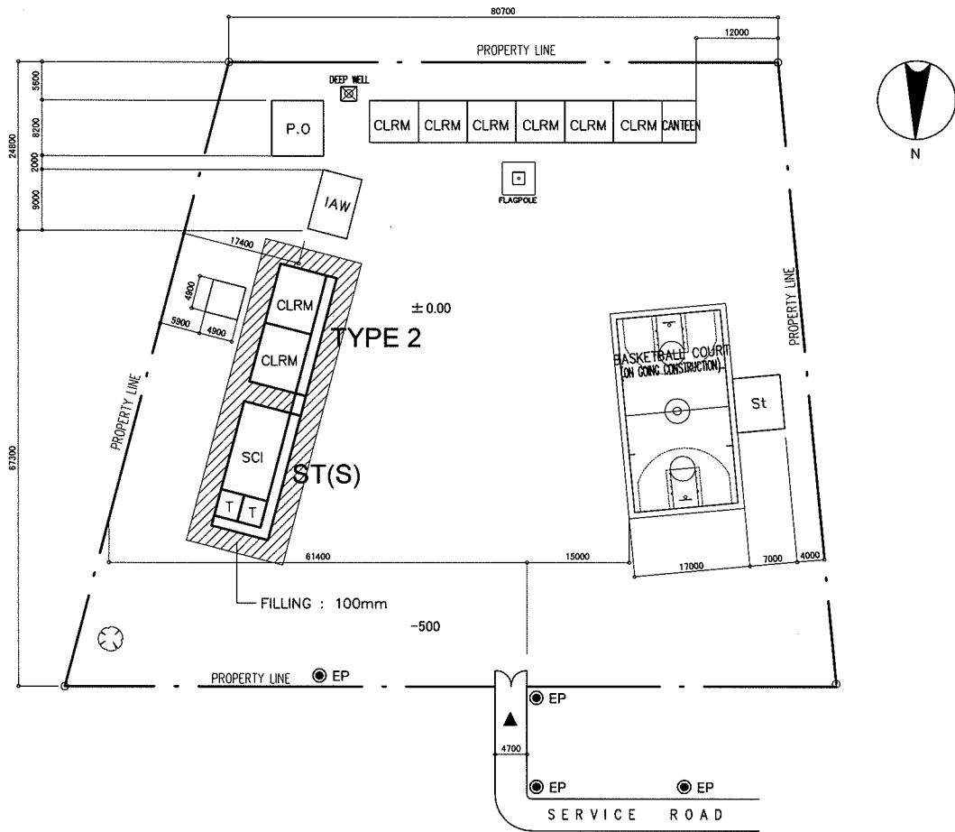
PROPOSED SITE PLAN SCALE 1:1000M
