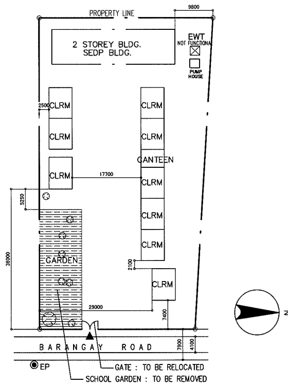
EXISTING SITE PLAN SCALE 1:1000M
