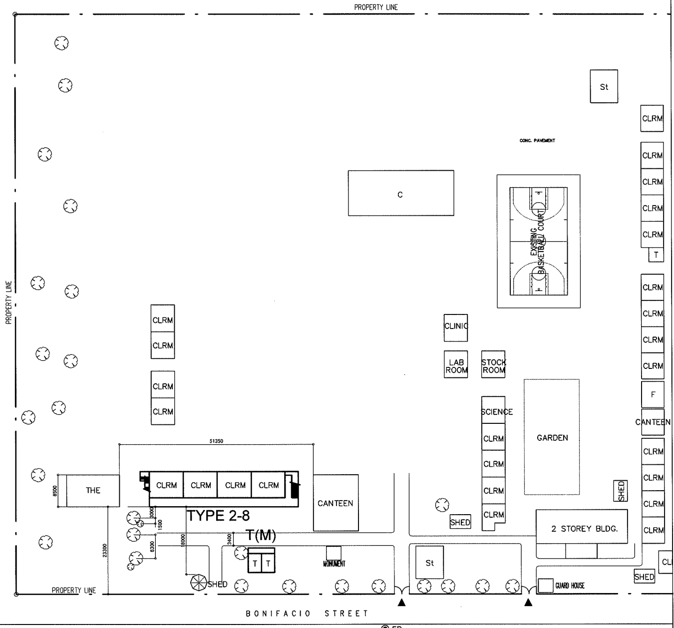
PROPOSED SITE PLAN SCALE 1:1000M
