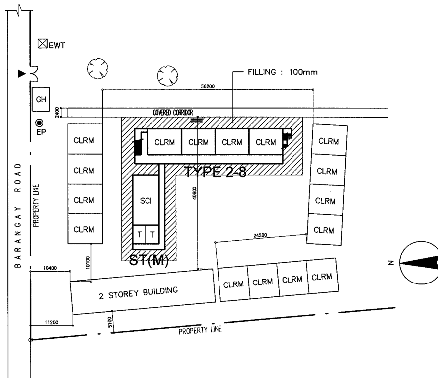
PROPOSED SITE PLAN SCALE 1:1000M
