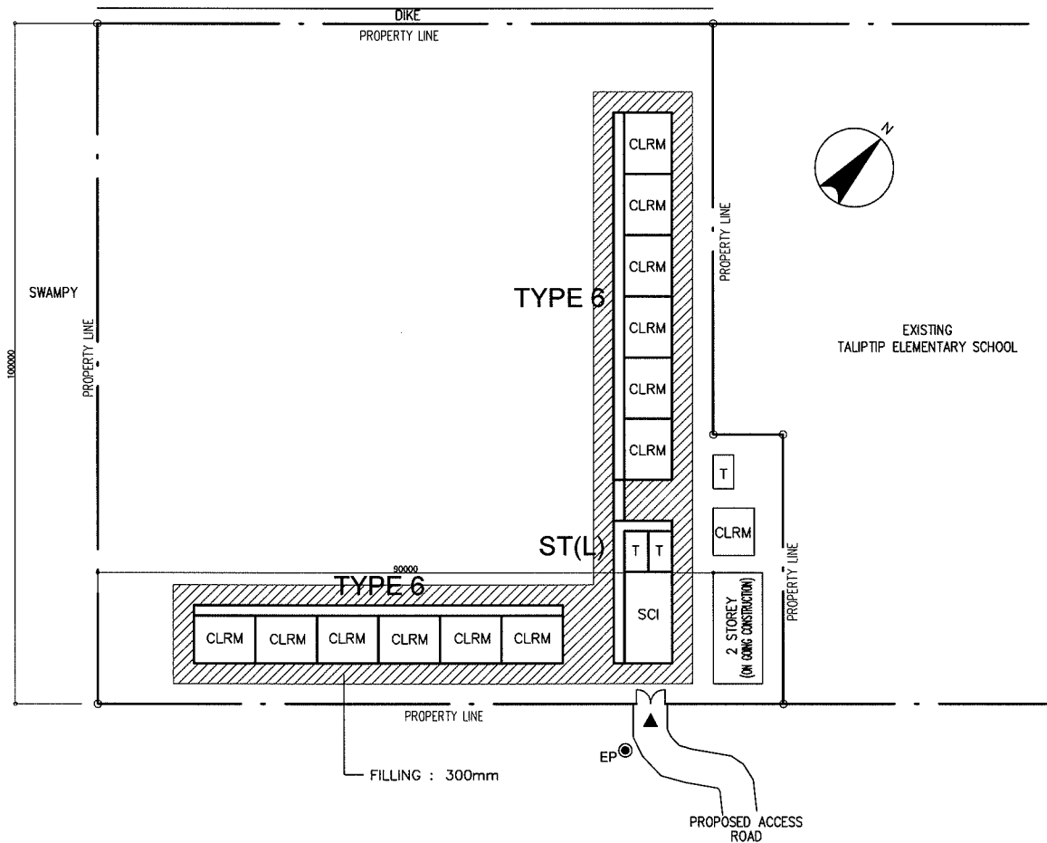
PROPOSED SITE PLAN SCALE 1:1000M
