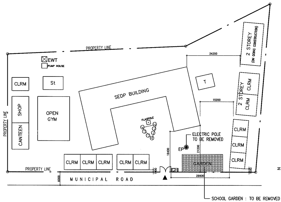
EXISTING SITE PLAN SCALE 1:1000M
