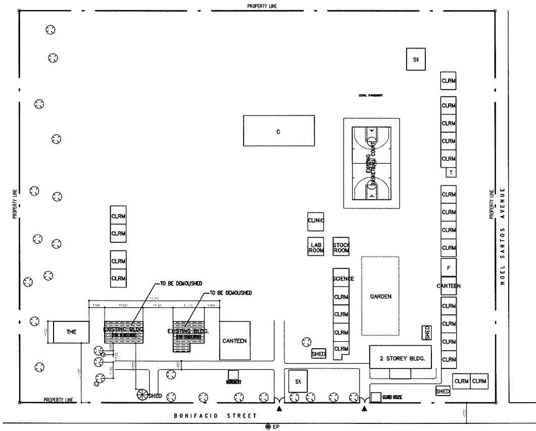
EXISTING SITE PLAN SCALE 1:1500M
