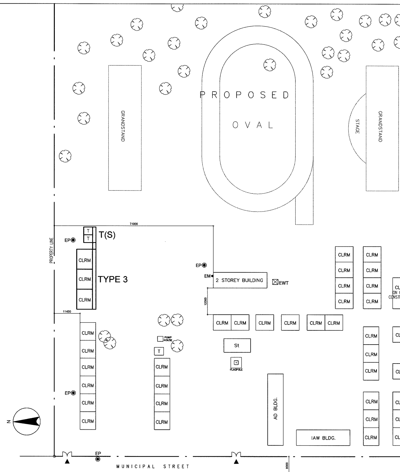
PROPOSED SITE PLAN SCALE 1:1000M
