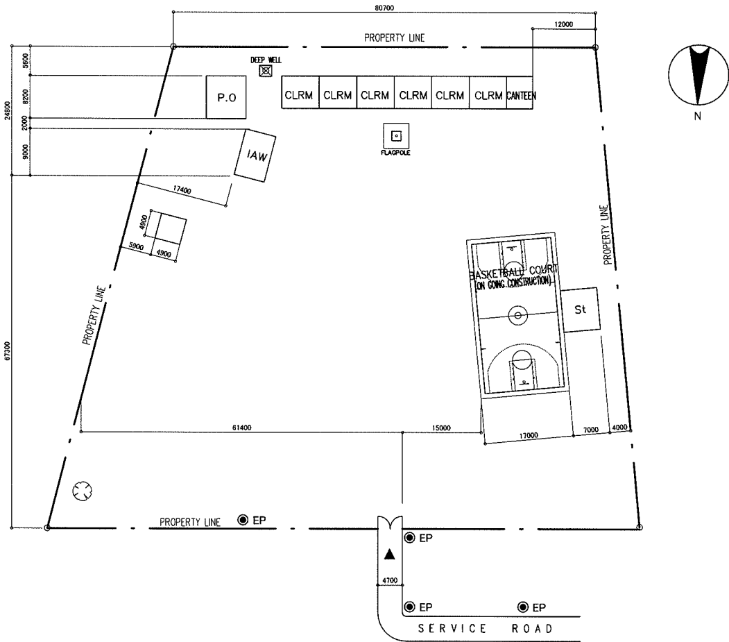
EXISTING SITE PLAN SCALE 1:1000M
