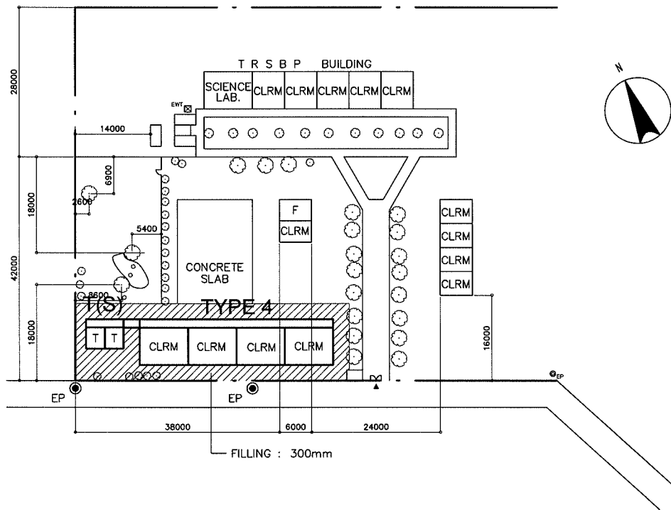
PROPOSED SITE PLAN SCALE 1:1000M
