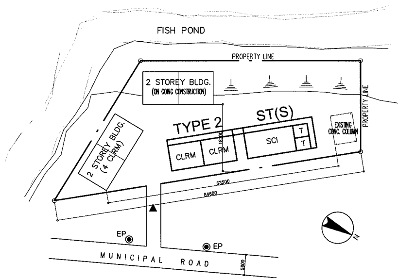
PROPOSED SITE PLAN SCALE 1:1000M
