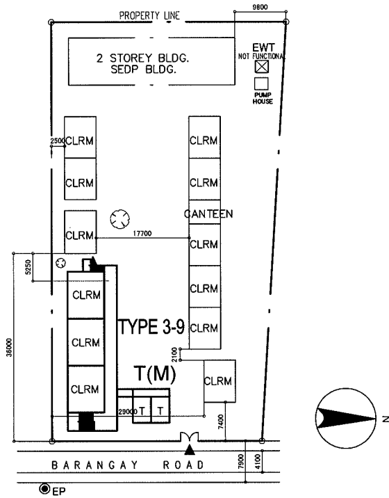
PROPOSED SITE PLAN SCALE 1:1000M
