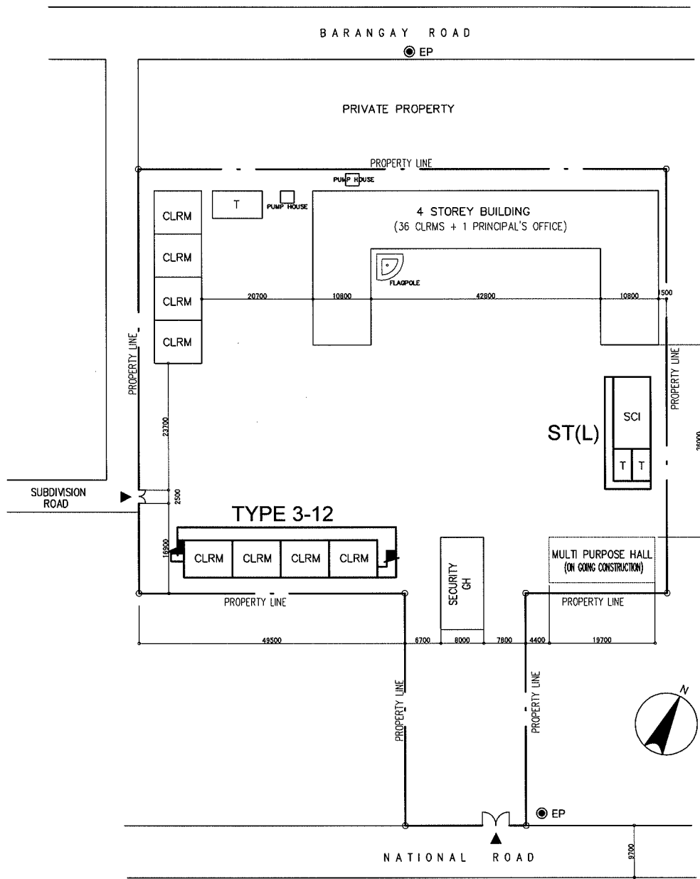
PROPOSED SITE PLAN SCALE 1:1000M
