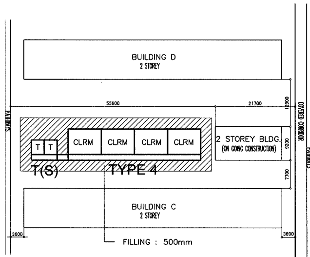
PROPOSED SITE PLAN SCALE 1:1000M
