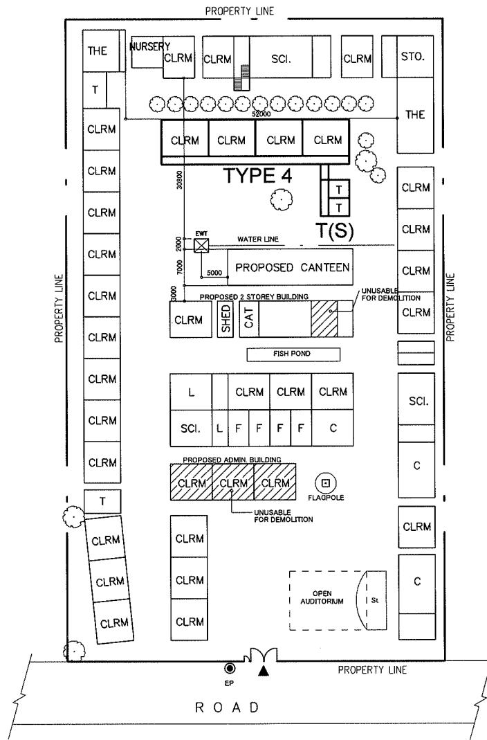
PROPOSED SITE PLAN SCALE 1:1000M
