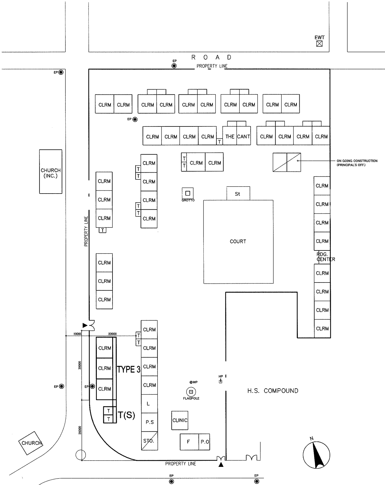
PROPOSED SITE PLAN SCALE 1:1000M
