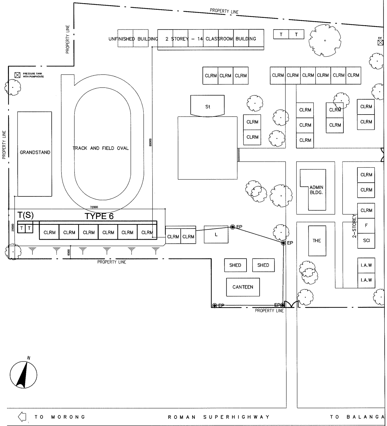
PROPOSED SITE PLAN SCALE 1:1000M
