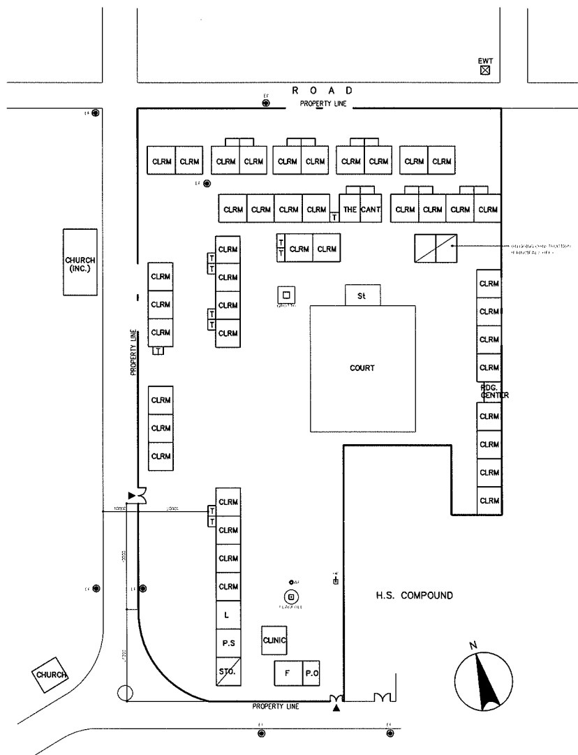
EXISTING SITE PLAN SCALE 1:1500M
