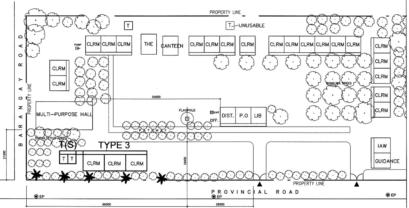
PROPOSED SITE PLAN SCALE 1:1000M
