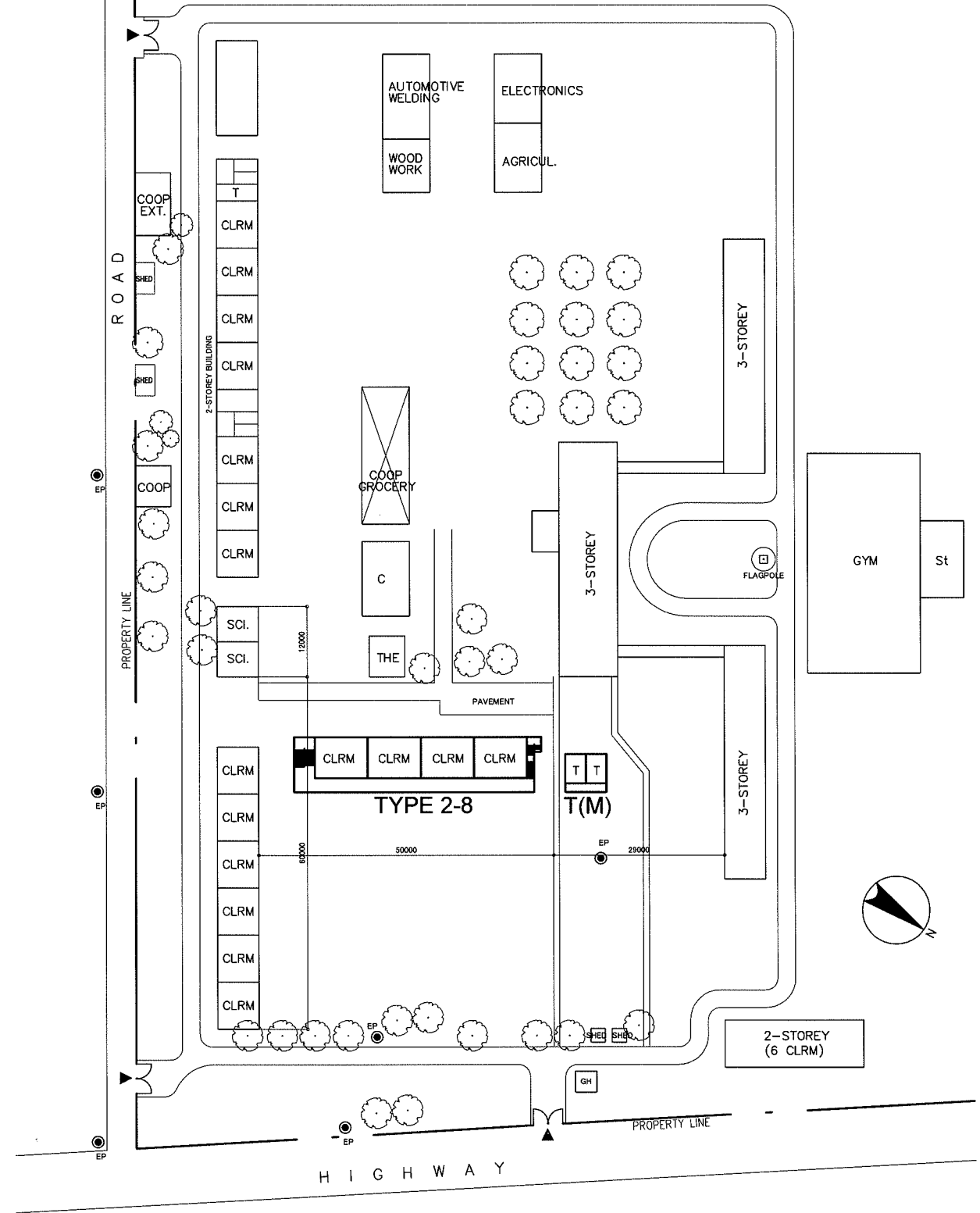
PROPOSED SITE PLAN SCALE 1:1000M
