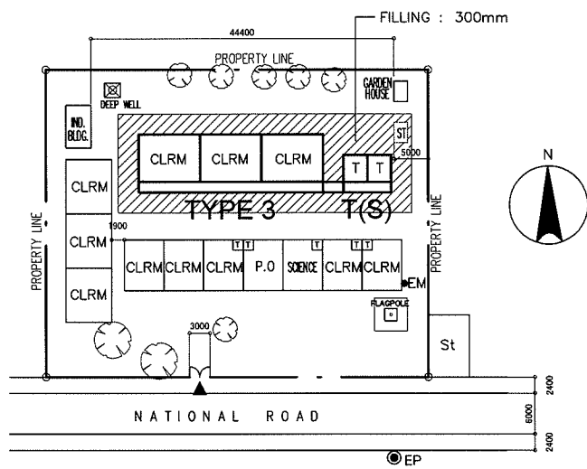
PROPOSED SITE PLAN SCALE 1:1000M
