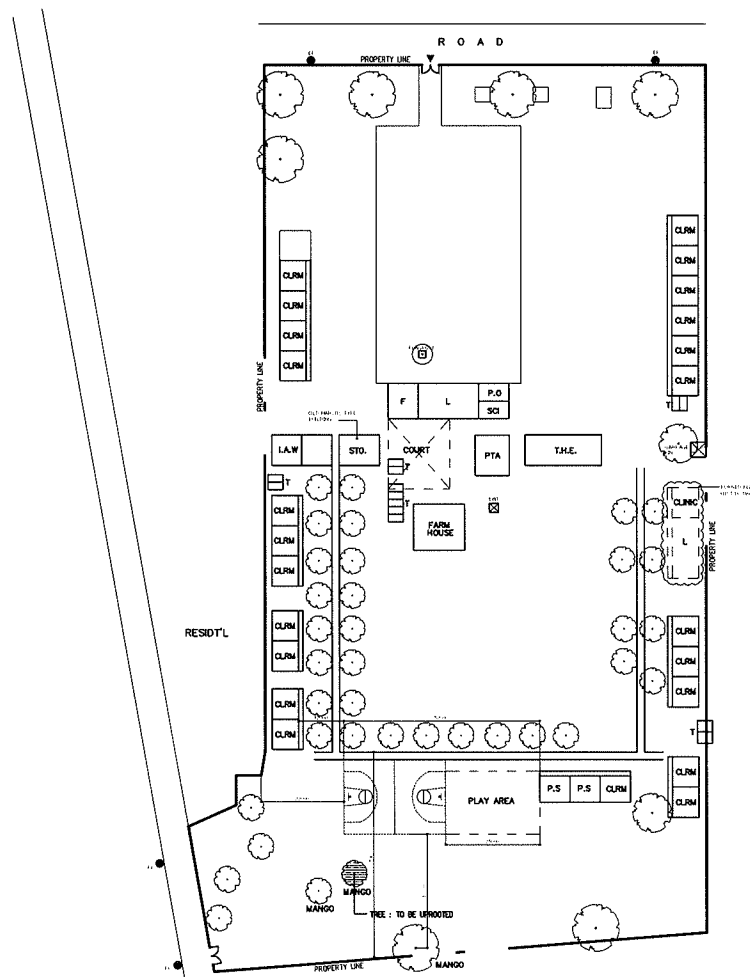
EXISTING SITE PLAN SCALE 1:2000M
