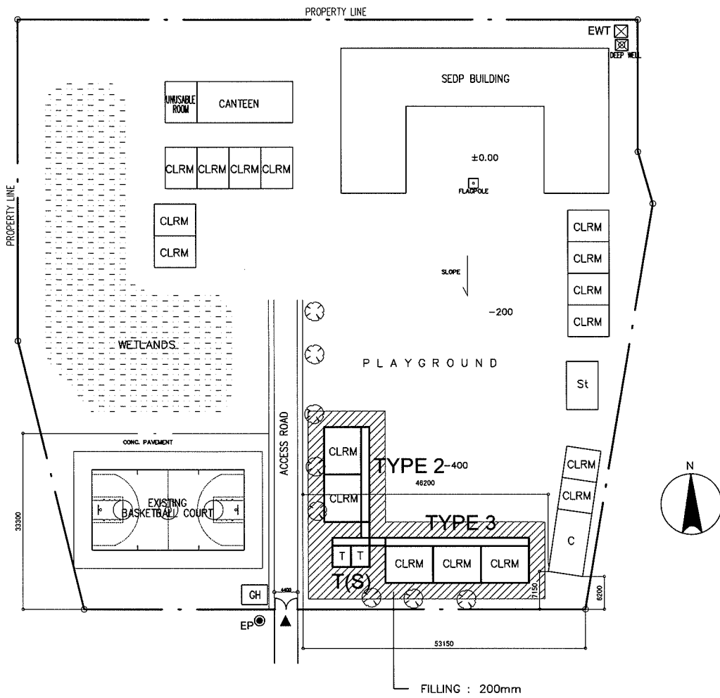
PROPOSED SITE PLAN SCALE 1:1000M
