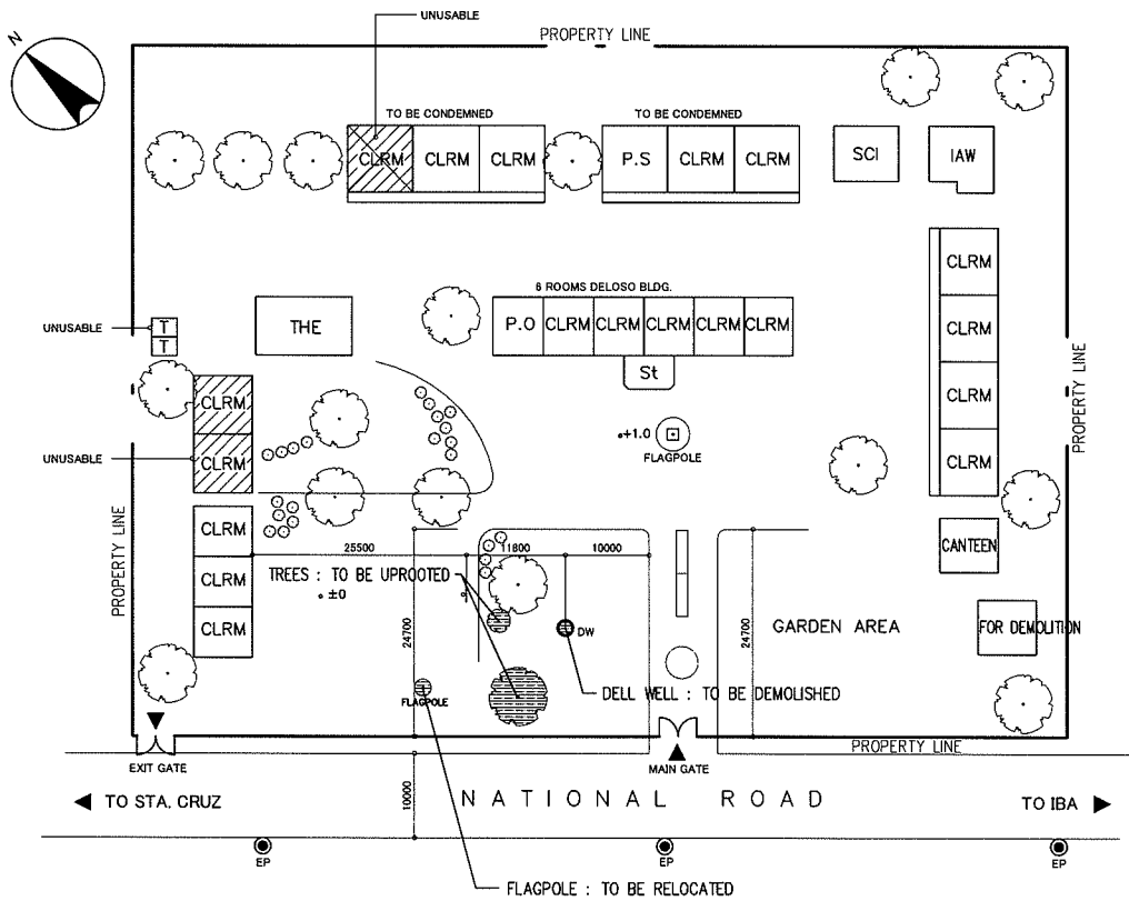
EXISTING SITE PLAN SCALE _____ 1:1000M
