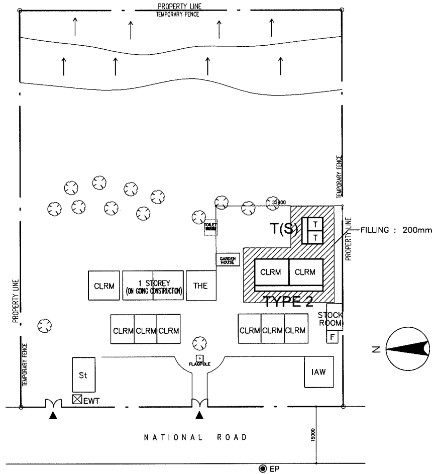
PROPOSED SITE PLAN SCALE 1:1000M
