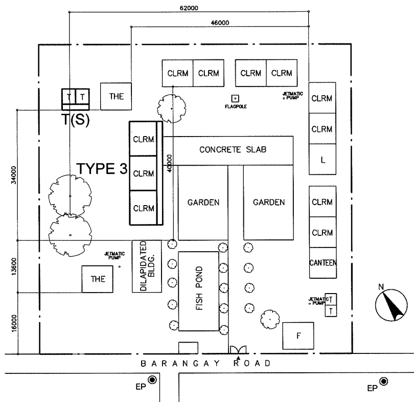
PROPOSED SITE PLAN SCALE 1:1000M
