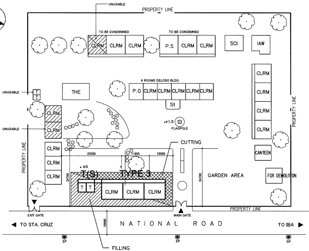
PROPOSED SITE PLAN SCALE 1:1000M
