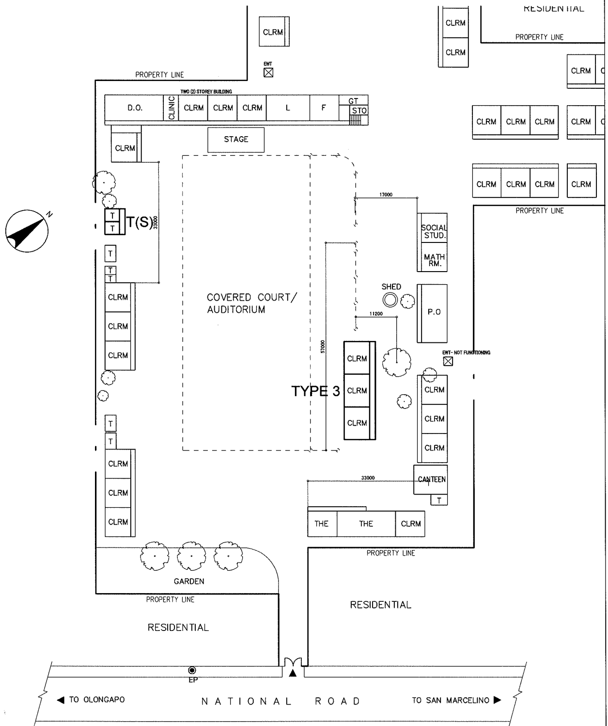
PROPOSED SITE PLAN SCALE 1:1000M
