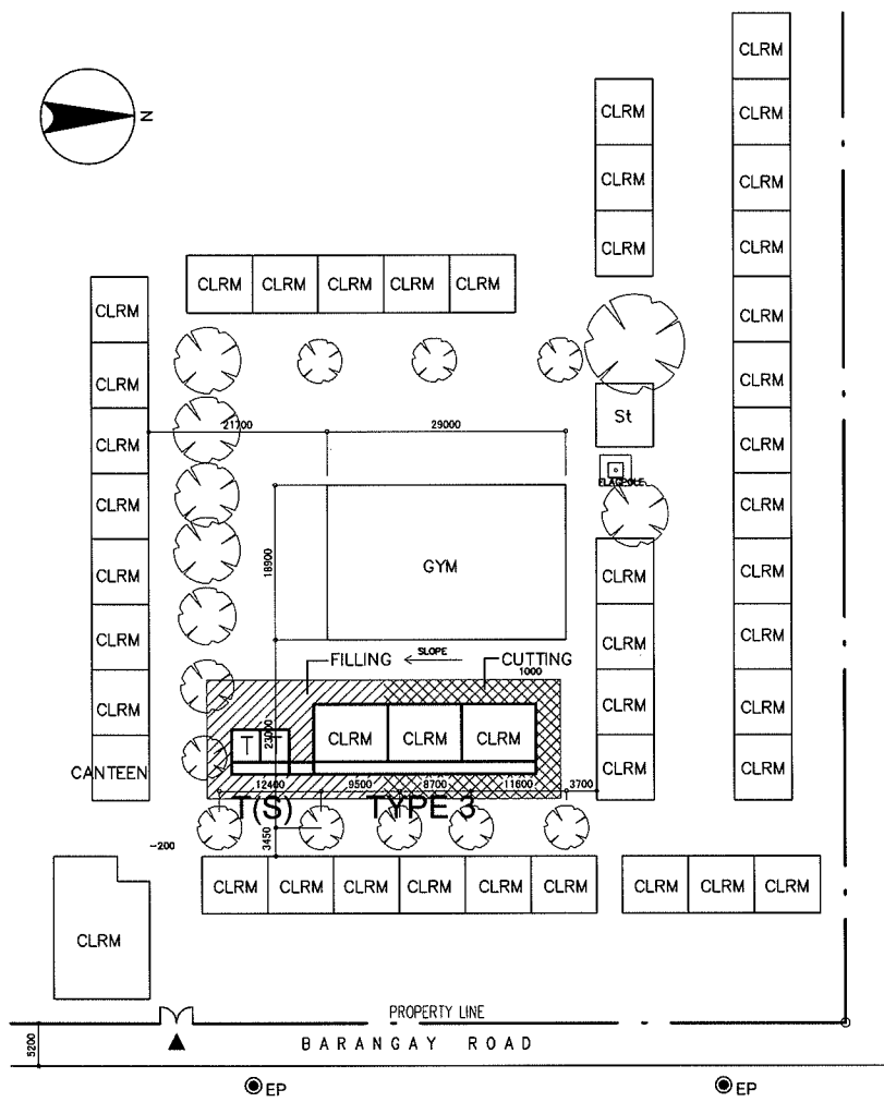
PROPOSED SITE PLAN SCALE 1:1000M
