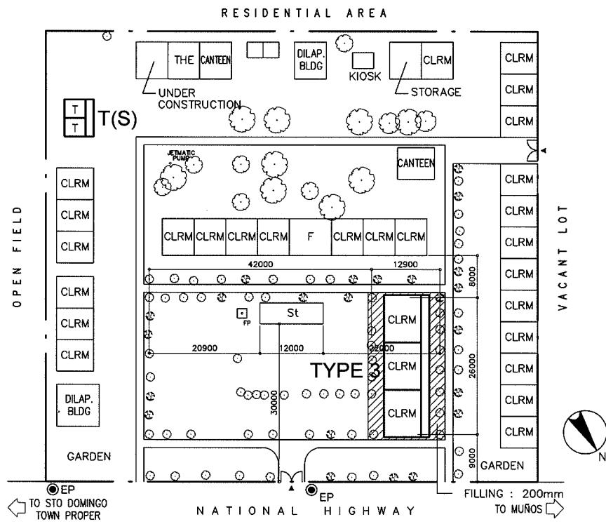
PROPOSED SITE PLAN SCALE 1:1000M
