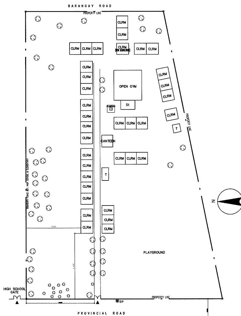
EXISTING SITE PLAN SCALE 1:1500M
